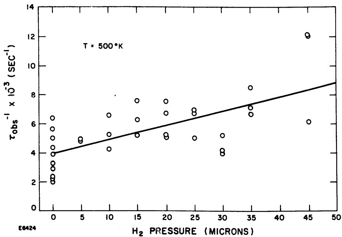
Fig. A-3 Plot of Pseudo First Order Rate Constant \tau_{\text{OBS}}^{-1} vs P_{\text{H}_2} at 500°K for \text{Pb } ^3\text{P}_2 monitored 4058 Å
