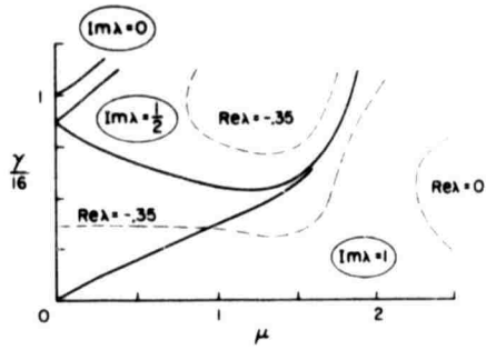
Fig. 13. Lines of constant \text{Im}\lambda and \text{Re}\lambda , based on numerical calculation of the eigenvalues (from Ref. 2); \nu = 1 , K_P = 0 ; ——— \text{Im}\lambda , — — — \text{Re}\lambda ; circled values of \text{Im}\lambda indicate areas in which \text{Im}\lambda is constant.
