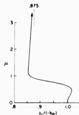
Fig. 10. Motion of the root on the real axis for varying \mu , \gamma = \infty . For large \gamma there are two real roots; \lambda_1 is the finite real root; the other root is at \lambda = -\infty for \gamma = \infty .
