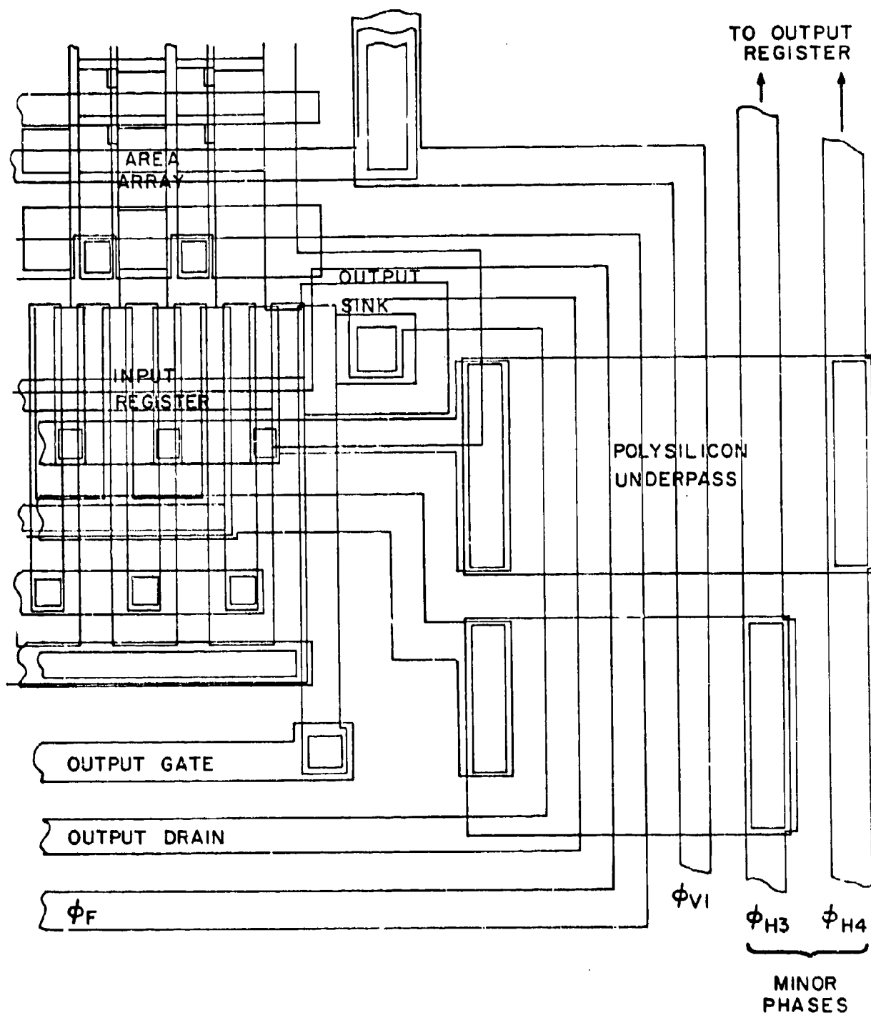
FIGURE 4-36. OUTPUT END OF THE INPUT REGISTER
