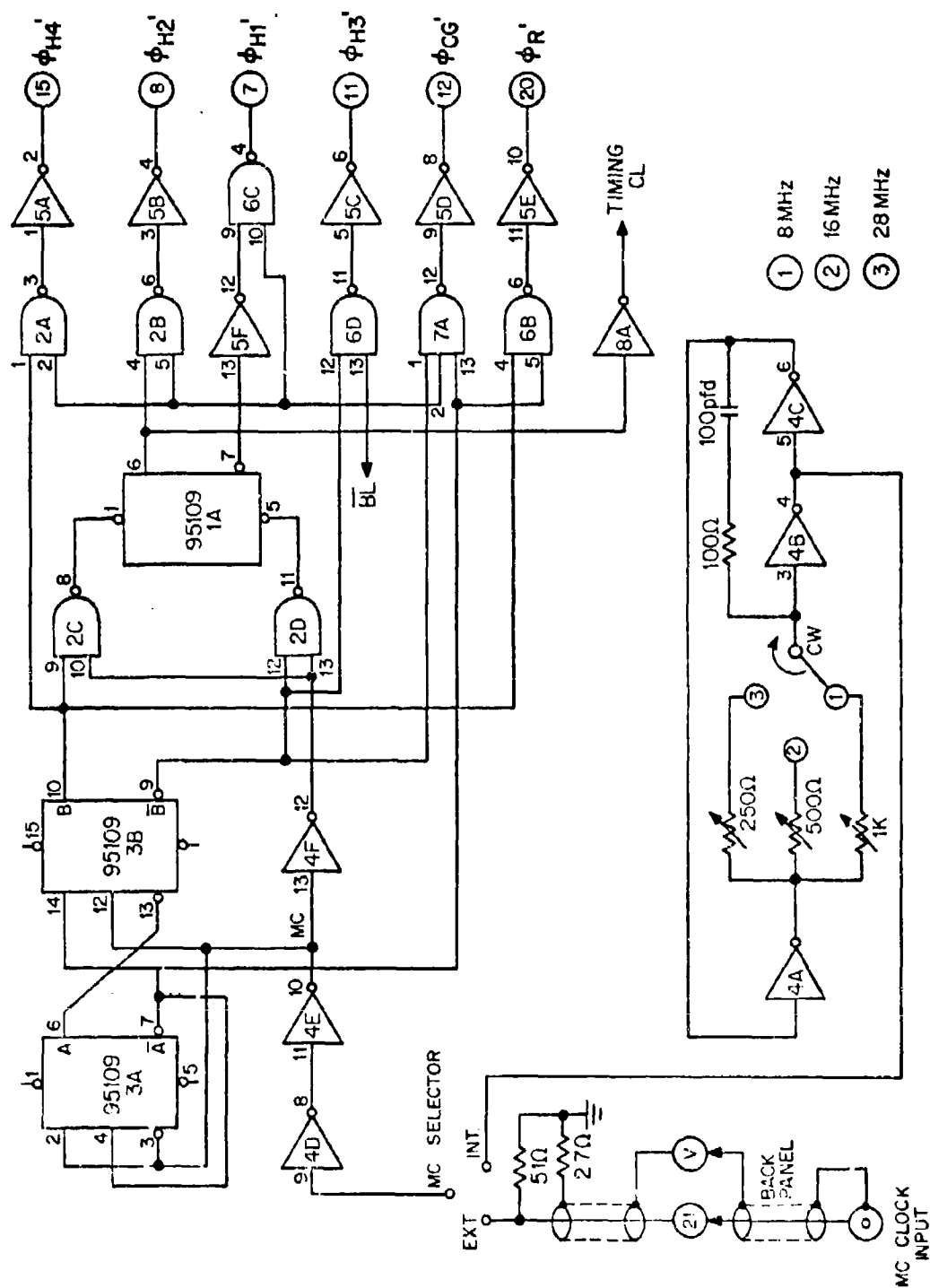
FIGURE 4-52. LOGIC FOR HORIZONTAL REGISTERS AND DFGA
