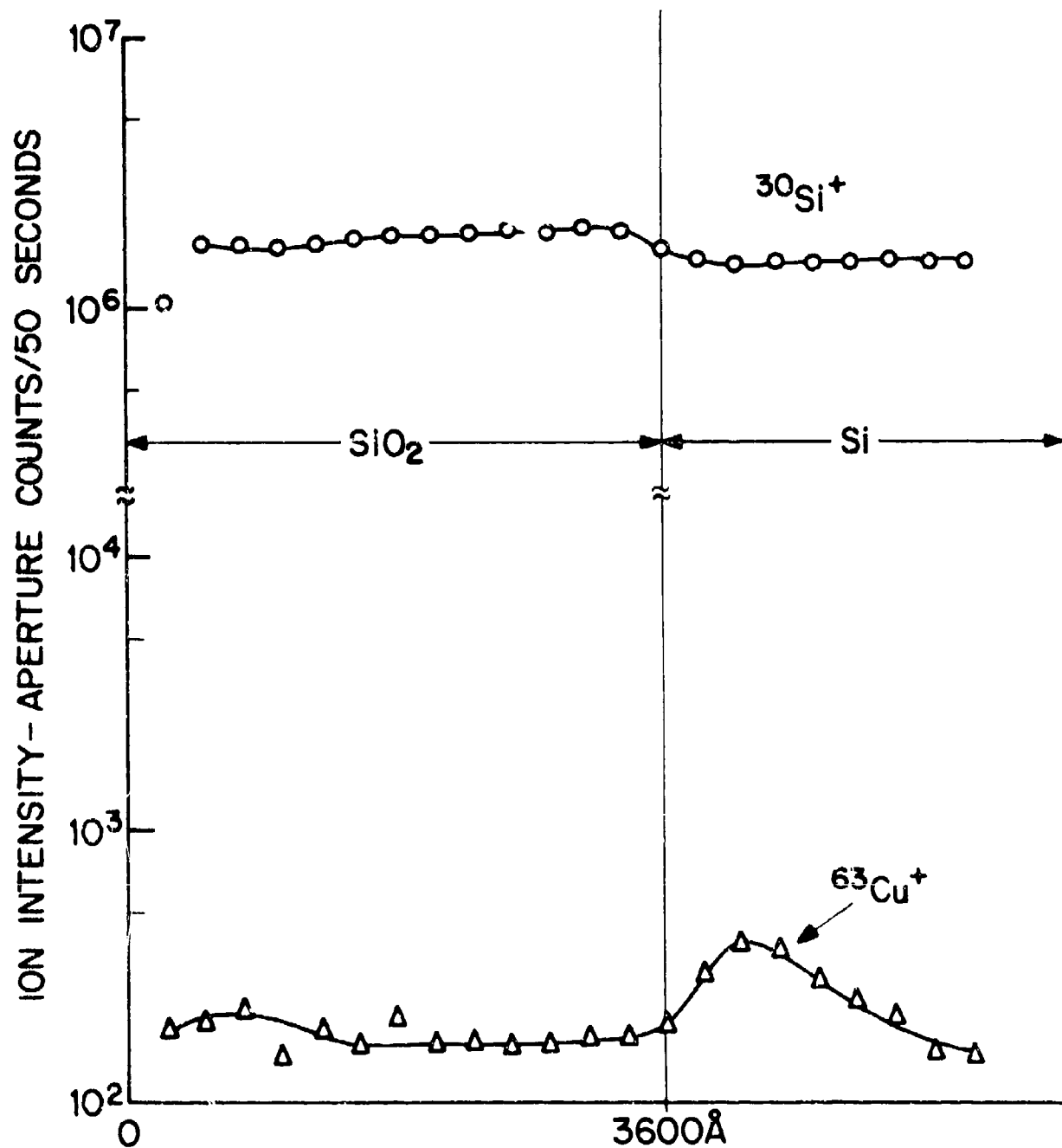
FIGURE 6-3. TYPICAL ^{63}\text{Cu}^+ PROFILE FOR \text{SiO}_2 LAYERS GROWN IN A CHLORINE-CONTAINING AMBIENT
