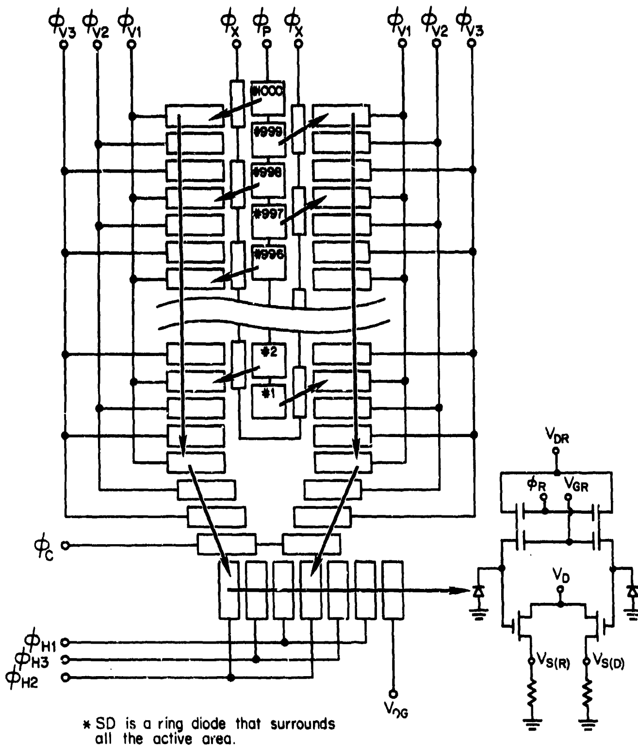
FIGURE 4-1. BLOCK DIAGRAM OF CCLID-1000B
