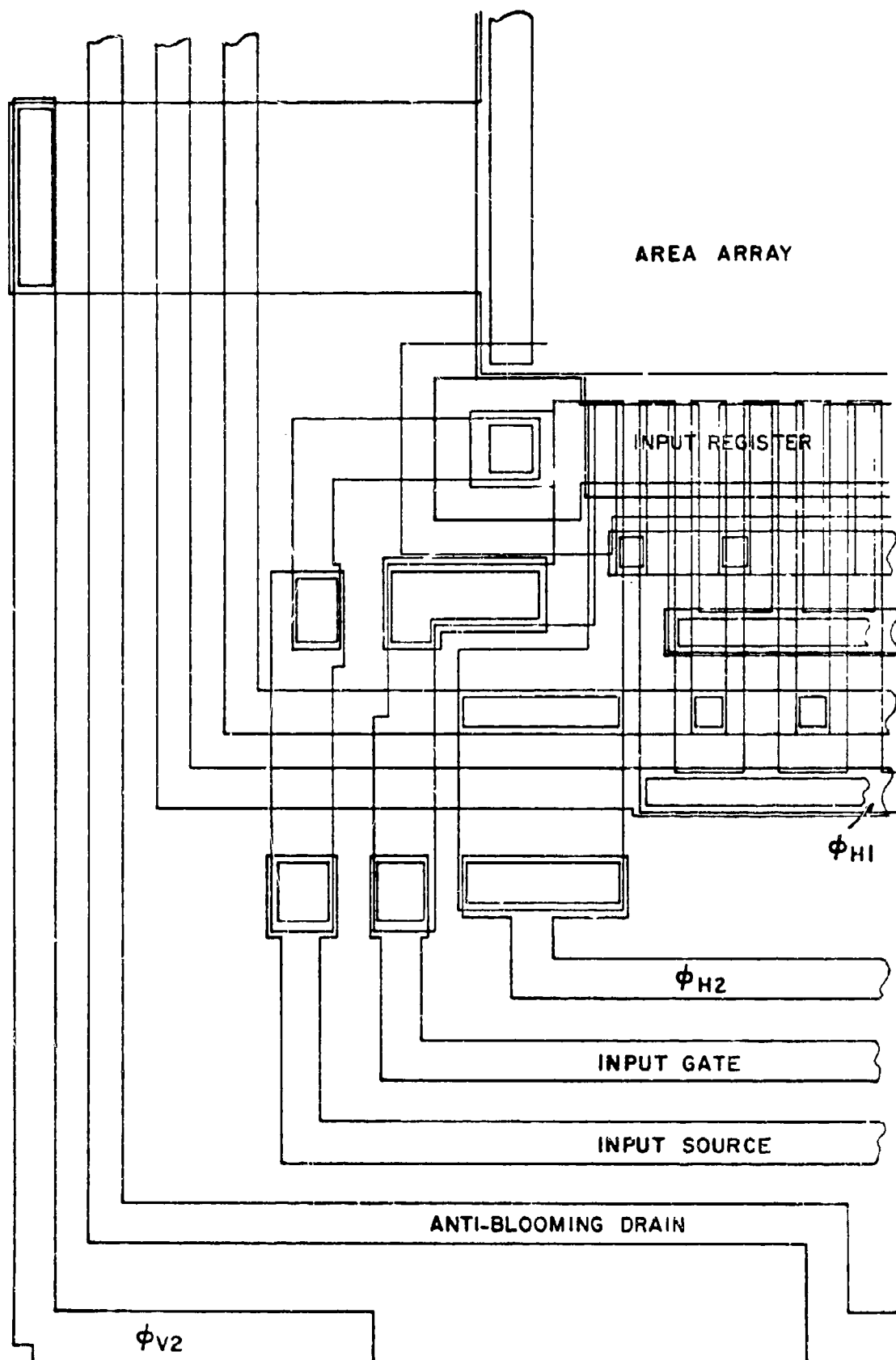
FIGURE 4-49. ELECTRONIC INPUT STRUCTURE
