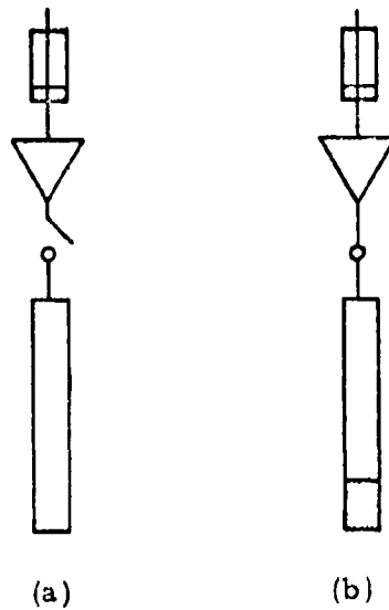
Figure 3.2.2 A Small Signal-Charge Packet in the Input Register Results in a Large Charge Packet in the Output Register.
