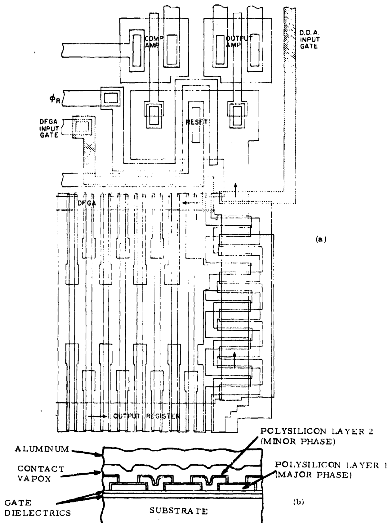
FIGURE 4-33. (a) OUTPUT SECTION OF CCAID-244A AND (b) CROSS-SECTION THROUGH HORIZONTAL GATE STRUCTURE
