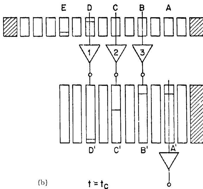
Figure 3.2.4 Charge Distribution in a Three-stage DFGA at Various Time Intervals Showing how Charge Summing is Obtained. (Sheet 1 of 3)
