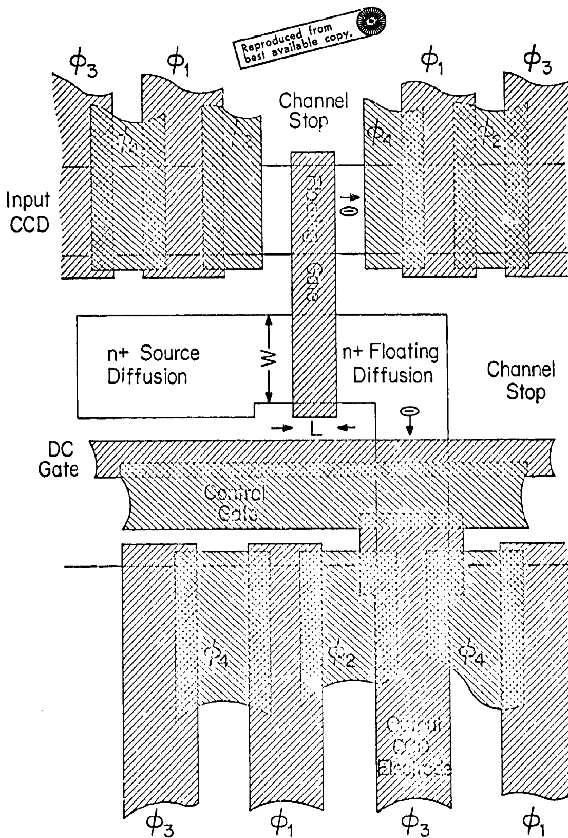
Figure 4.2.1 Layout of a Charge Amplifier in the DFGA.
