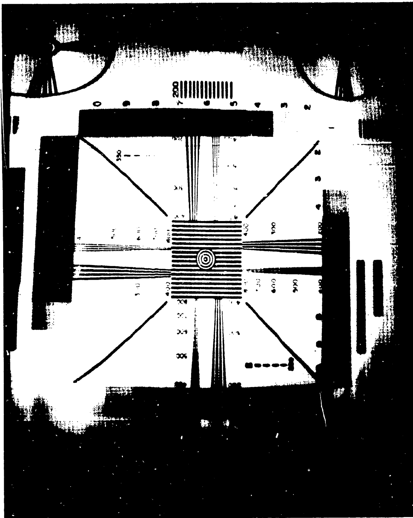
FIGURE 4-13. SLOW-SCAN CAMERA IMAGE
