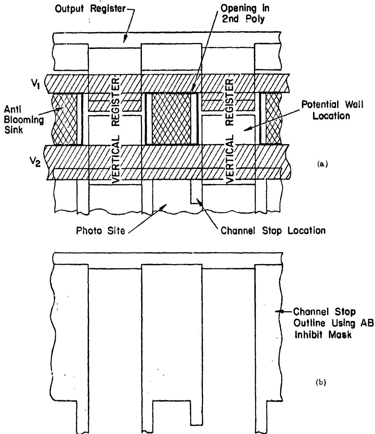
FIGURE 4-35. ANTI-BLOOMING STRUCTURE MODIFICATION (a) Anti-blooming on 244A. (b) Modified channel stop outline when AB inhibit mask is used. The effect of the inhibit mask is to dope the entire anti-blooming structure heavily p-type.
