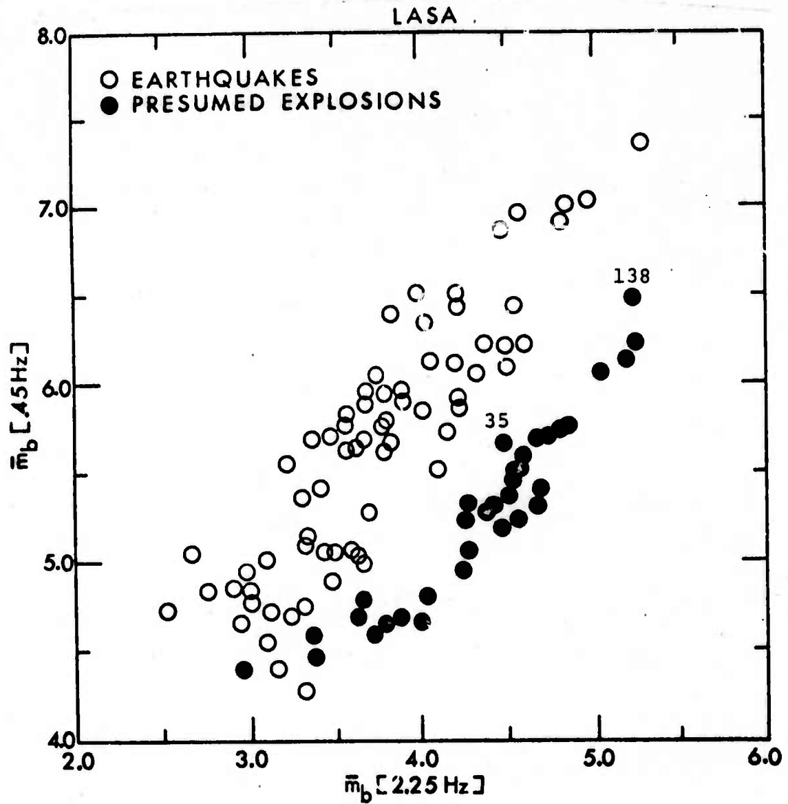
Figure 3.3. Spectral magnitudes, \bar{m}_b , computed at 0.45 Hz and 2.25 Hz. The presumed explosions numbered 35 and 138 occurred at Novaya Zemlya.
