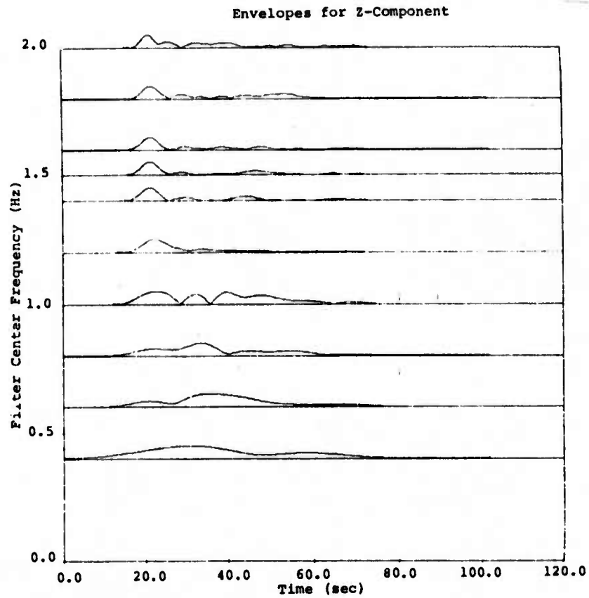
Figure 2.4c. Envelopes for LASA 2030 vertical motion.
