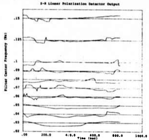
Figure 2.12f. Linear polarization fraction for Piledriver at RKON.
