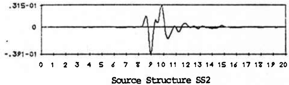
(a) Synthetic seismograms for two near source crustal structures. Amplitude in microns at 1 Hz is indicated.
