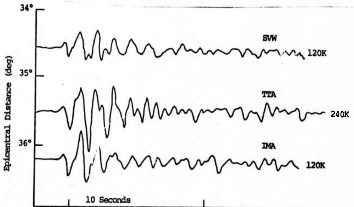
(b) Observed seismograms from the Palmer Network in Alaska for the Yucca Flat event Starwort. The station codes are indicated as is the magnification at 1 Hz.
