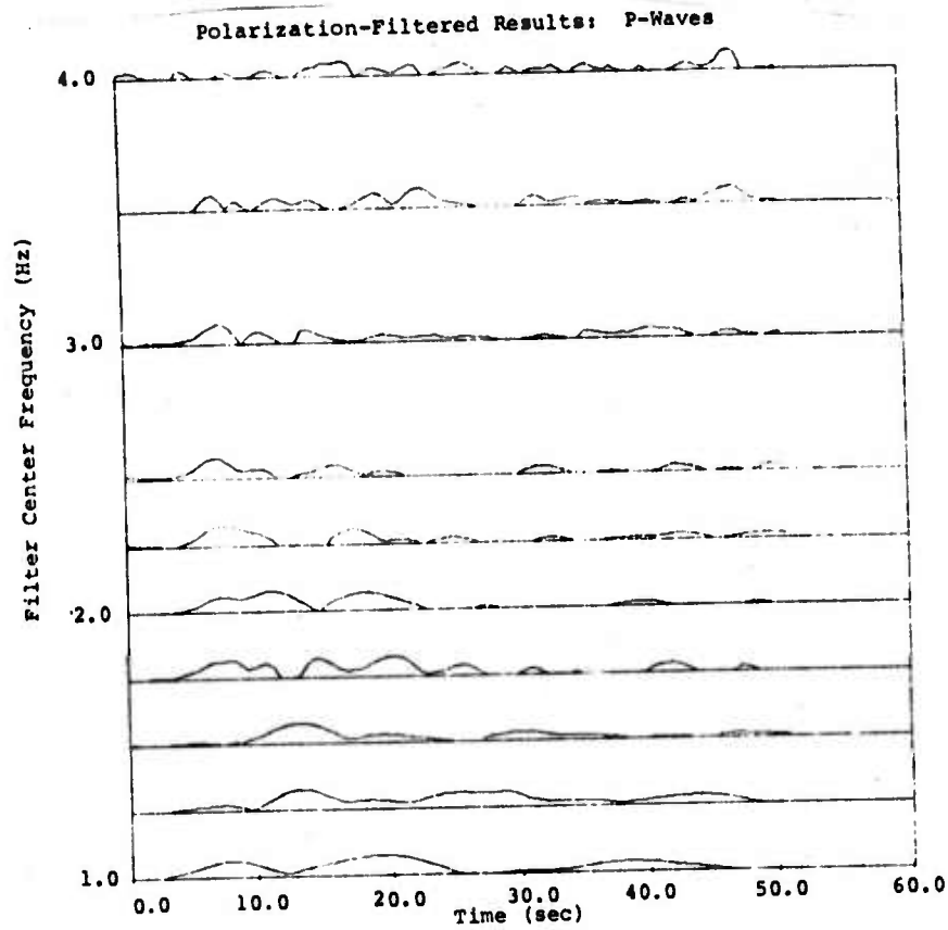
Figure 2.10h. Rex at RKON: P-wave projections.
