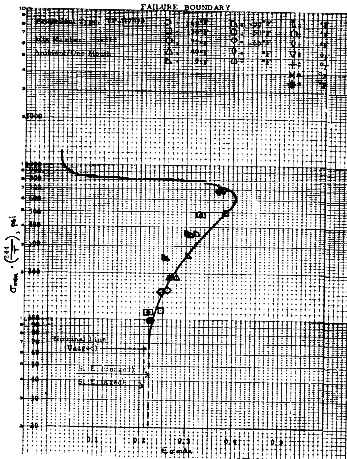
Figure 19. Failure Boundary, TP-H7070 Propellant Stored One Month at Ambient
