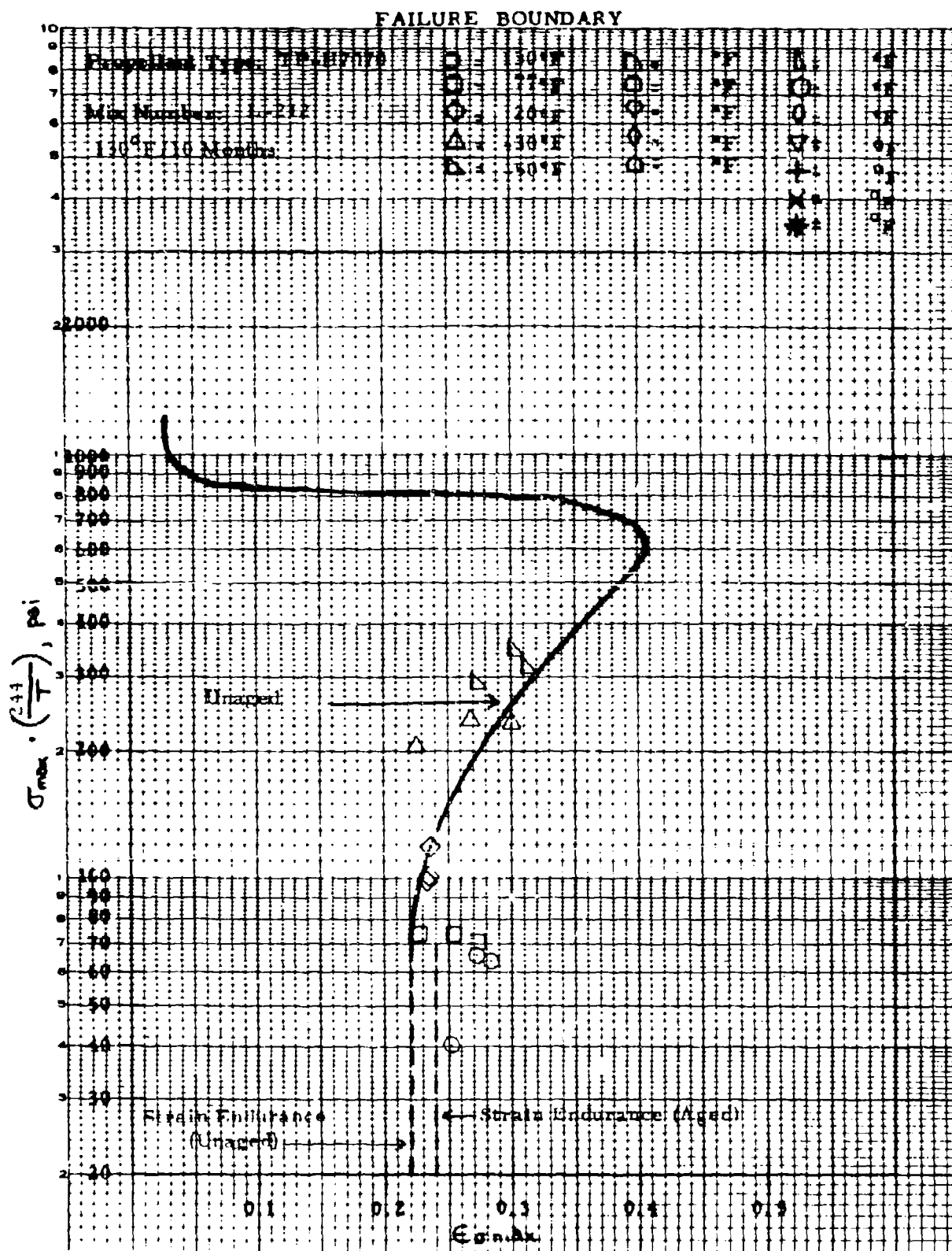
Figure 30. Failure Boundary, TP-H7070 Propellant Stored Ten Months at 130°F
