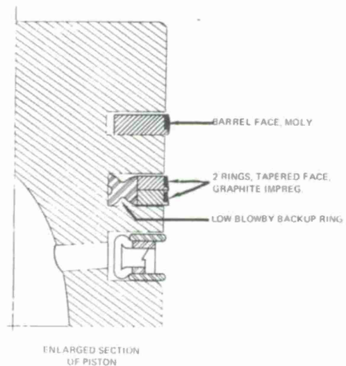
FIGURE 1. TRW LOW-BLOWBY PISTON RING CONFIGURATION
