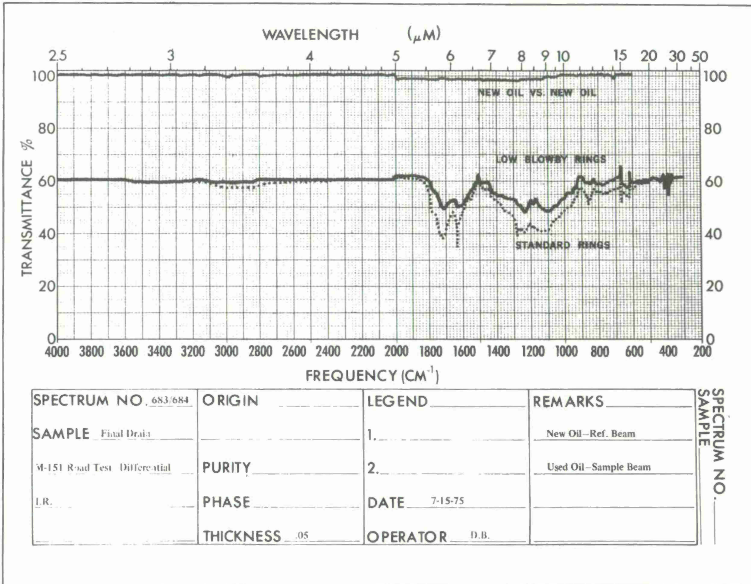
FIGURE 9. DIFFERENTIAL INFRARED ANALYSIS OF FINAL OIL SAMPLES, M-151 ROAD TEST
