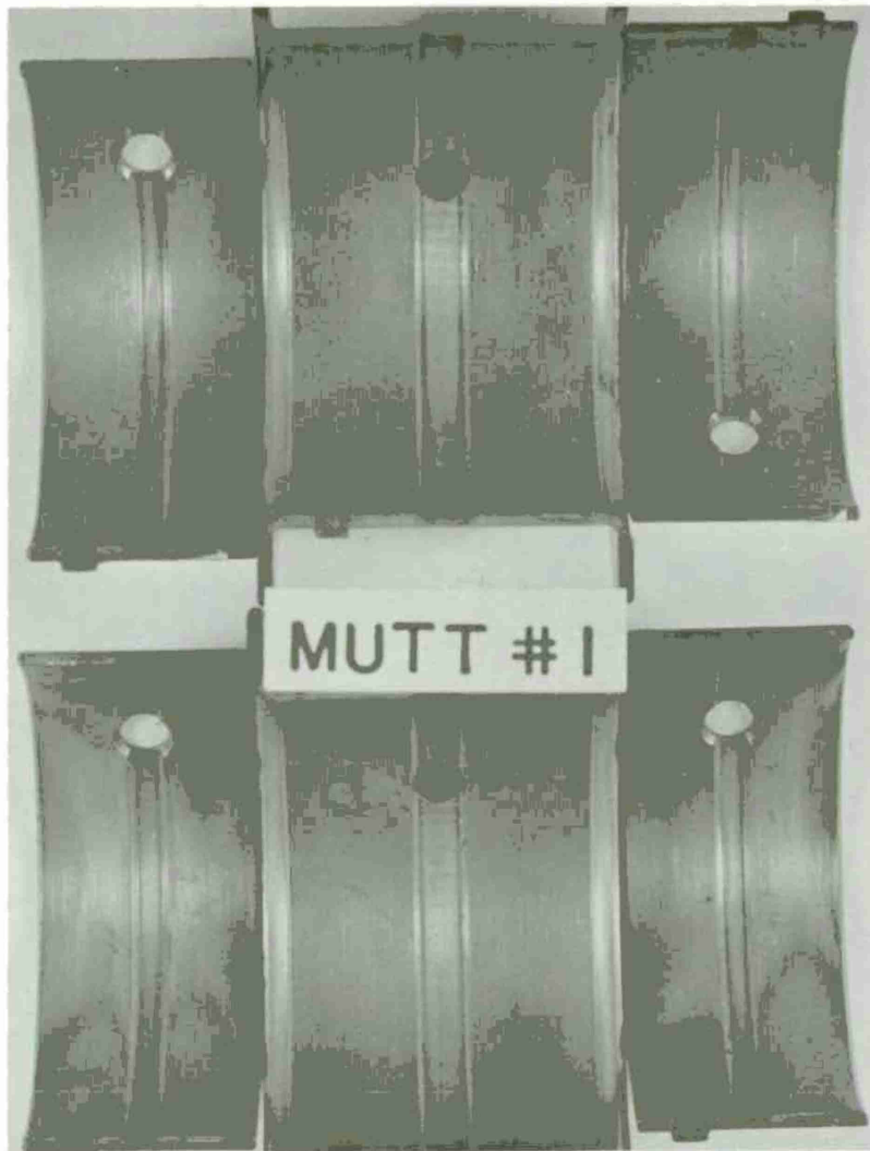
STANDARD RING-EQUIPPED ENGINE MAIN BEARINGS
