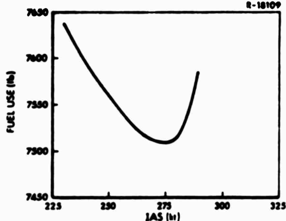
b) FUEL USE VS. CLIMB IAS
