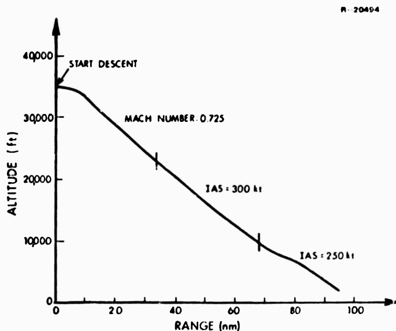
Figure 20 Conventional Descent Profile
