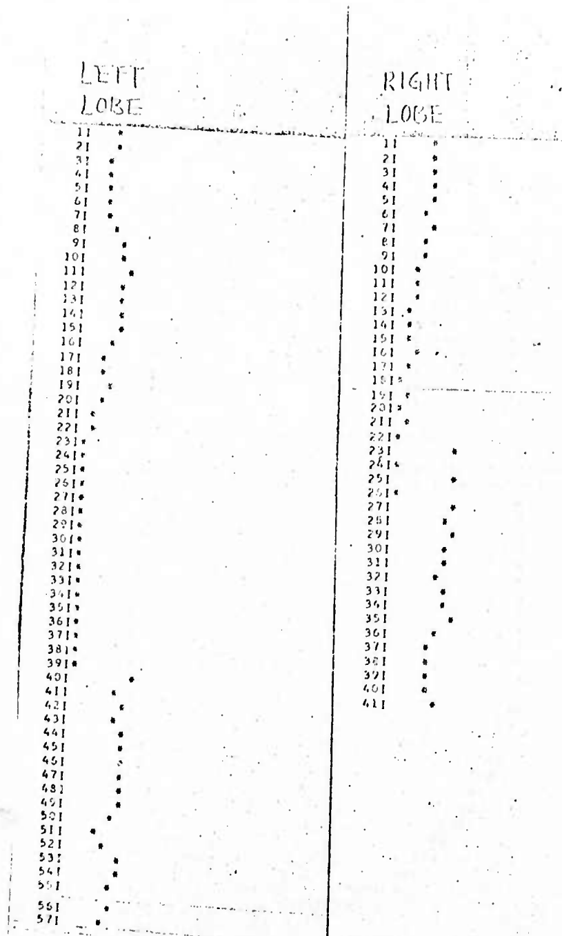
Fig. 14 Scatter plot.
