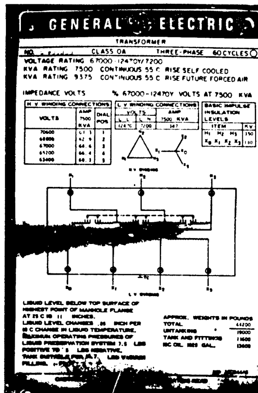
Figure 15. Nameplate of 69 kV/12.47 kV Power Transformer
