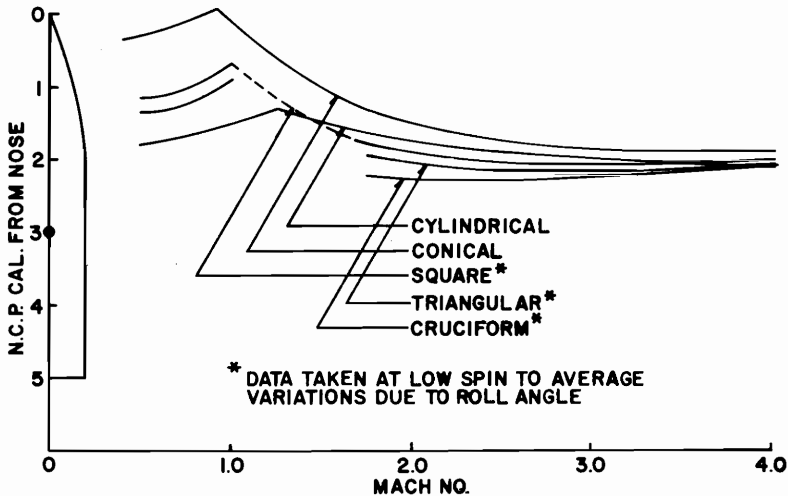
Figure 12. The Normal Force Center of Pressure on the Improved Boattails
