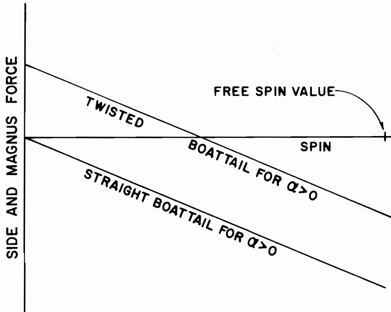
Figure 14. The Side and Magnus Forces on the Straight and Twisted Boattails
