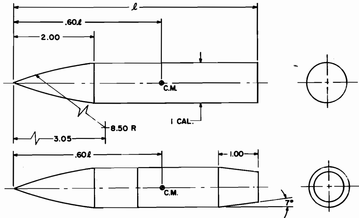
Figure 1. The Cylindrical and Conical Boattail, Dimensions in Calibers, l = 5, 6 , or 7 calibers
