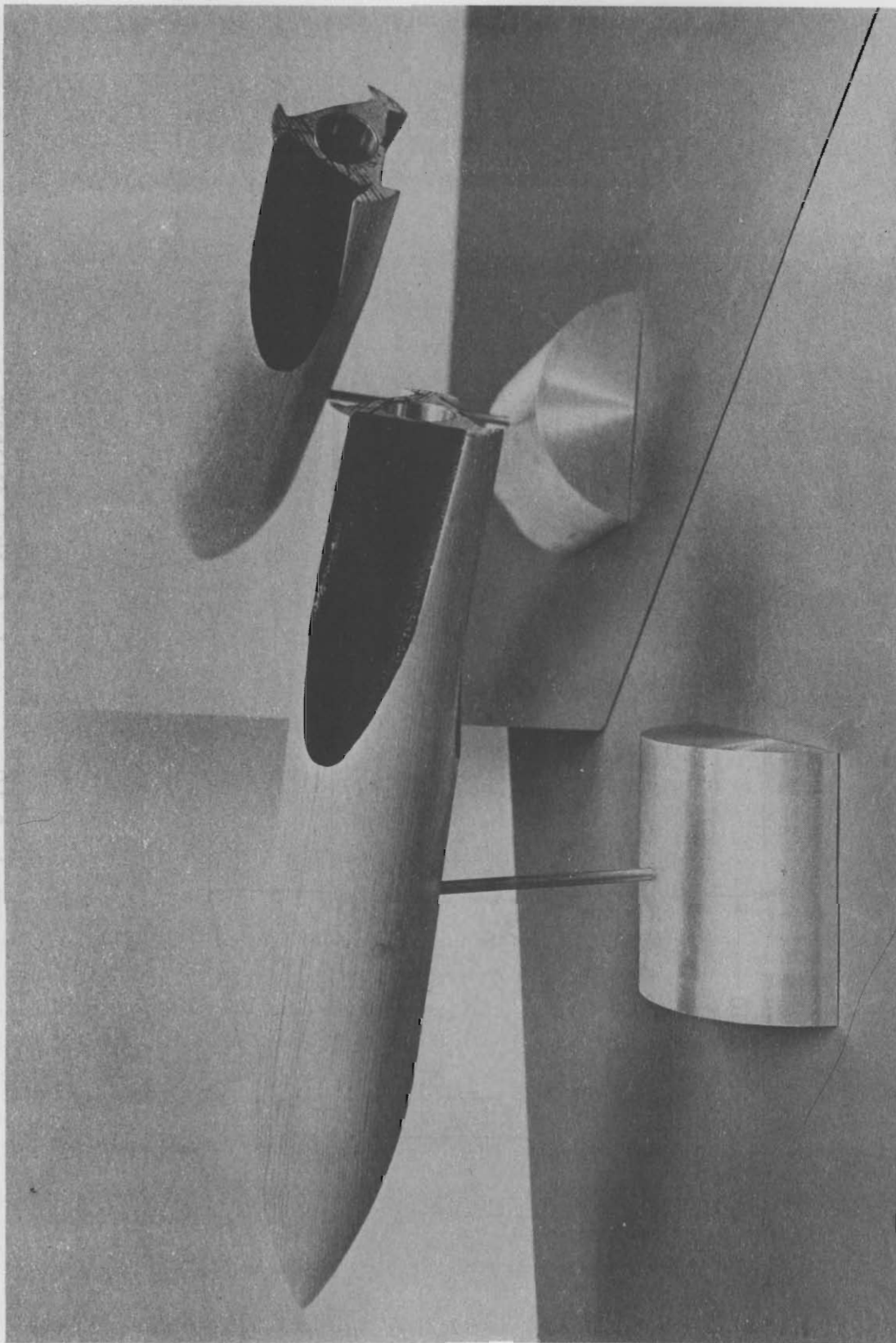
Figure 4. A Canted Boattail
