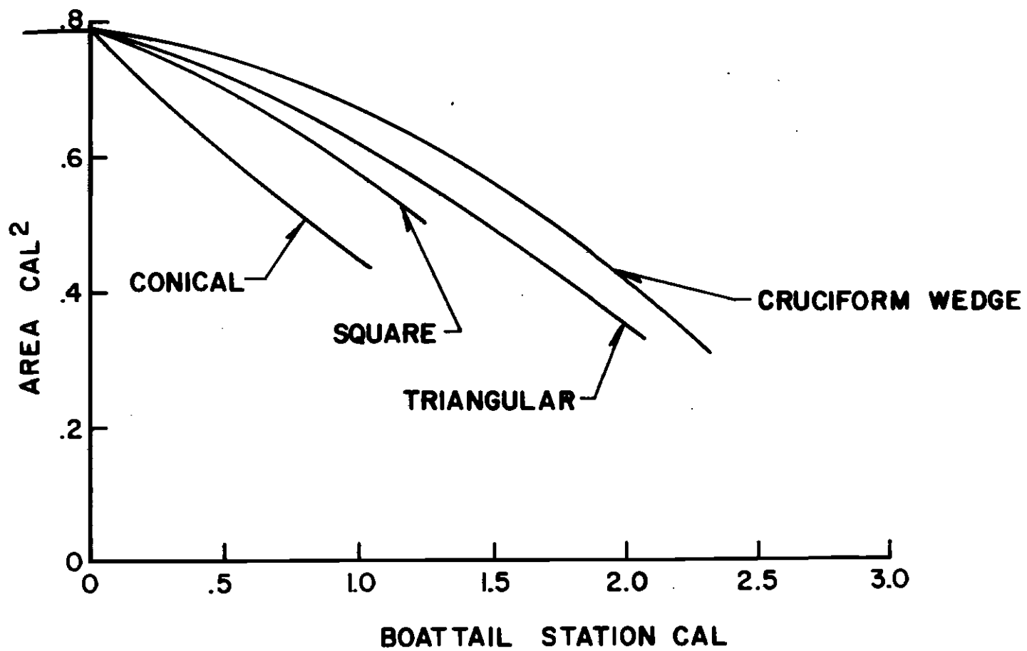
Figure 6. Cross Sectional Areas of 7° Boattails
