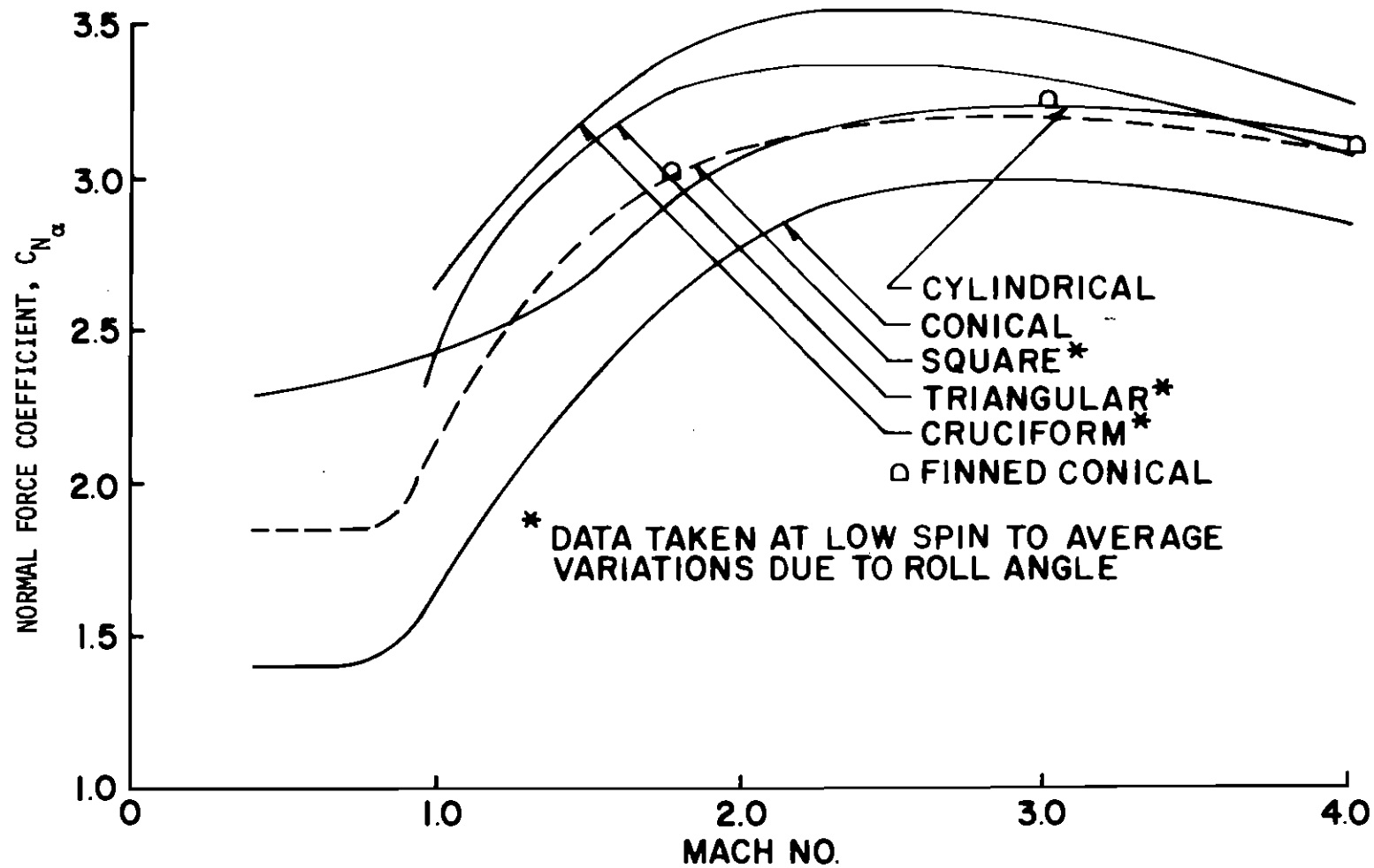
Figure 10. The Normal Force on the Improved Boattail Configurations
