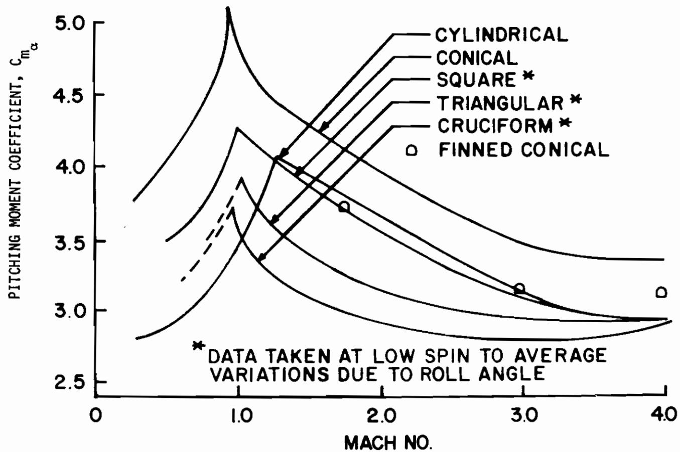
Figure 11. The Pitching Moment on the Improved Boattails
