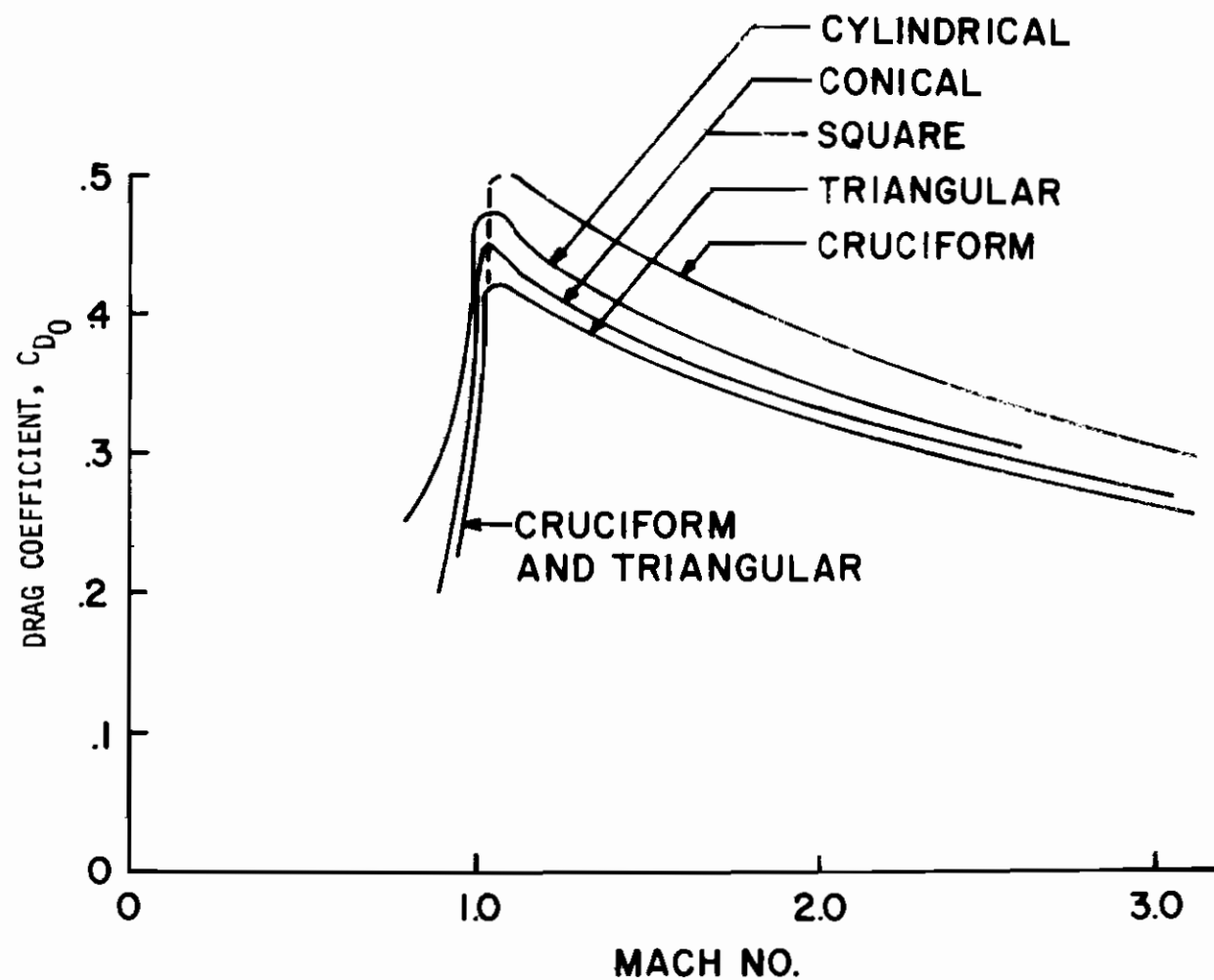
Figure 7. The Zero Yaw Drag of the Improved Boattails
