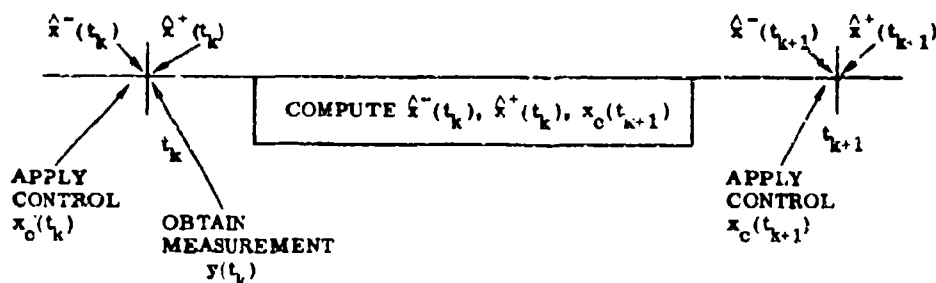
Figure 1. Time Sequence of Estimation and Control Computations
