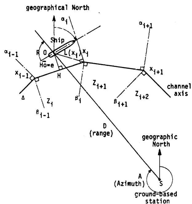
Figure 1.: Ship sailing along the channel
