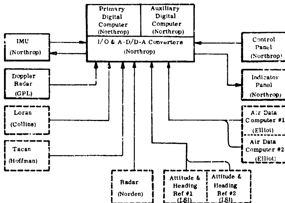
Figure 5. Block Diagram of C-5 Navigation System Equipment.
