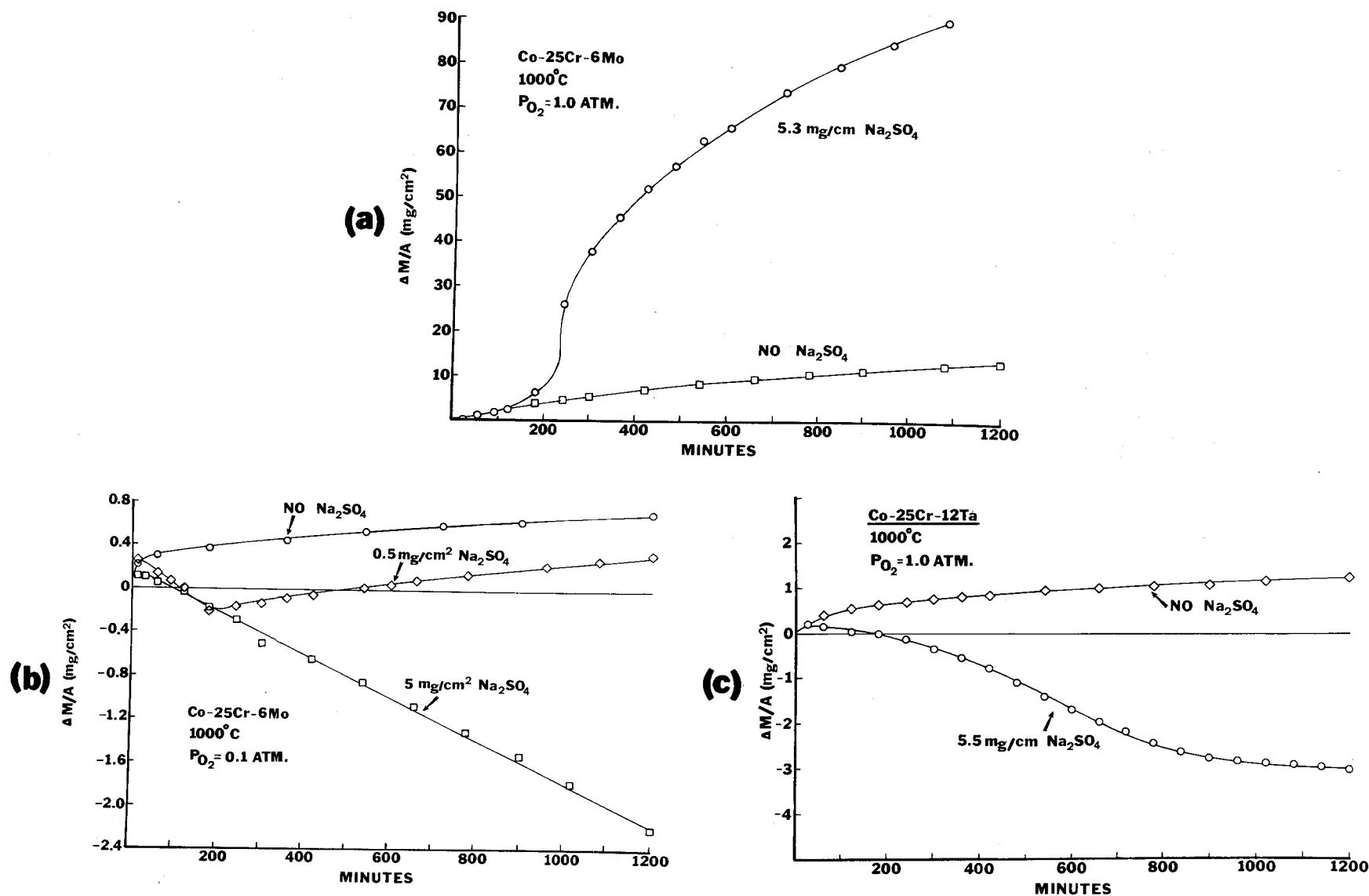
Figure 67 Weight change versus time curves obtained for the isothermal oxidation of Co-25Cr-6Mo in 1 atm (a) and 0.1 atm (b) of oxygen and Co-25Cr-12Ta (c) alloys with and without deposits of \text{Na}_2\text{SO}_4 .
