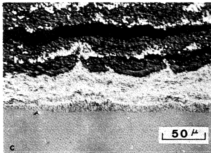
Figure 47 Photomicrographs and microprobe images of the microstructure of Co-25Al-12W after 20 hrs oxidation in 1 atm oxygen at 1000°C. Prior to oxidation this specimen was coated with 5 mg/cm 2 Na 2 SO 4 and annealed for 1 hr in argon at 1000°C. (a) Optical micrograph showing overall scale thickness. (b) Optical micrograph showing details at the scale/alloy interface. (c) Electron backscatter image of scale/alloy interface. (d) Tungsten X-ray image showing that tungsten is enriched in the oxide scale at the alloy/scale interface.
