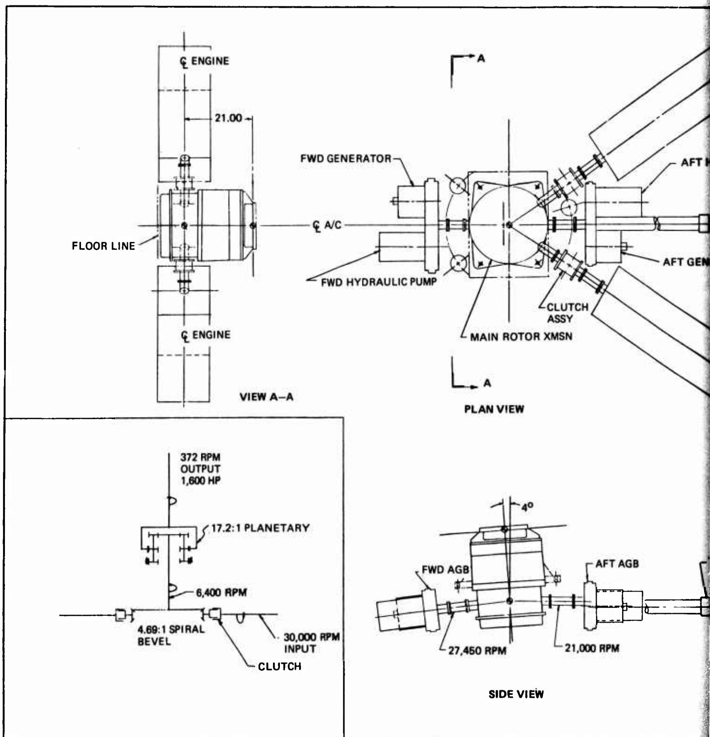
Figure 5. Free Planet Version for Direct Engine Input.
