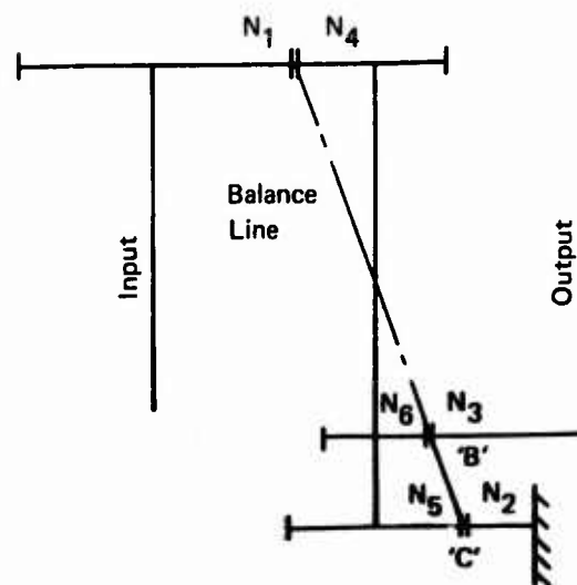
Free Planet Schematic
