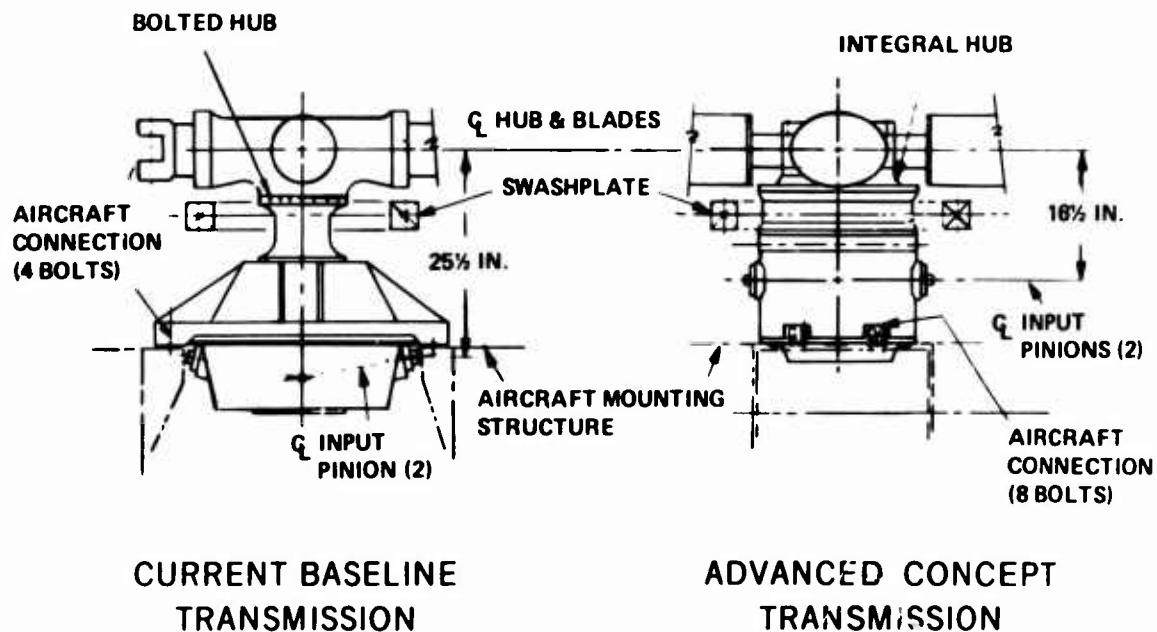
Figure 19. Main Transmission Configuration Comparison
