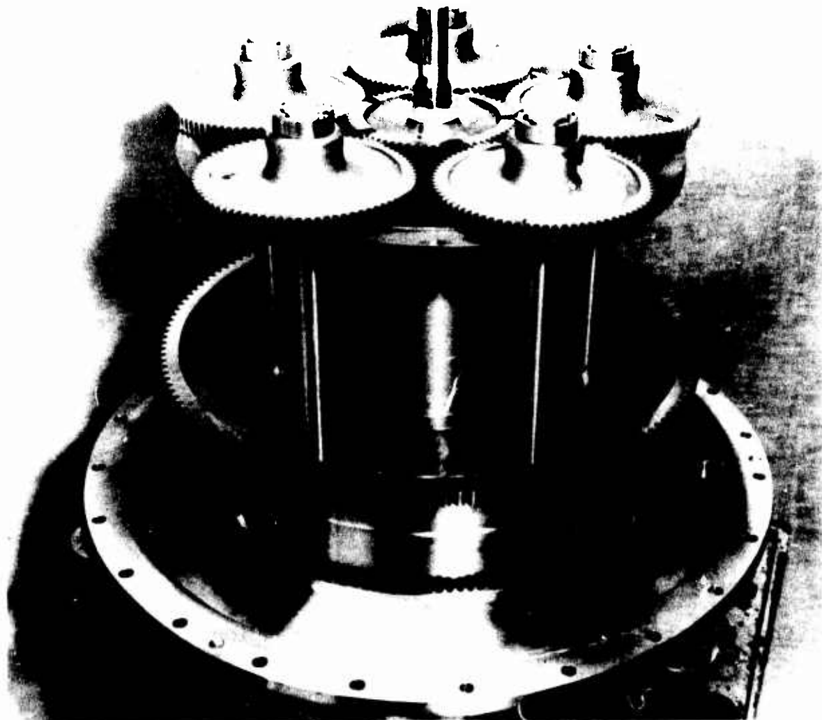
Figure 1. FP500 Series Free Planet Assembly (Curtiss-Wright).
