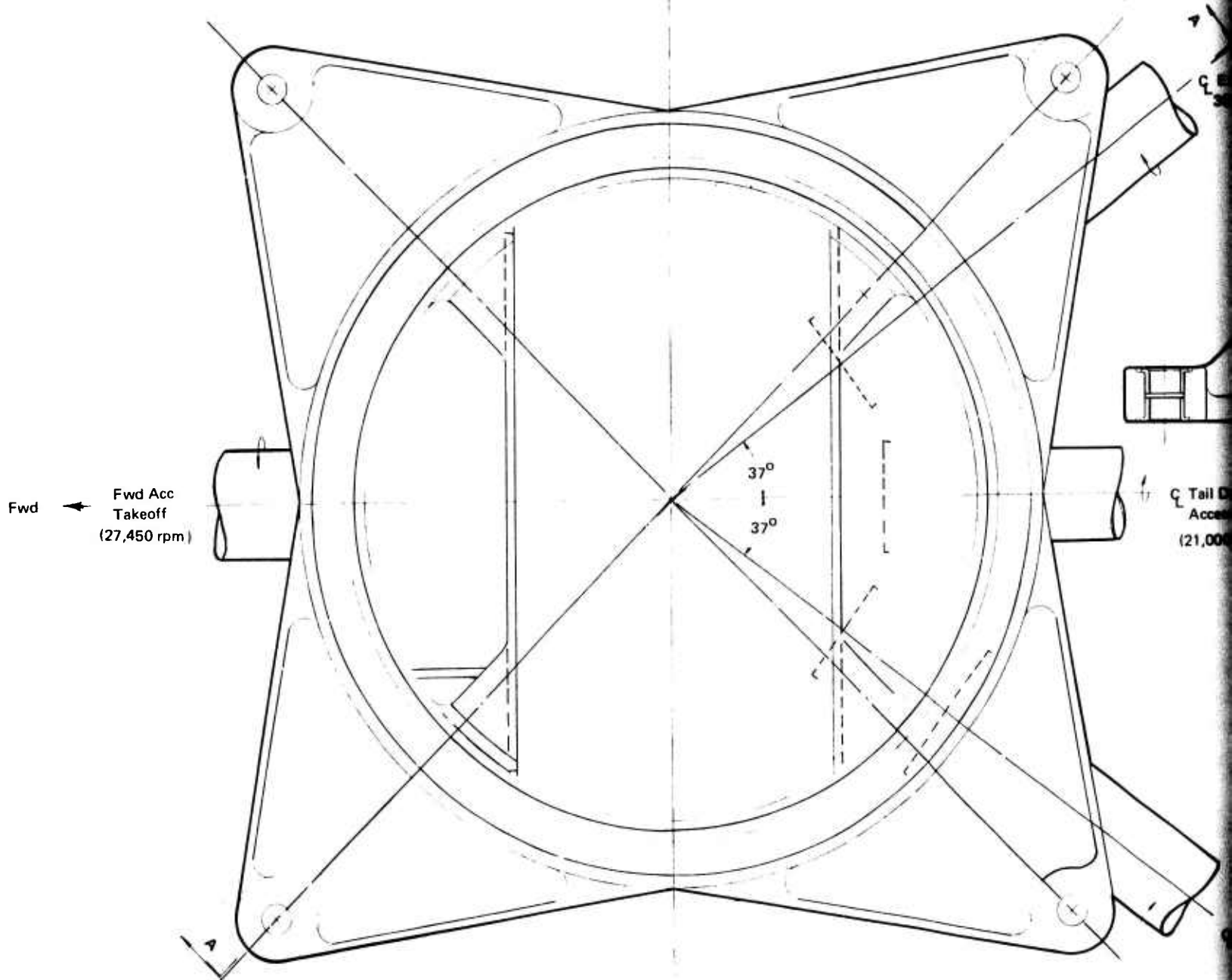
Figure 10. Free Planet Application Study Configuration IV (17.2:1 Free Planetary).
