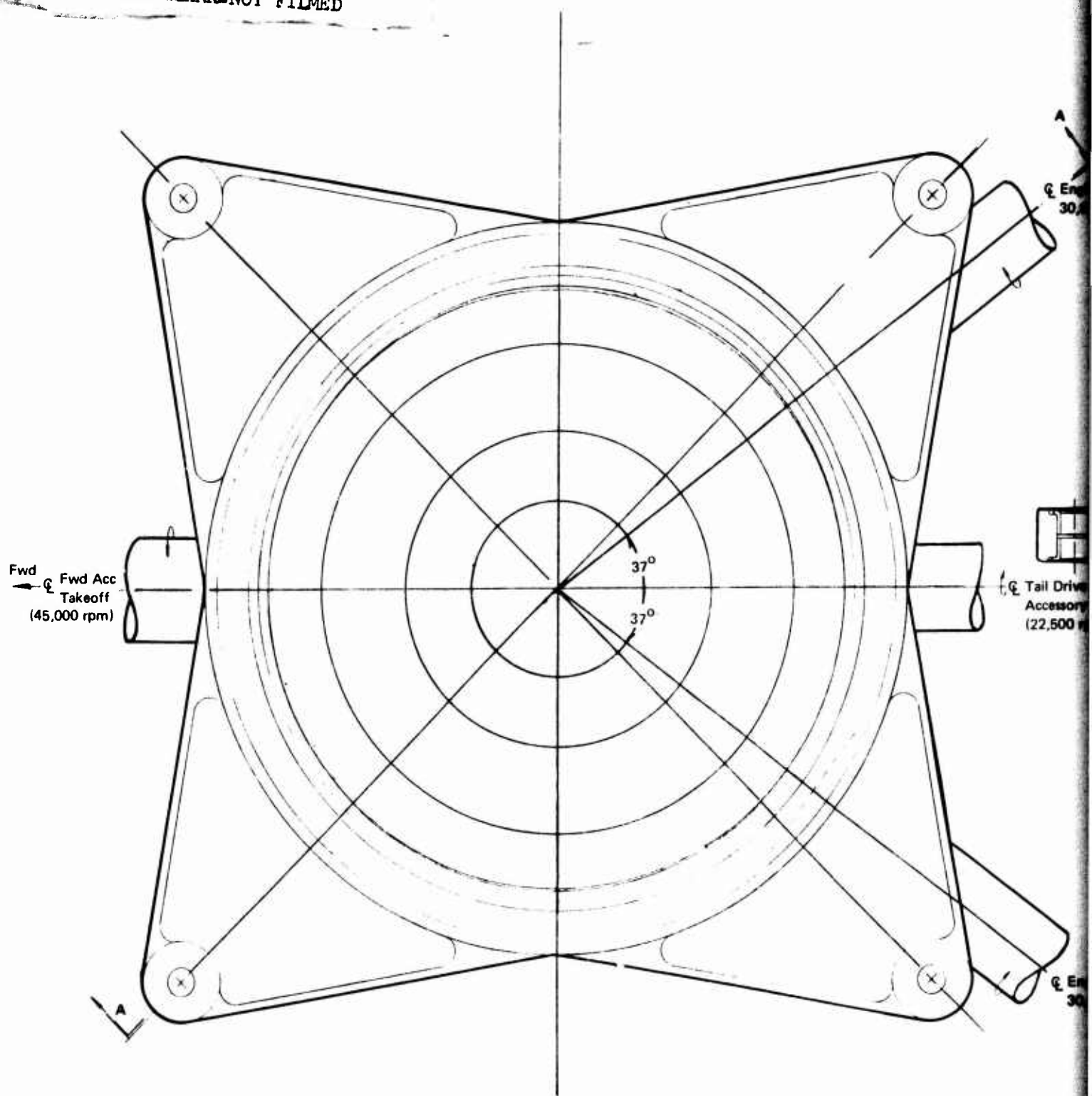
Figure 9. Free Planet Application Study Configuration III (17.2:1 Conventional Planetary).
