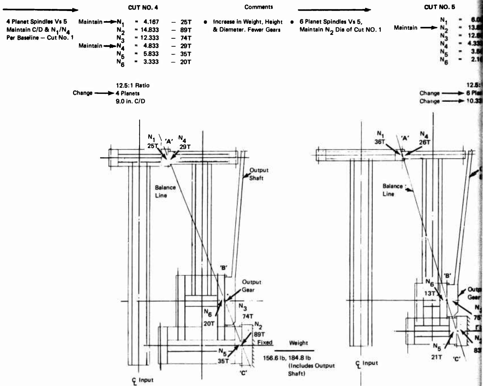
Figure 12. Free Planet Study Parametric Study (1,604 hp, 372 rpm).
