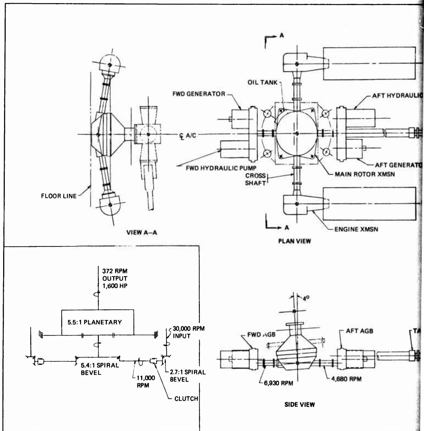
Figure 2. Conventional Transmission - Configuration No. 1.
