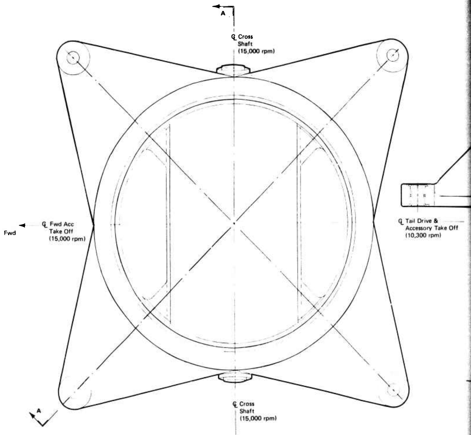
Figure 8. Free Planet Application Study Configuration II and IIa (12.9:1 Free Planetary).
