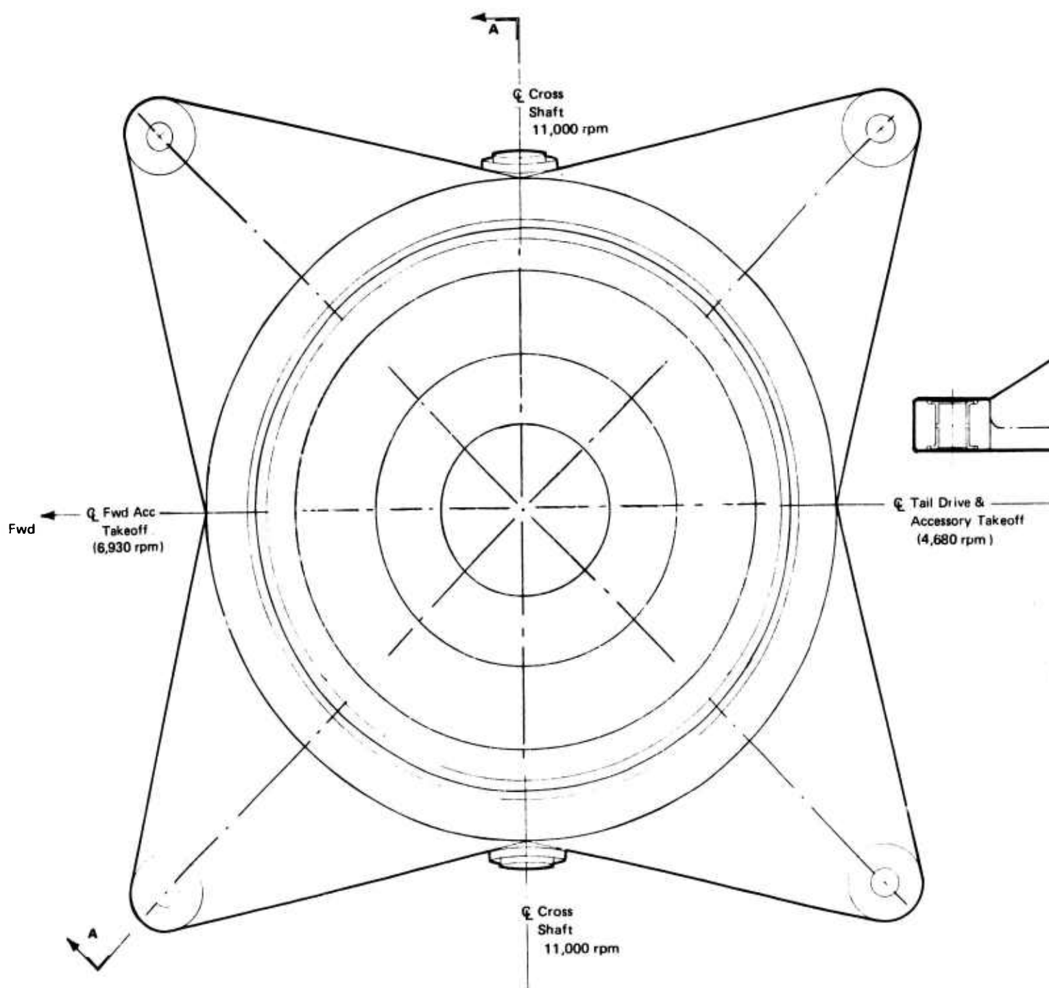
Figure 7. Free Planet Application Study Configuration I (5.5:1 Planetary Ratio, Conventional).
