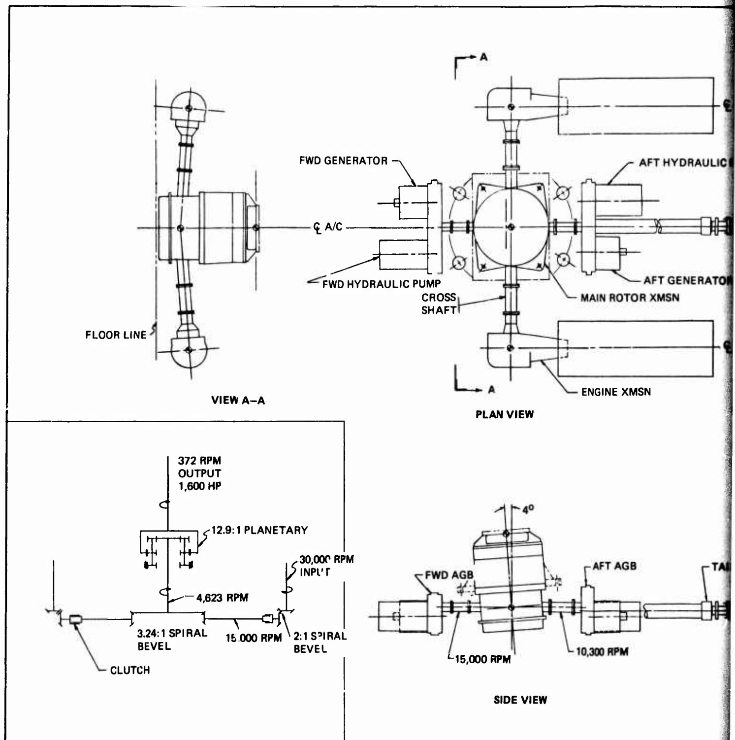
Figure 3 . Free Planet Version of Configuration No. 1.
