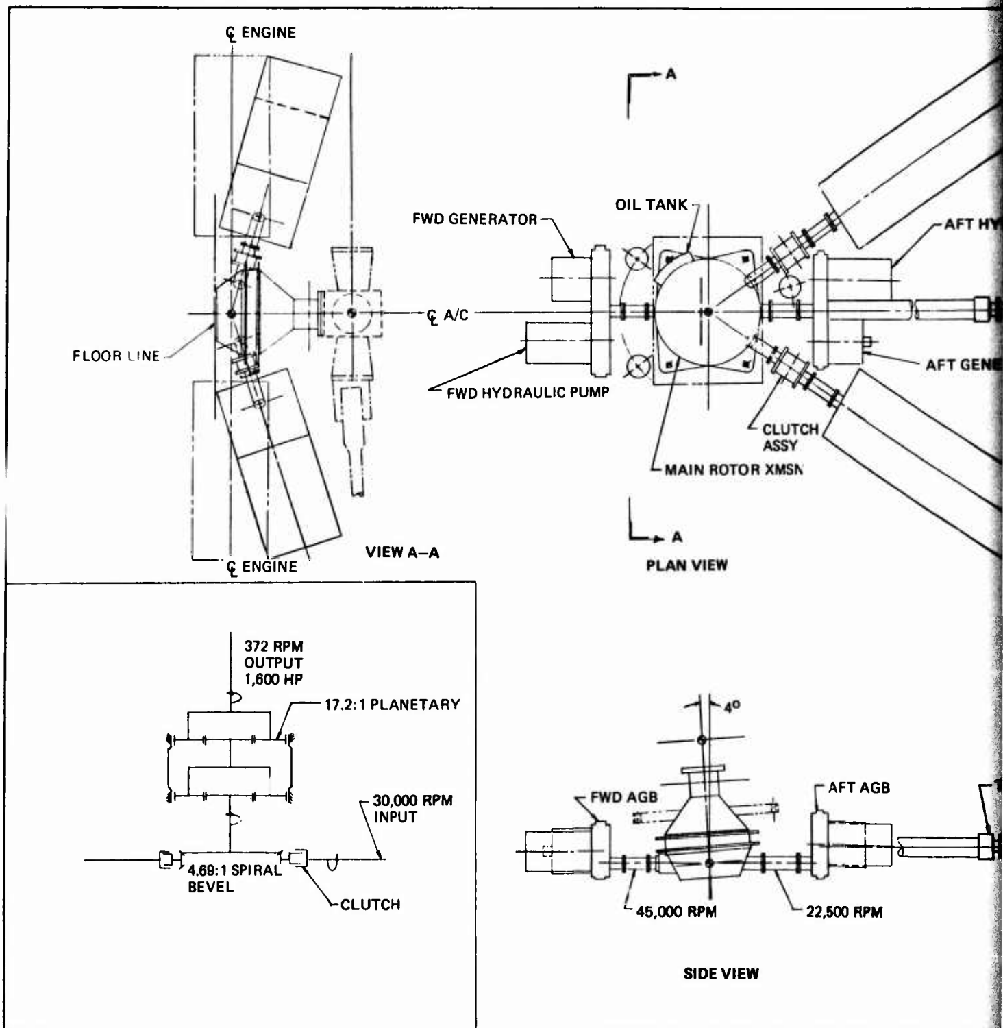
Figure 4. Conventional Version for Direct Engine Input.
