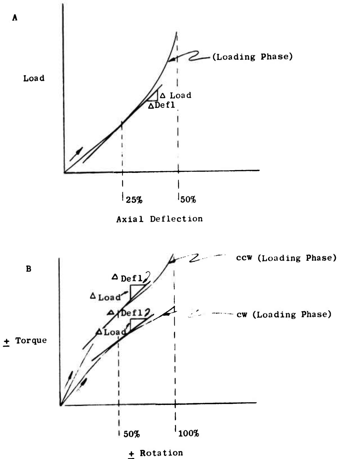
Figure 3. Samples of Load-Deflection Curves
