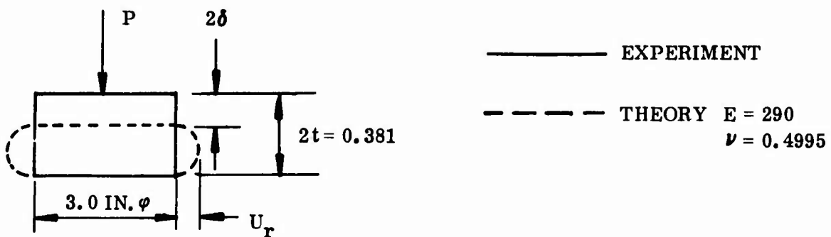
Figure 6-6. Comparison of Theory and Experiment (Compression Specimen)
