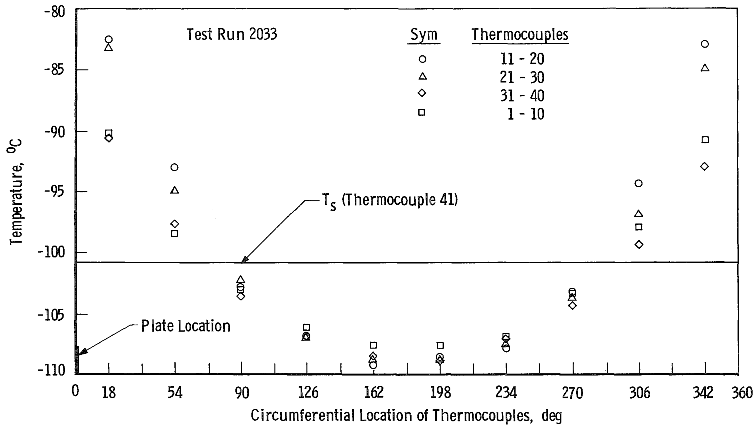
Figure 24. Sphere temperature distribution for 125°C plate temperature without solar simulation.
