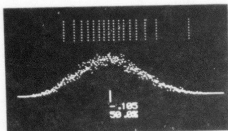
K_2 (voiced)
