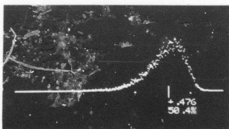
K_1 (silence)
