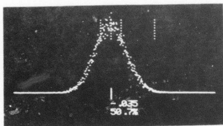
K_9 (voiced)
