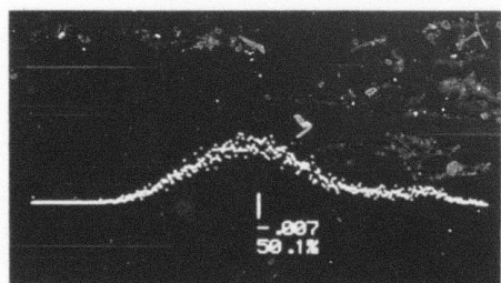
K_0 (silence)
