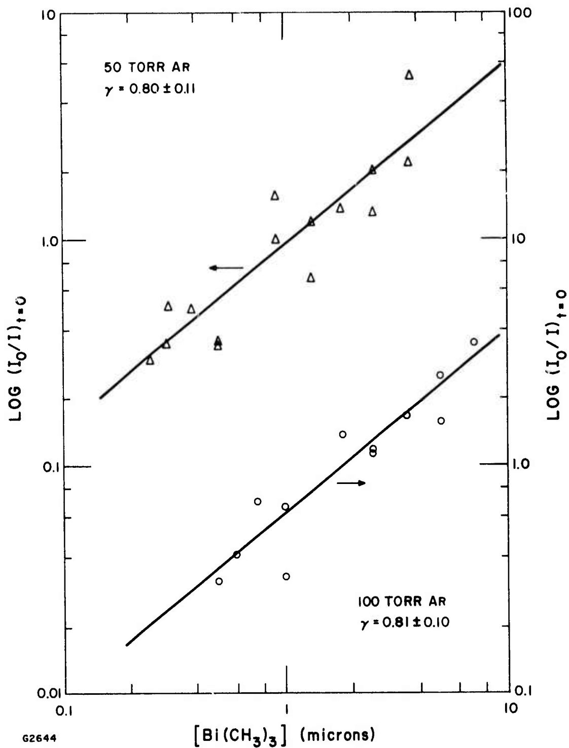
Fig. 5 \gamma - Plot for Bi ^2D_{3/2}^o State Monitored at 2848 Å
