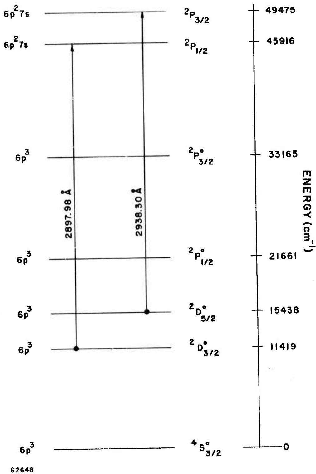
Fig. 4 Bismuth Partial Energy Level Diagram
