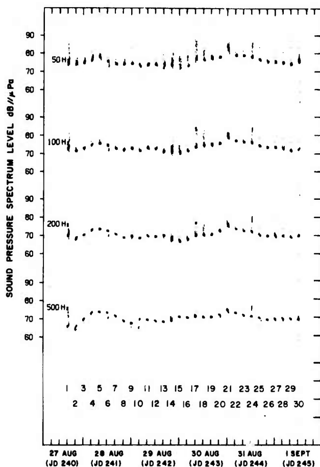
Fig. 6 — Hydrophone data, 2375-m depth
