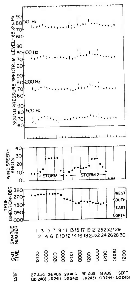
Fig. 7a — Acoustic data and environmental observations
