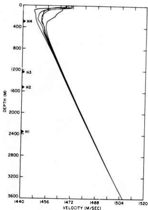
Fig. 2 — Profiles of sound speed vs depth for October
