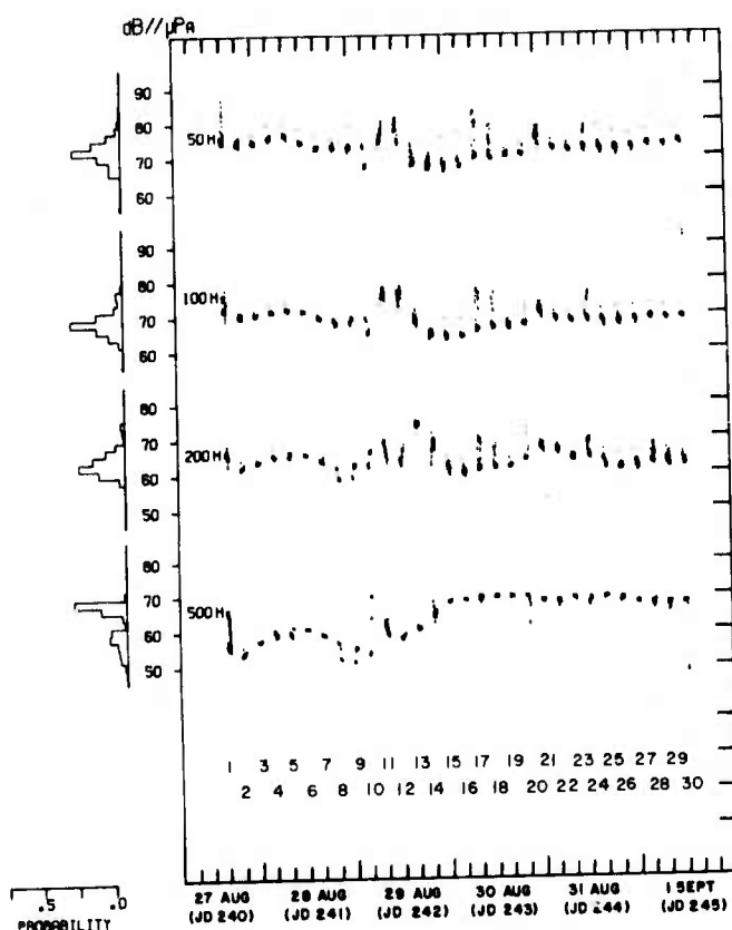
Fig. 5 — Hydrophone data, 1537-m depth
