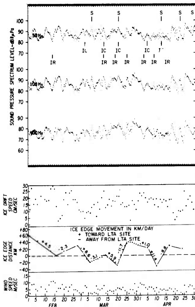
Fig. 11 — Acoustic data and environmental observations, February-April 1973
