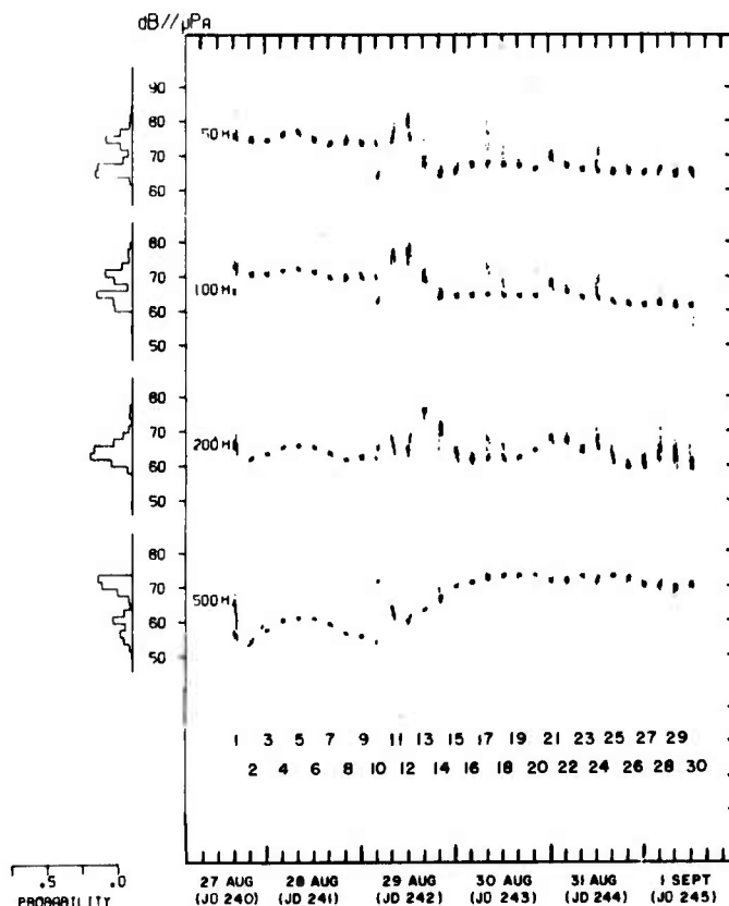
Fig. 3 — Hydrophone data, 241-m depth
