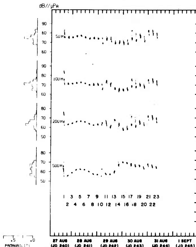
Fig. 4 — Hydrophone data, 1232-m depth
