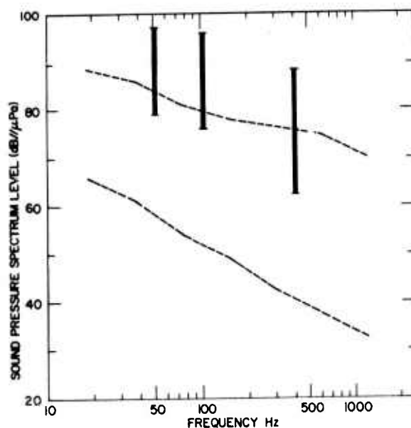
Fig. 12 — Comparison of 50-, 100-, and 400-Hz data to previous measurements
