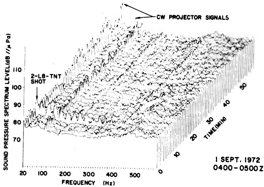
Fig. 8b — Isometric plot during developed seas (sample 28)
