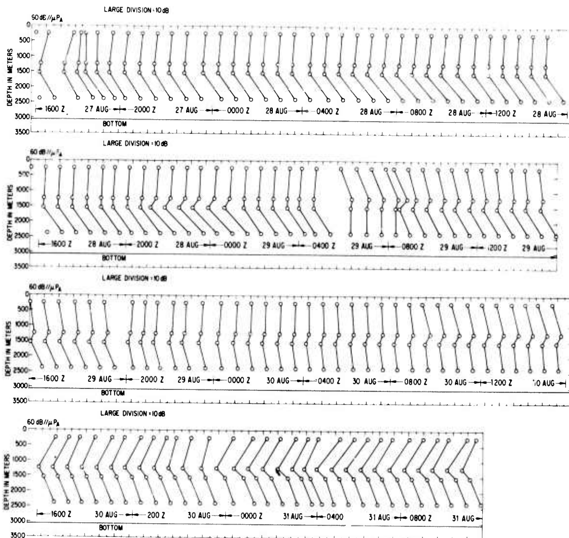
Fig. 10 — Ambient noise depth profiles at 500 Hz
