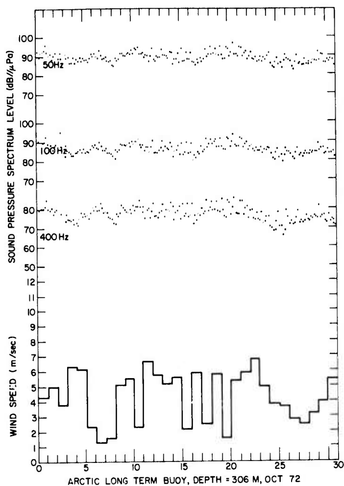
Fig. A5 — Acoustic data, October 1972
