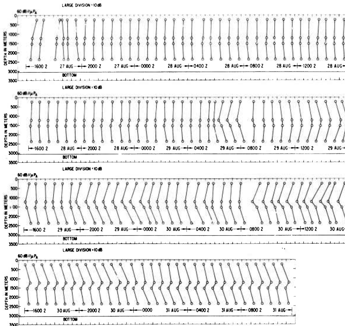
Fig. 9 — Ambient noise depth profiles at 50 Hz
