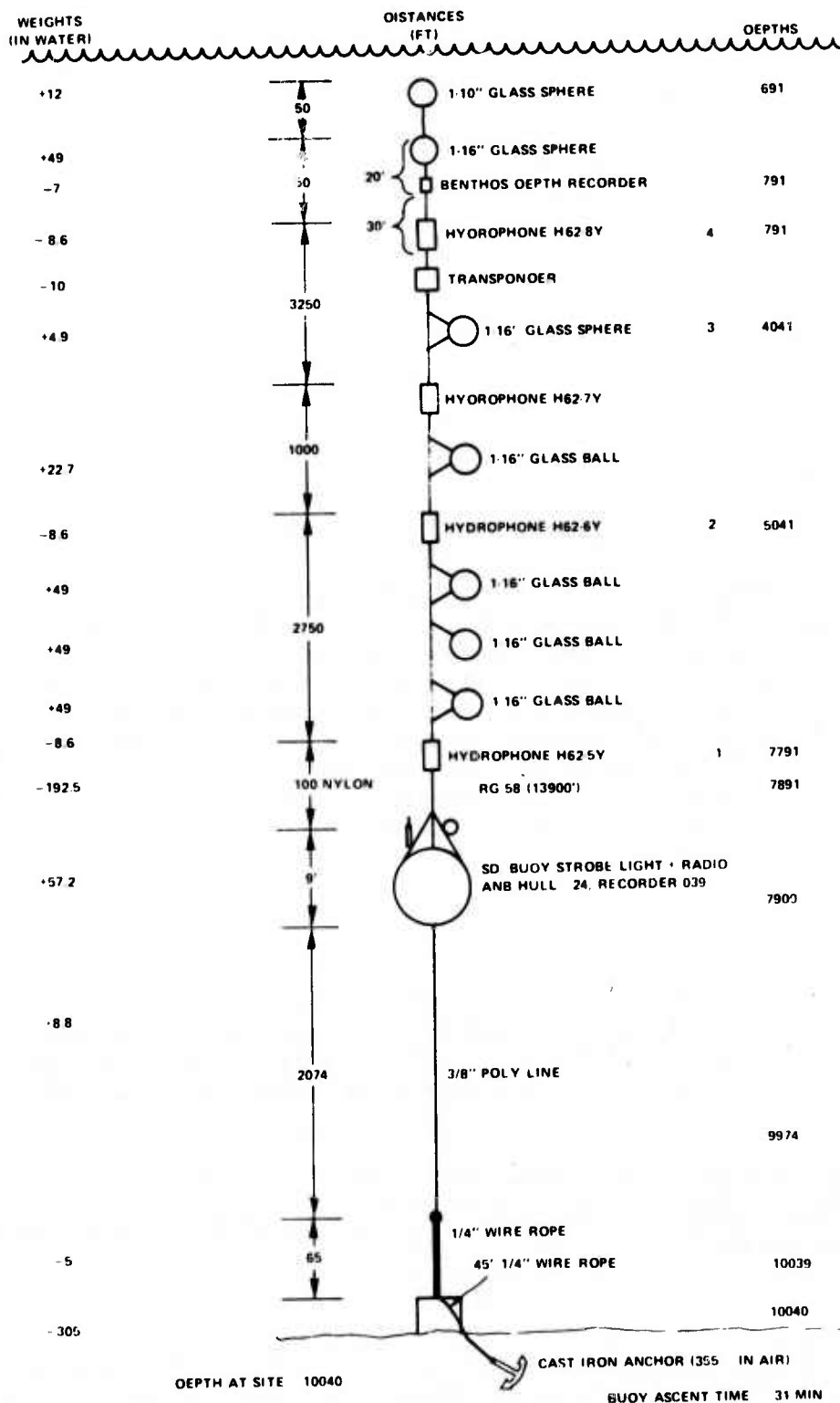
Fig. A1 — Mechanical arrangement of the STA
