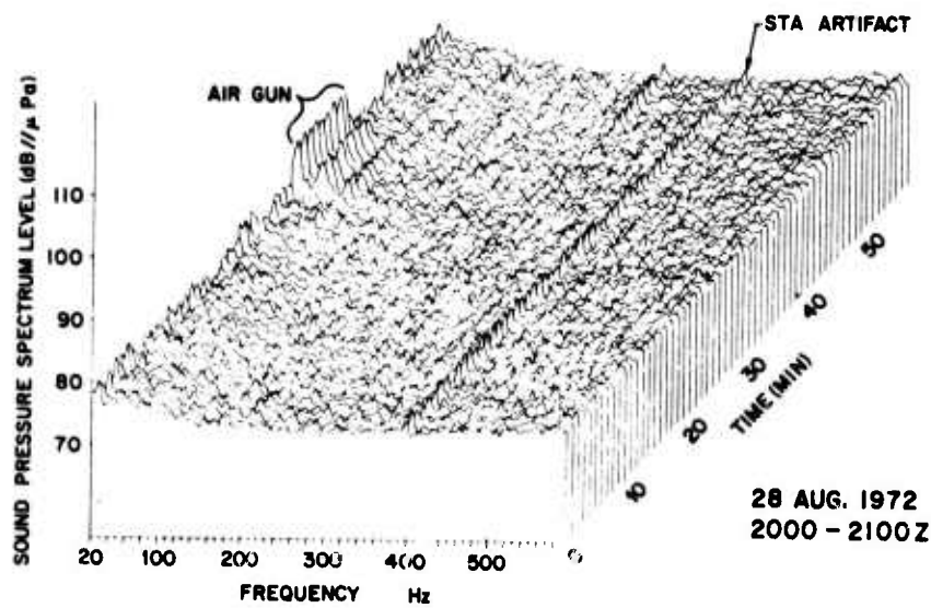
Fig. 8a — Isometric plot during developing seas (sample 8)
