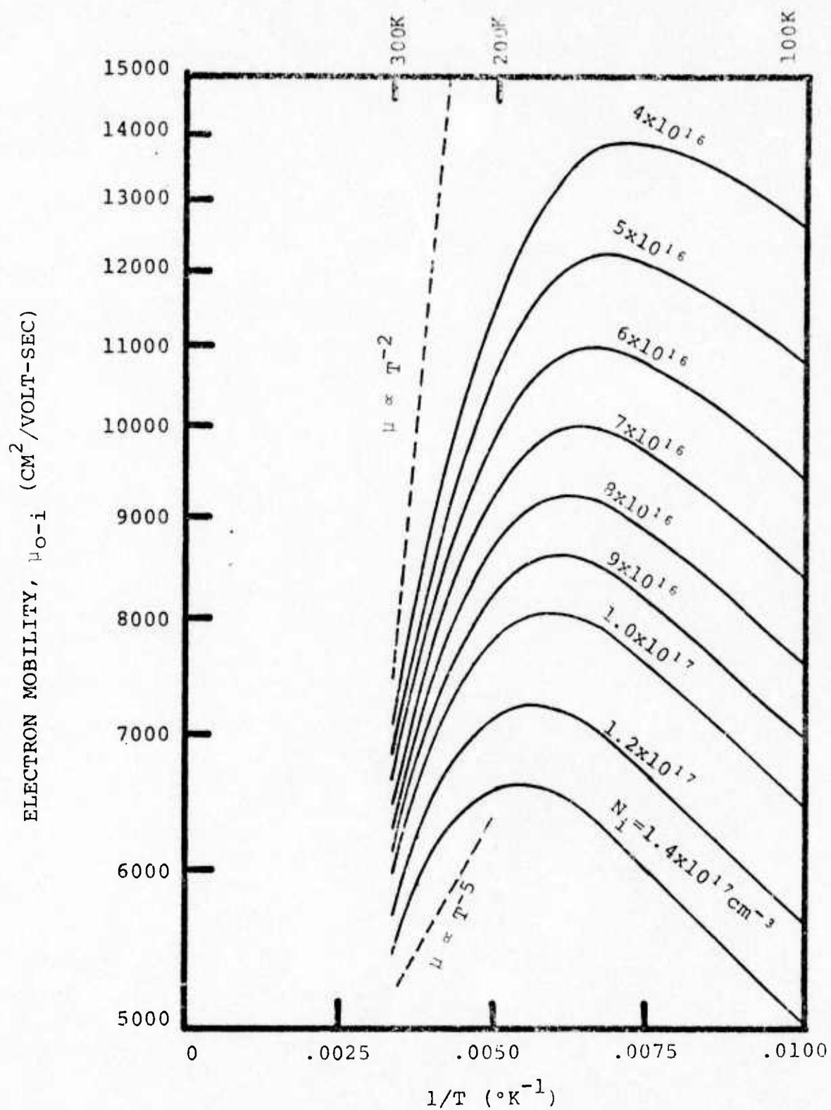
FIGURE 2.4 COMBINED MOBILITY LIMITS DUE TO POLAR OPTICAL PHONON AND IONIZED IMPURITY SCATTERING FOR InAs 0.61 P 0.39
