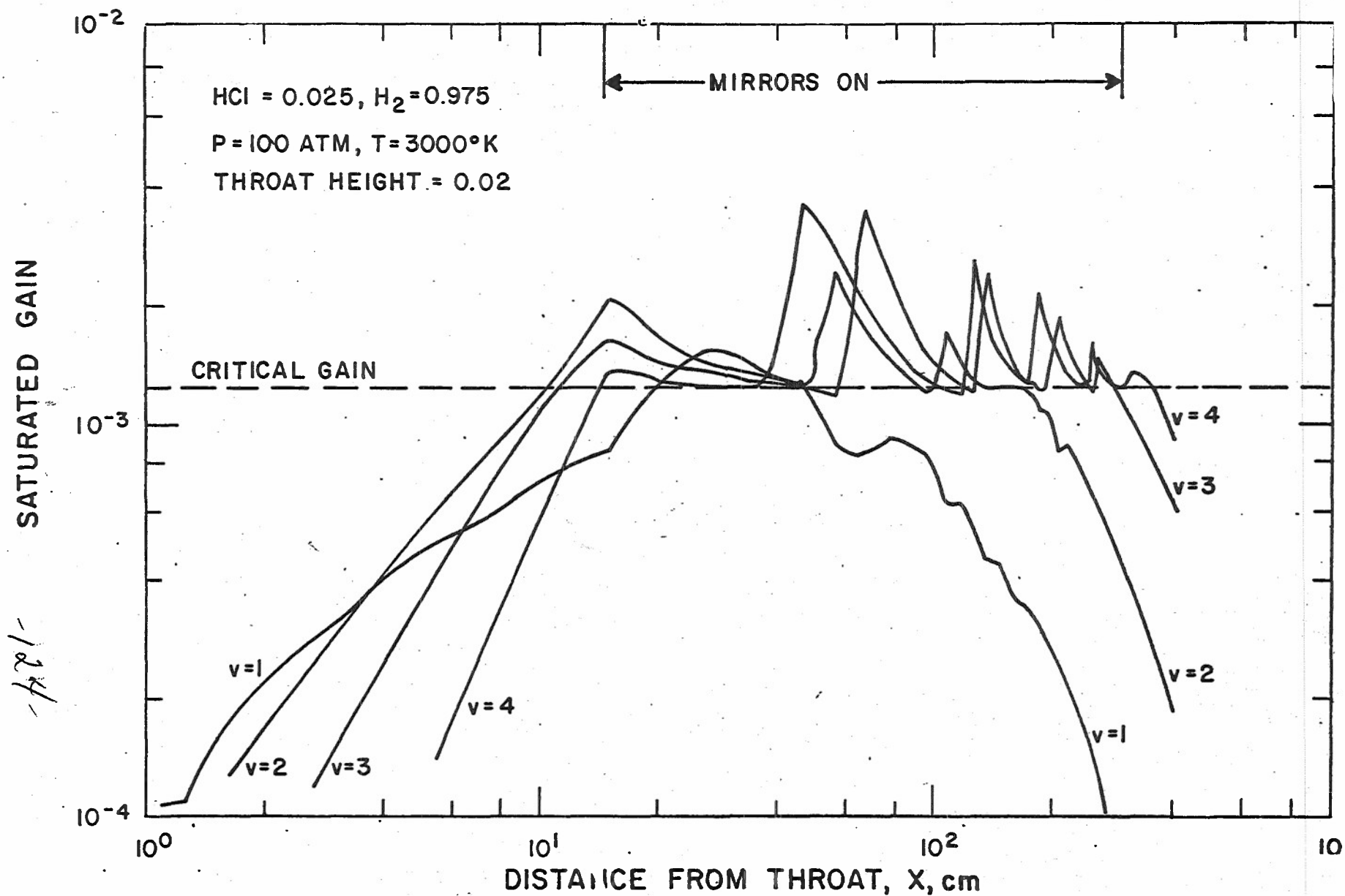
Figure 4.20. Saturated gain for v=1 to 4 vibrational levels of HCl. Cavity conditions: \lambda=100 \text{ cm} , R=0.98 , and L=0.2 .
