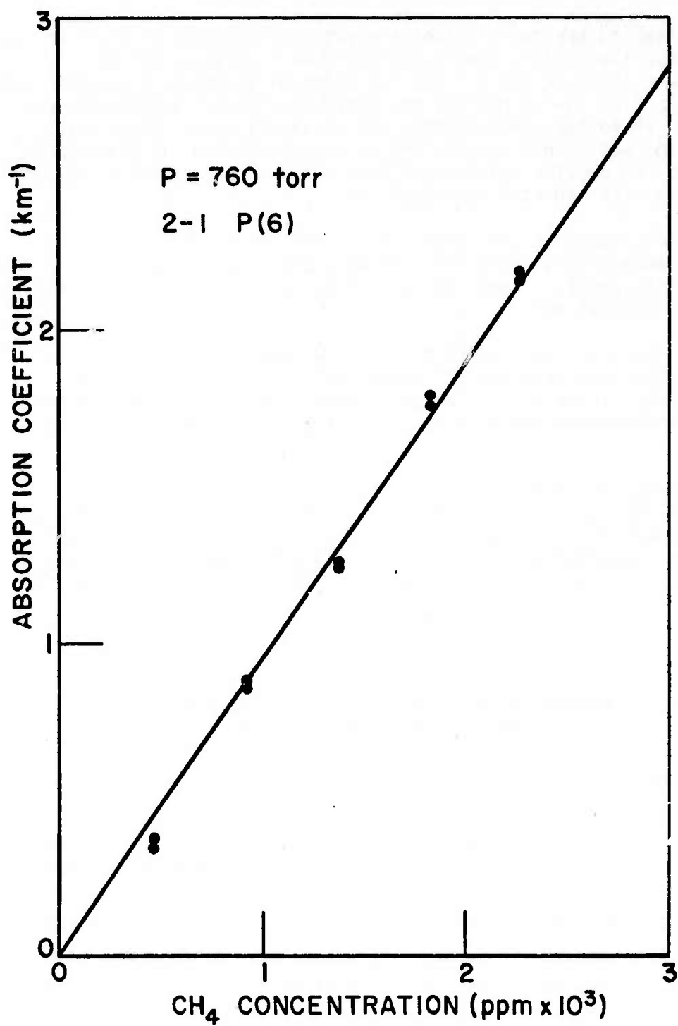
Fig. 65. Measured \text{CH}_4 - Air absorption coefficient for 2-1 P(6) line at 2680.179 cm -1 .
