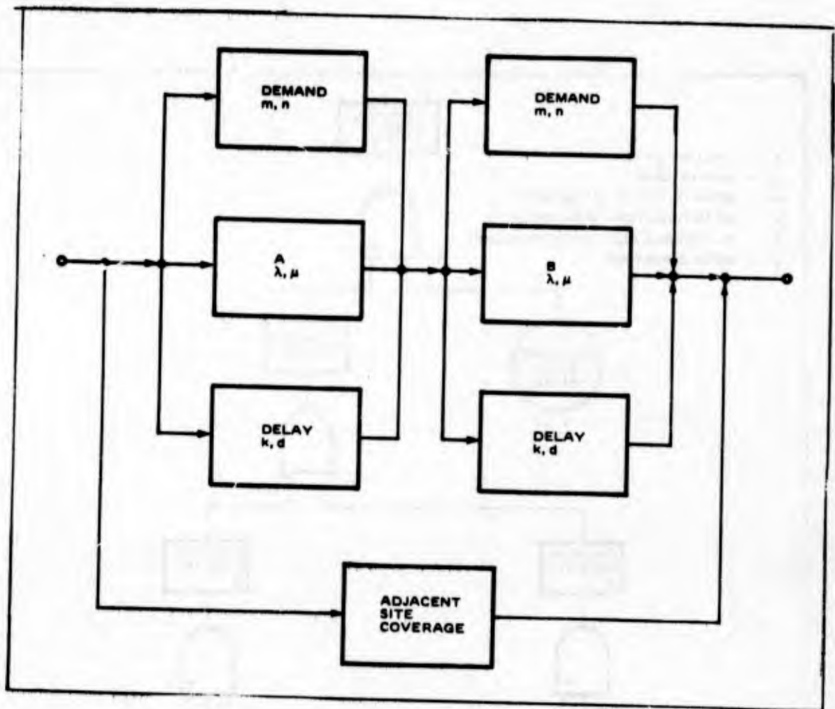
Figure 3.3.7 Multi-Function CBD with Adjacent Site Coverage
