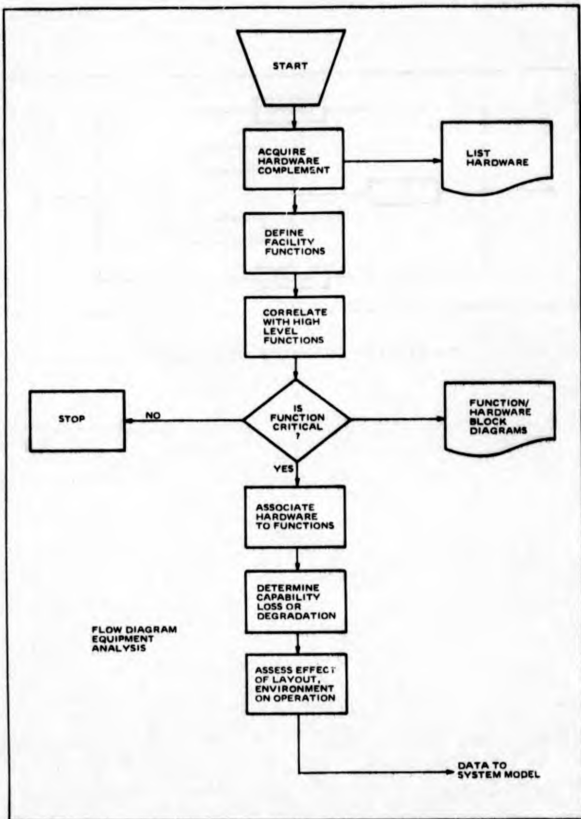
Figure 3.4.2 Flow Diagram Equipment Analysis
