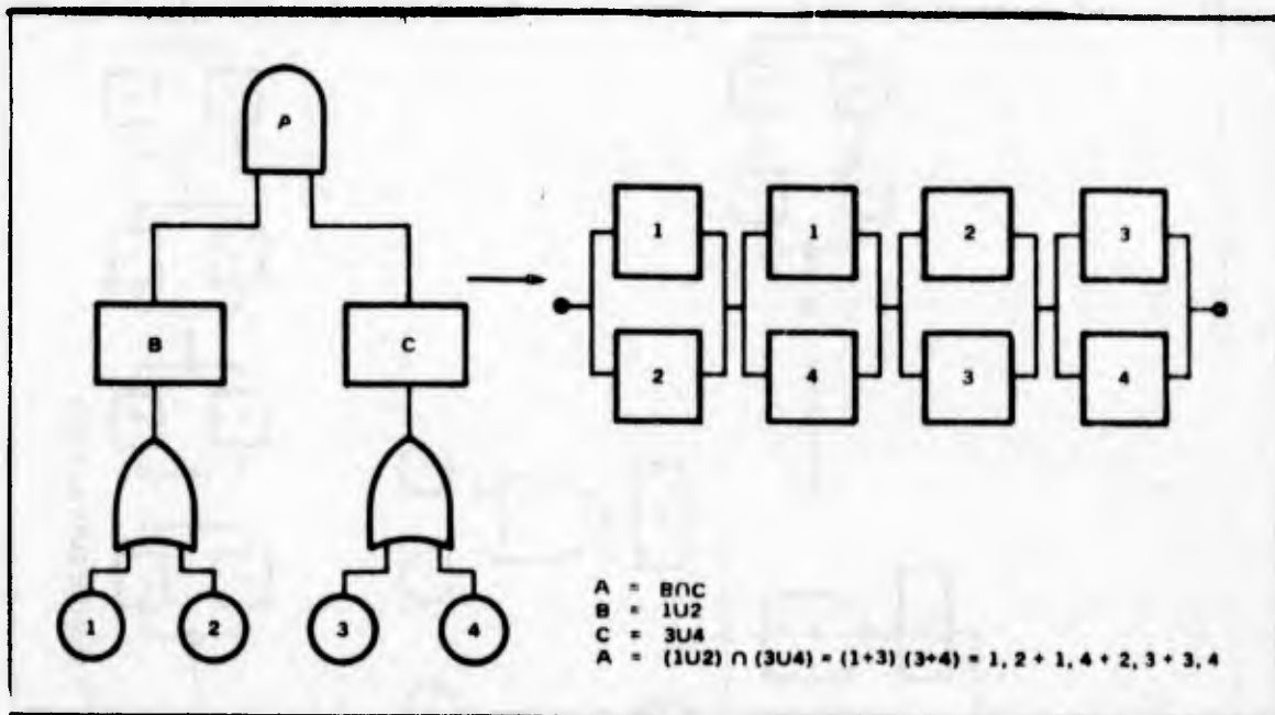
Figure 3.3.11 Boolean Determination of Cut Sets
