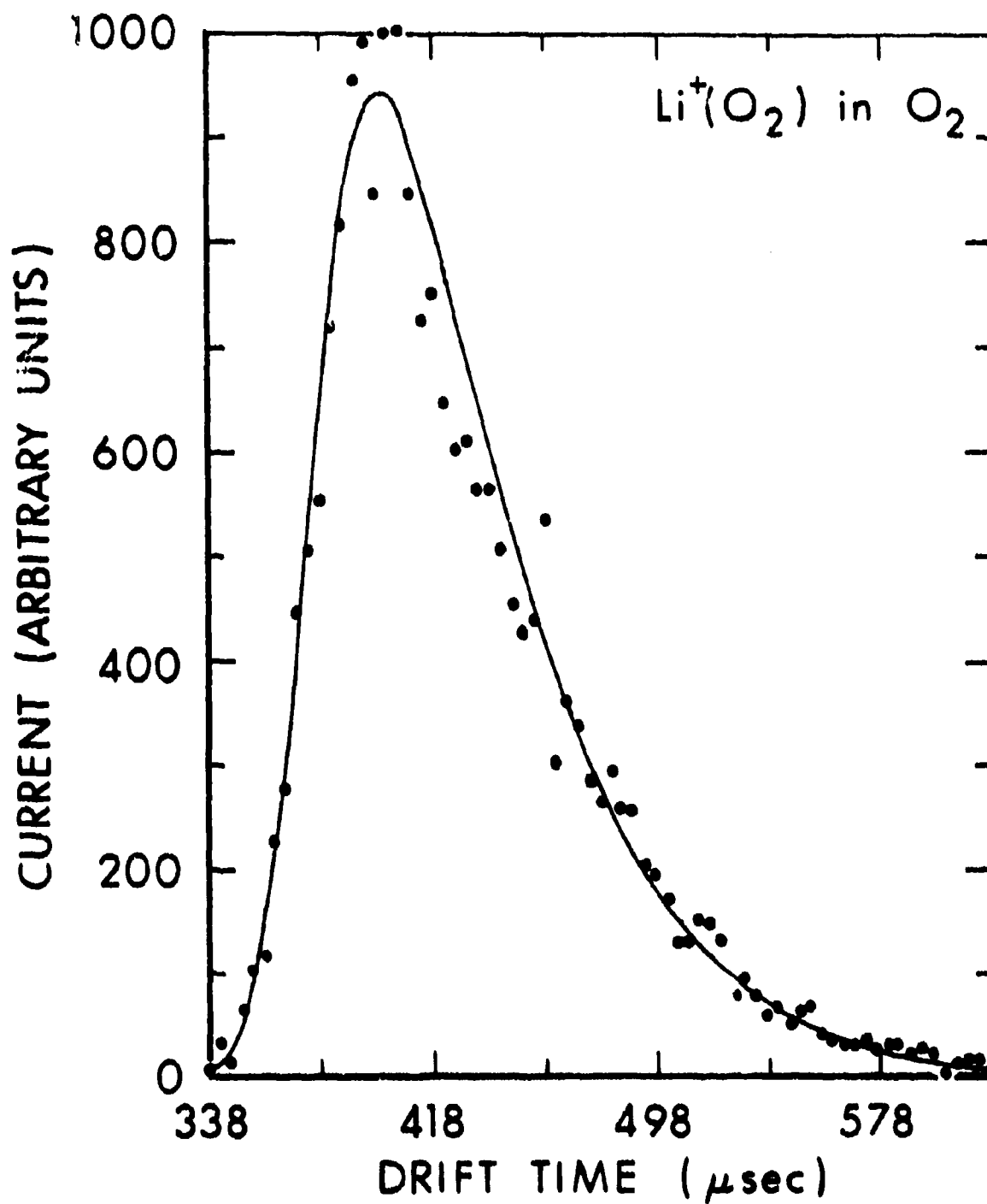
Figure 2. Comparison of experimental data with model calculations for Li + (O 2 ) under the same conditions as in Figure 1. The dots are measurements and the smooth curves are model calculations.
