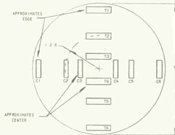
Fig. 4b. - Layout of fracture toughness specimens within a disk.
