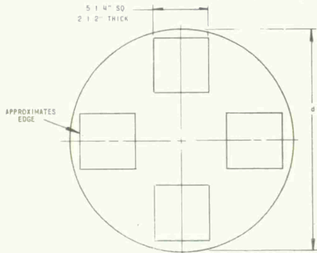
Fig. 4a. - Tensile and Charpy specimen layout within a disk.
