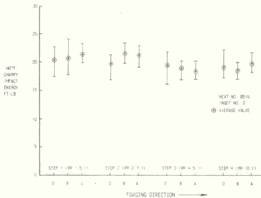
Fig. 10 - Variation of Charpy Impact energy with forging reduction in Ingot No. 2.
