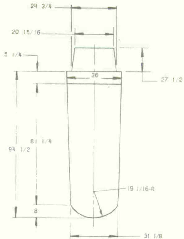
Fig. 1 - Schematic showing ingot dimensions.
