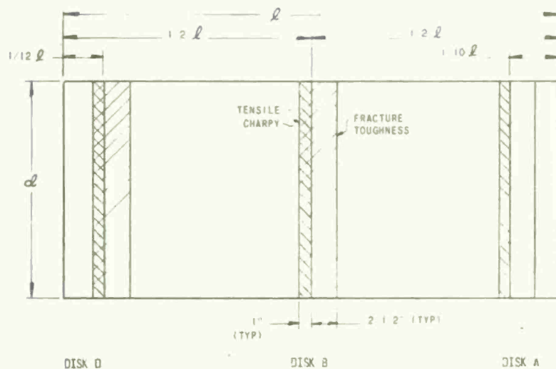
Fig. 3 - General sampling layout of disks within a step.
