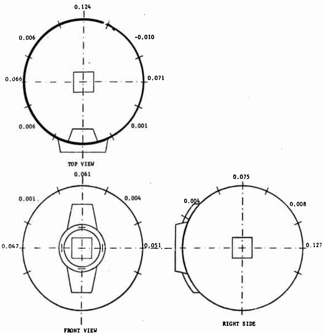
FIGURE 7. INCREMENTAL CHANGES IN THE FIDUCIAL MARK READINGS IN INCHES ON THE FIRST FIVE-FOOT EXPLOSION CONTAINMENT VESSEL DUE TO SHOT 4.
