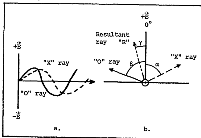
Figure 14. The Difference in Angular Rotation Between the Ordinary ("O") and Extraordinary ("X") Components of an Electromagnetic Wave Crossing a Magnetic Field. The direction of propagation is to the right in Figure 14a, and toward the observer in Figure 14b.
