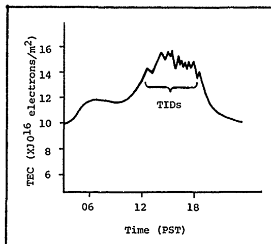
Figure 22. Fluctuations in TEC Due to Travelling Ionospheric Disturbances (TIDs). These measurements were made at Ely, Nevada by the Stanford Research Institute, while monitoring the ATS-1 satellite on 5 June 1967.
