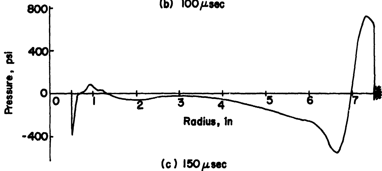
FIG. 24 ENTRY WALL NET PRESSURE 2p_0 (DRAG) \div p_0 (SHOCK) -\rho c \dot{w} AT 50, 100 AND 150 \mu sec
