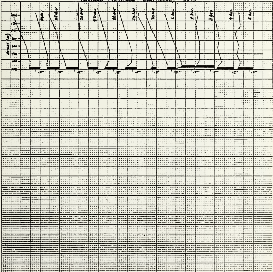
OAKLAND RADIOSONDE - 0400 (LOCAL) - 1973
