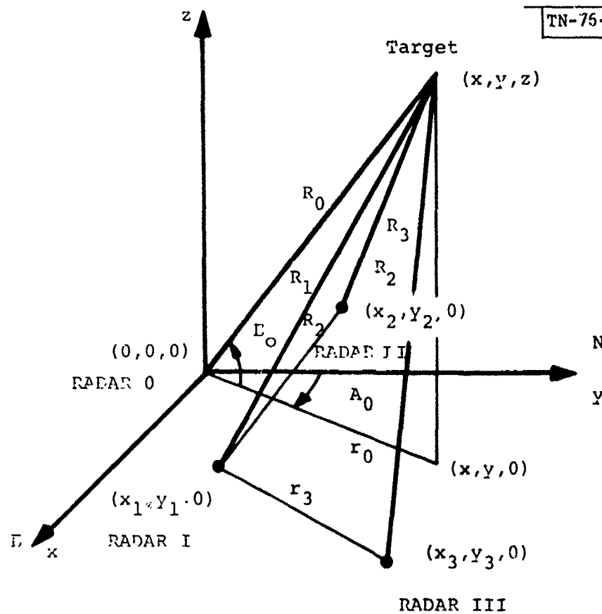
Figure A.3 Measurement transformation III.
