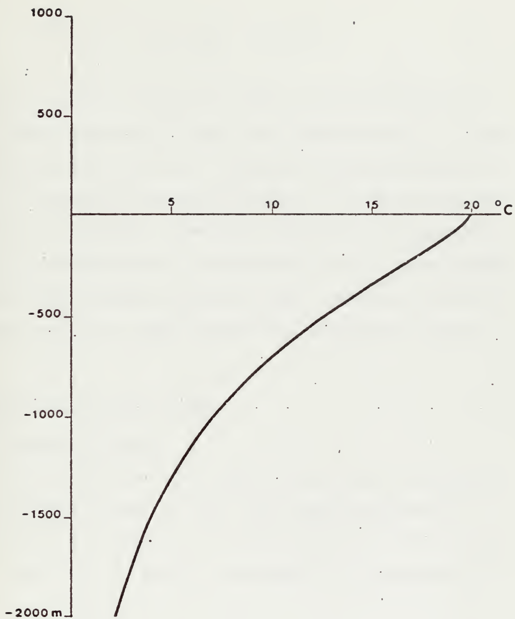
Figure 6. Initial temperature ( ^{\circ}\text{C} ) profile for numerical model.
