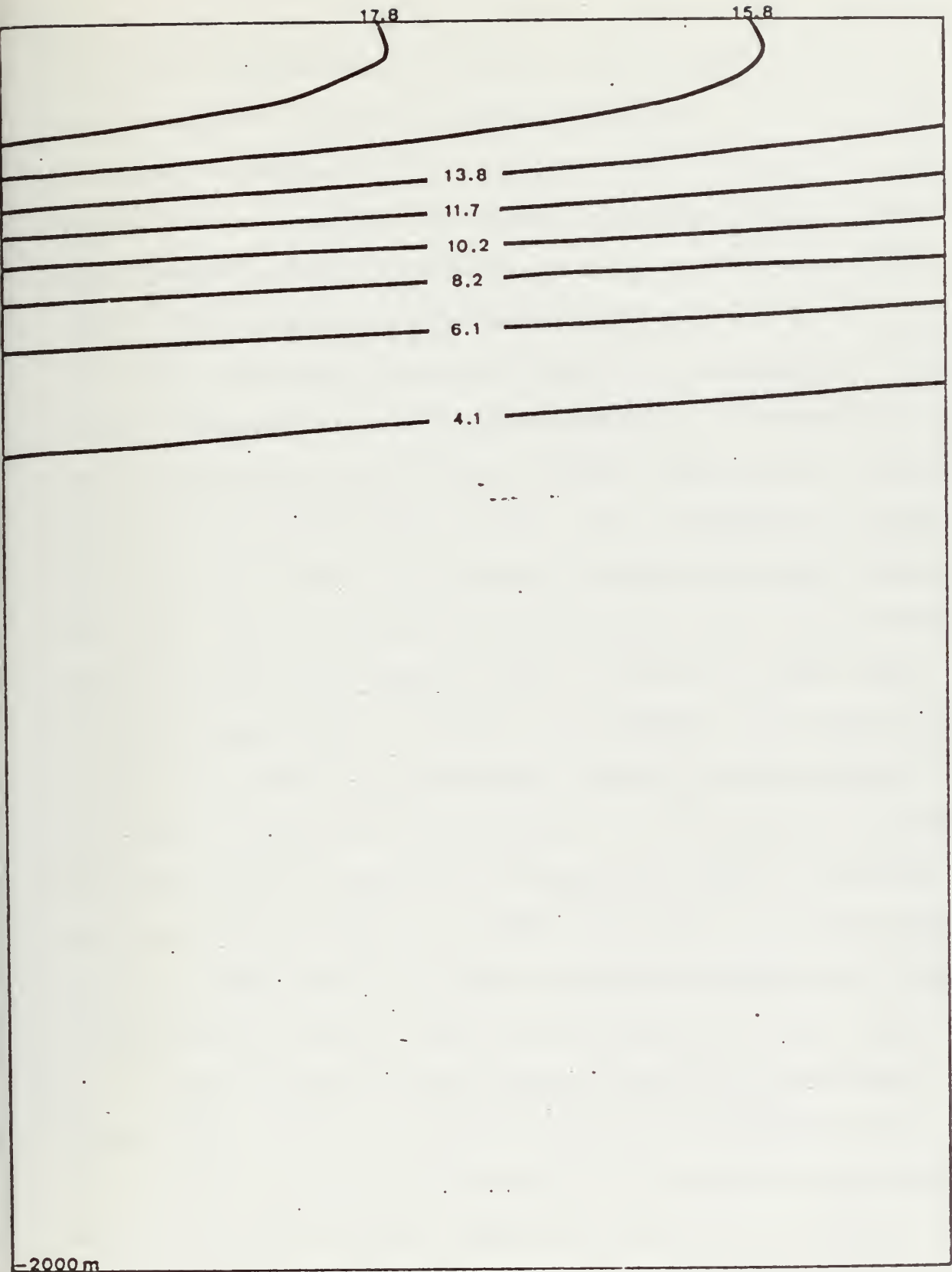
Figure 19. Numerical solution for (\partial T / \partial x)_{\circ} < 0 and w_{\circ} < 0 . Temperature is in ^{\circ}\text{C} . (\partial / \partial z) (\overline{w'T'}) = 0 .
