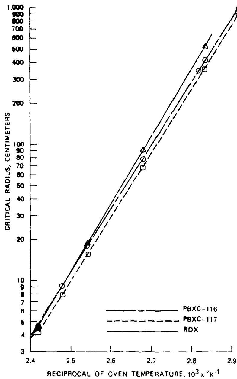
FIGURE 10. Critical Radius.
