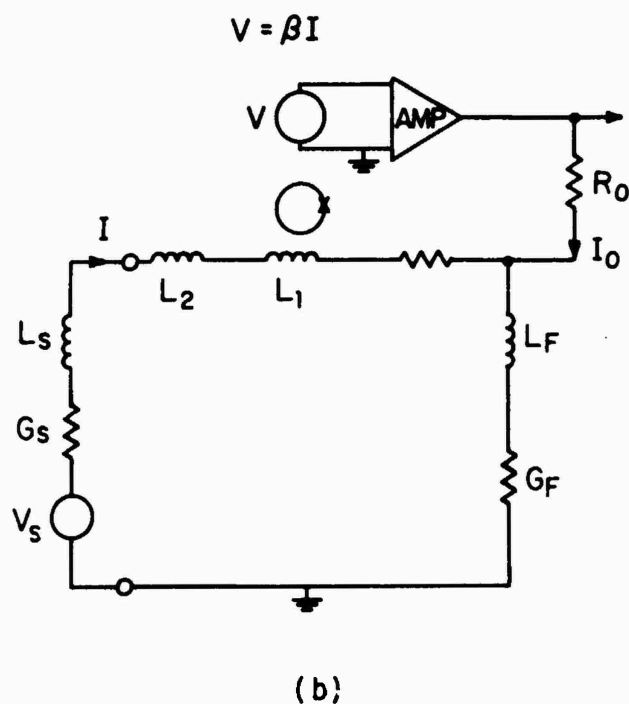
Fig. 18 a) Equivalent circuit of MOSFET current amplifier. b) Equivalent circuit of SQUID voltage amplifier.
