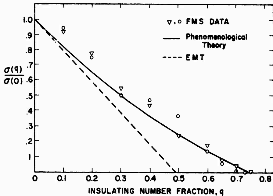
Fig. 36 Conductivity as a function of the fraction of insulating spheres in an experiment by FMS (ref. 90). To apply our theory we take the interstitial spaces as part of the insulating volume fraction. The results of the EMT are also plotted. Note that the data and both theories have been normalized not at zero volume fraction, which is unattainable in this system, but at zero number fraction.
