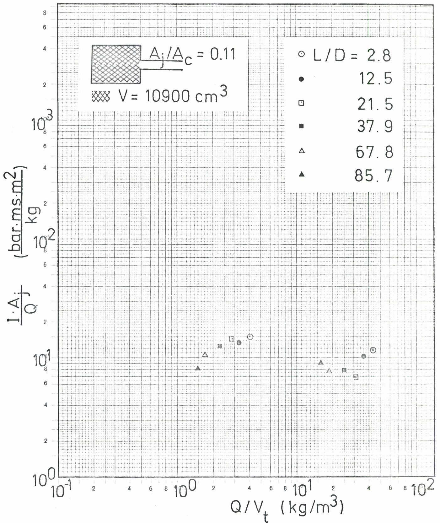
Fig. 4.3j Scaled impulse versus effective loading density [Eq.(2.1e)] at various distances in tunnel diameters from the chamber exit.
