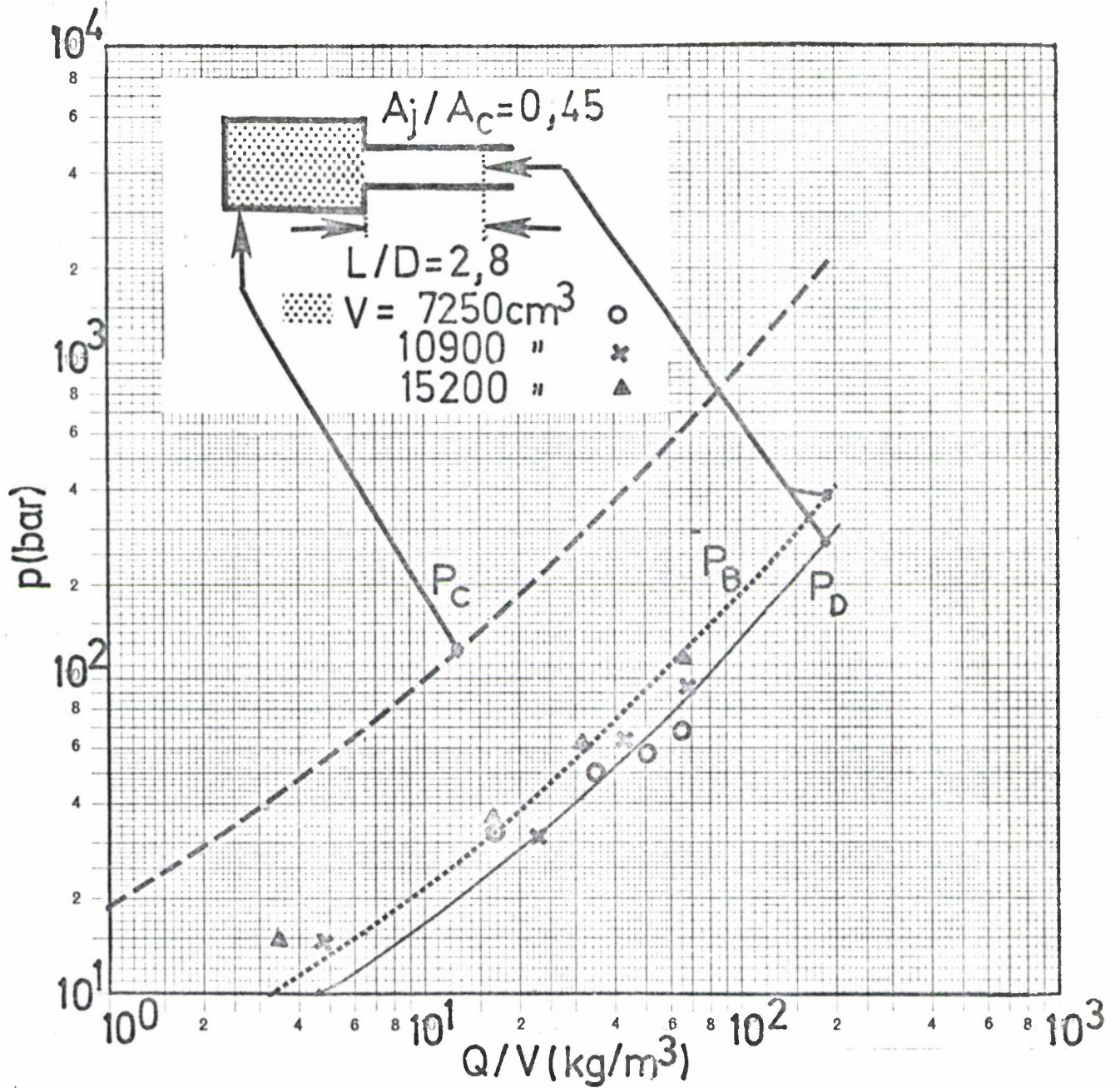
Fig. 4.1a Peak pressure near the chamber exit versus loading density for three chamber volumes. The ratio between the tunnel and chamber cross-sections is A_j/A_c = 0,45 .
