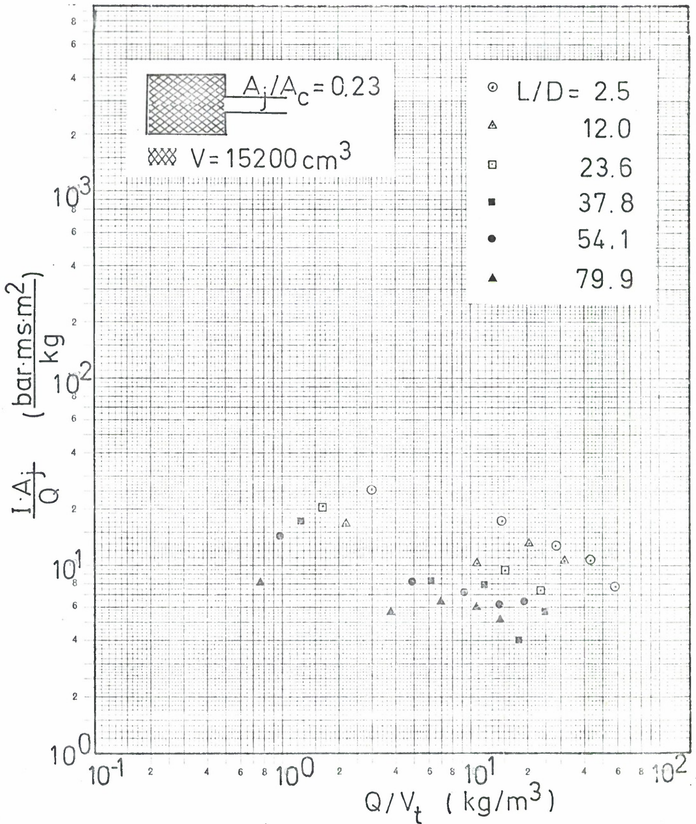
Fig. 4.3h Scaled impulse versus effective loading density [Eq.(2.1e)] at various distances in tunnel diameters from the chamber exit.
