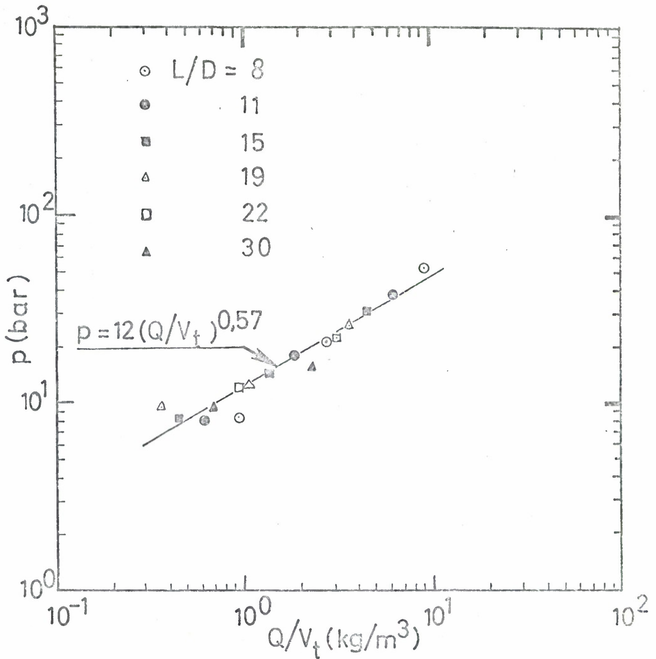
Fig. 4.5c. "Smooth wall" peak pressure p_0 versus effective loading density for the large scale test data in Fig. 4.5b.
