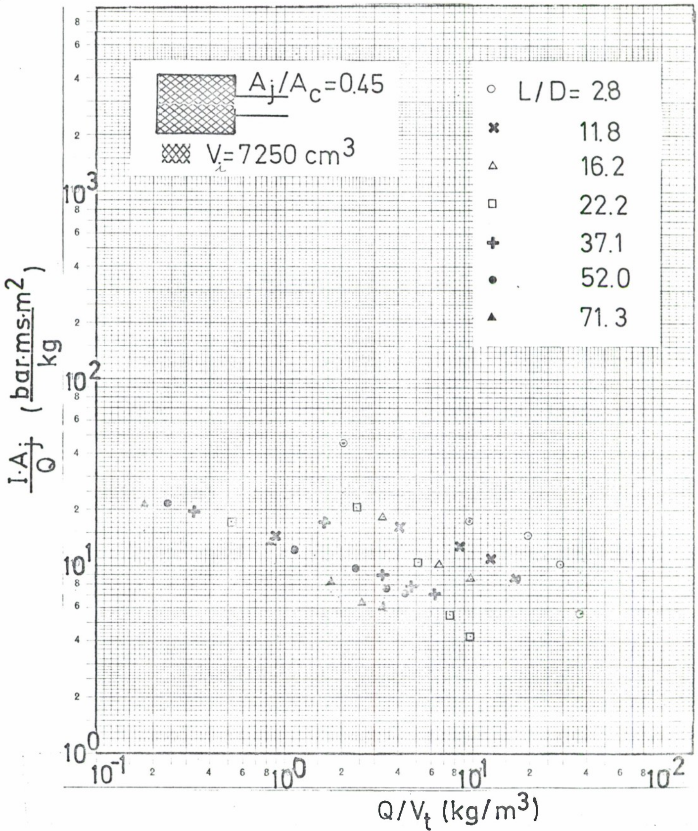
Fig. 4.3b Scaled impulse versus effective loading density [Eq.(2.1e)] at various distances in tunnel diameters from the chamber exit.
