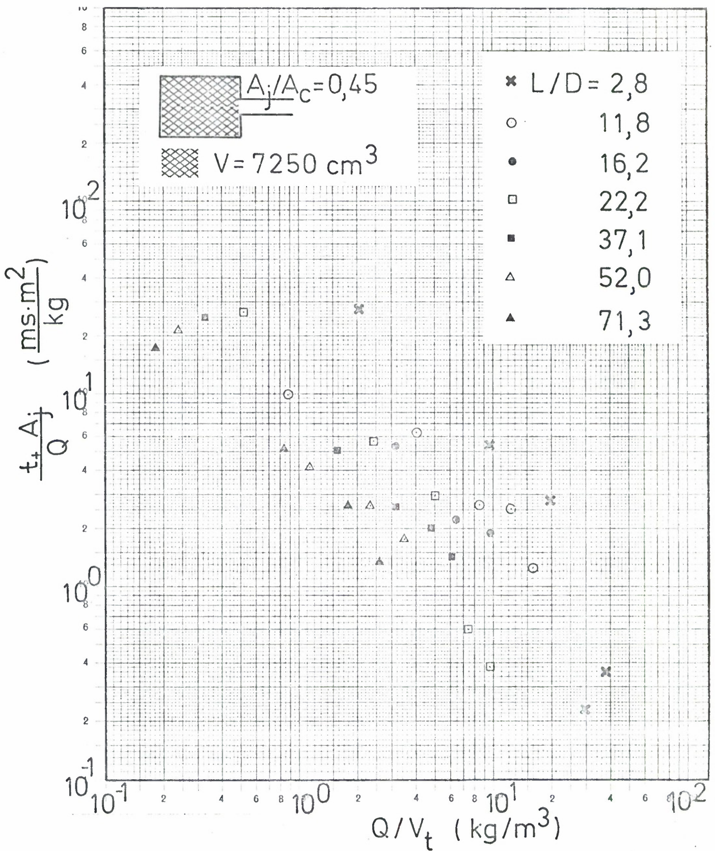
Fig. 4.3k Example of scaled positive duration versus effective loading density [(Eq.(2.1f))] at various distances in tunnel diameters from the chamber exit.
