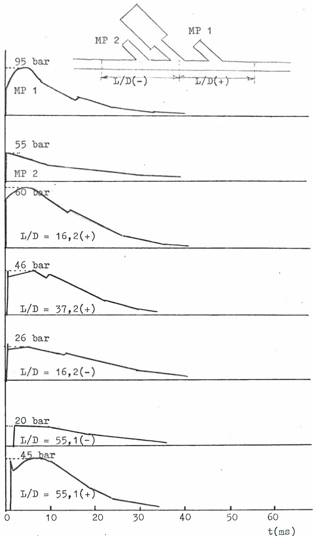
Fig. 4.4a. Averaged pressure-time recordings for Model 3 ( Q = 926 \text{ g TNT} , V_i = 18500 \text{ cm}^3 and L_i = 30 \text{ cm} ).
