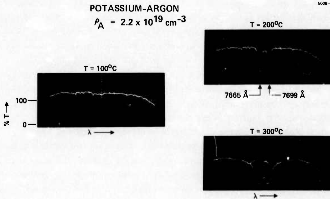
Fig. III-8. Optical transmission through potassium-argon in 15 cm sealed off cell.
