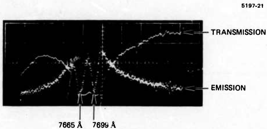
Fig. III-16. Superposition of potassium-argon excimer optical emission and transmission spectra.
