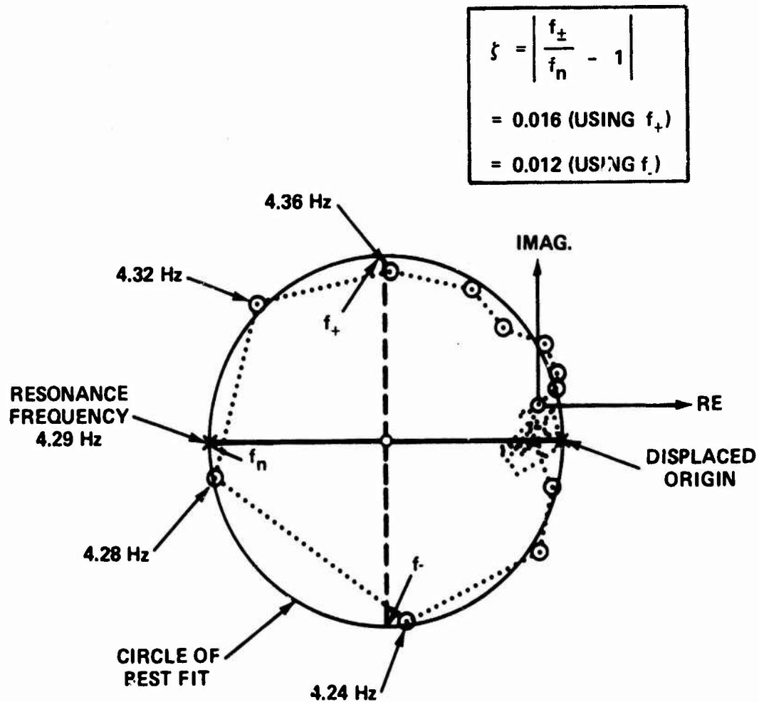
Figure 11c - Complex Plane Plot of Transfer Function of Force and Velocity
