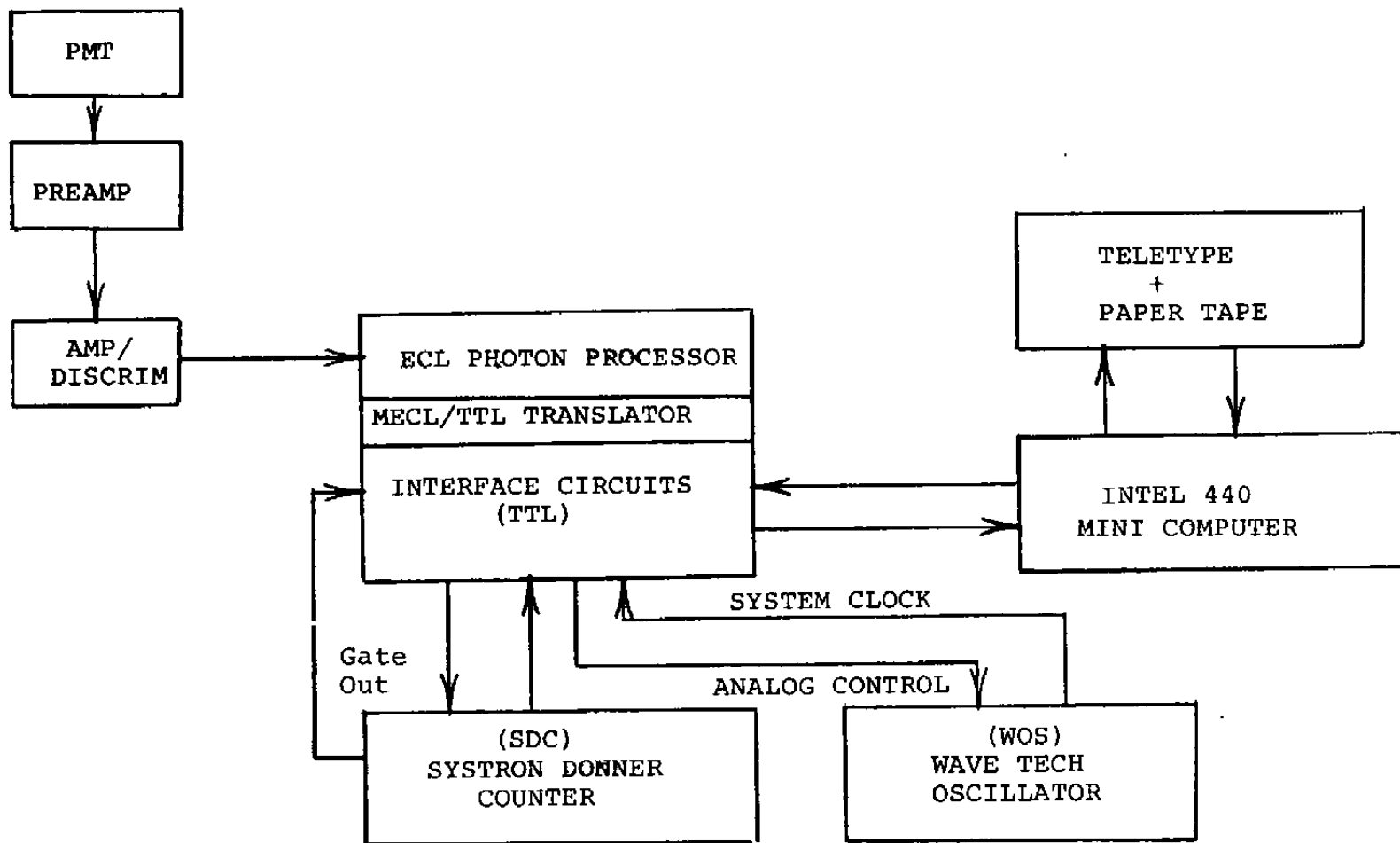
Figure 6. Proposed Extended System with Digital Counter.
