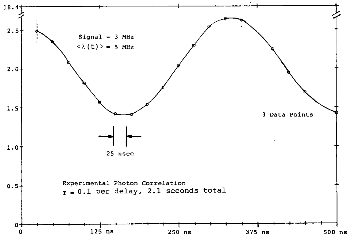
Figure 13. Experimental Photon Correlation.
