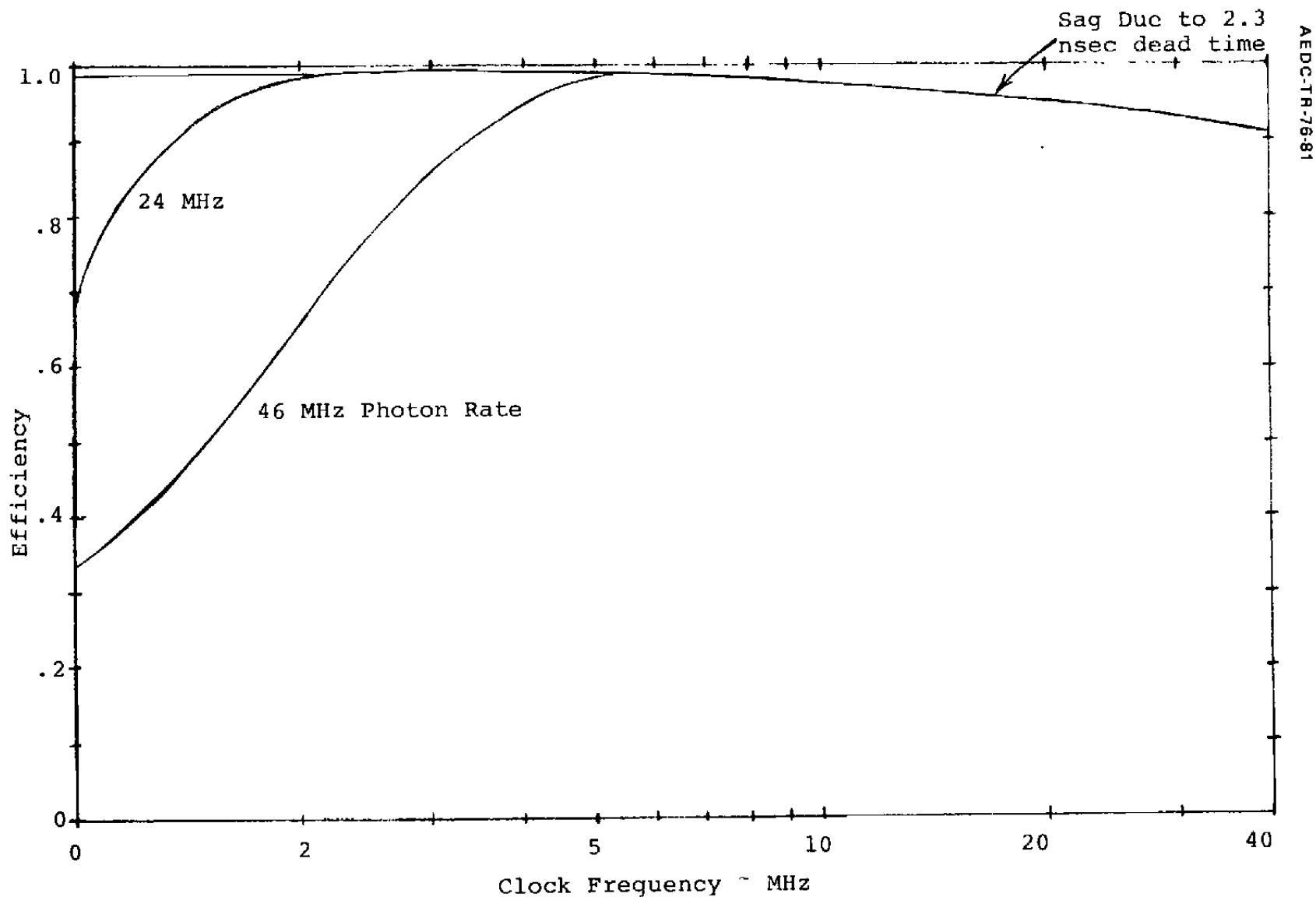
Figure 12. Efficiency of Four-Bit Counter Vs. Clock Frequency and Data Rate.
