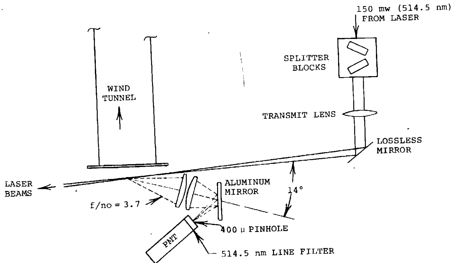
Figure 9. Optical Setup for Burst Height Distribution (Top View).
