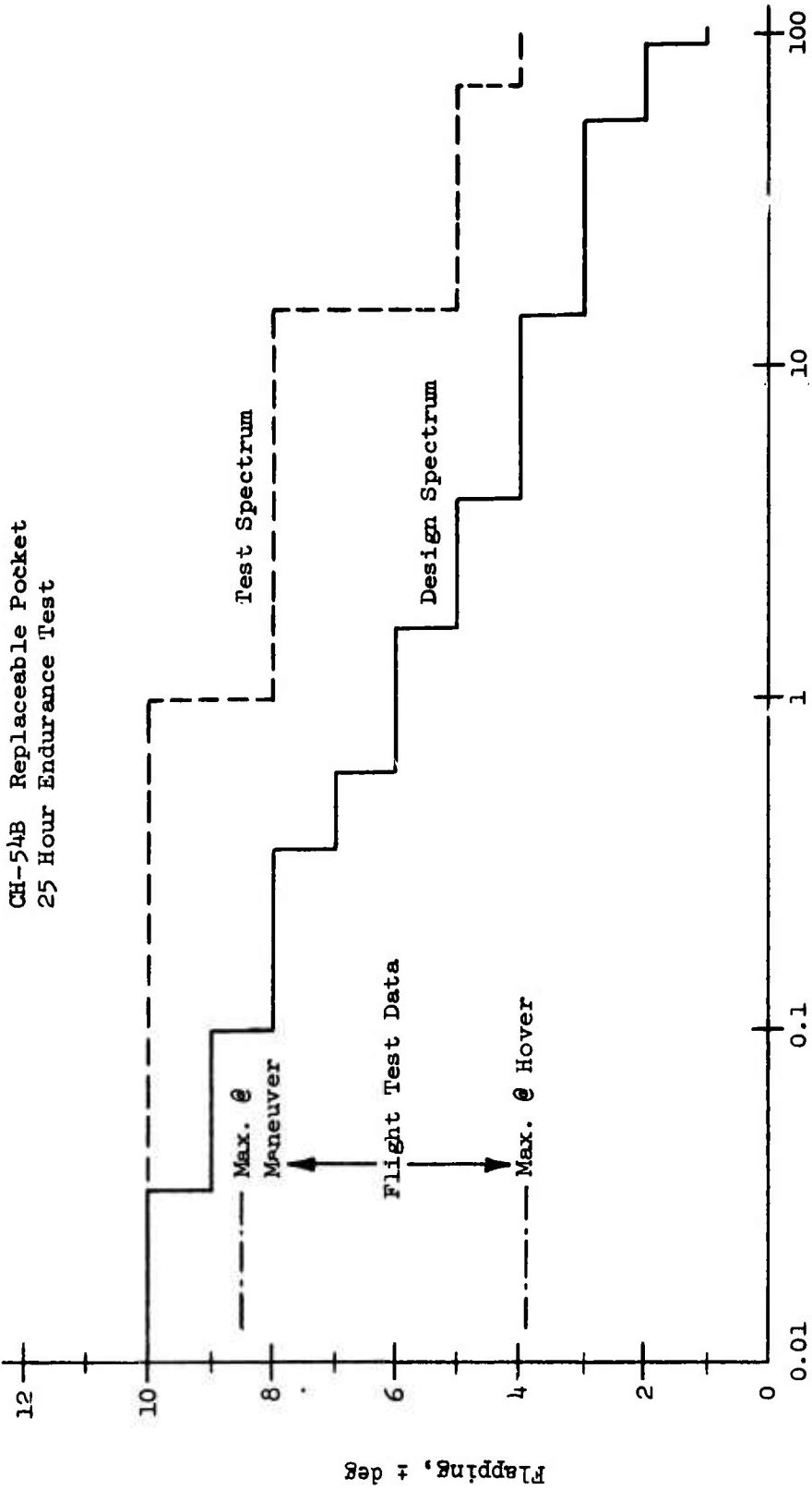
Flapping Spectrum Cumulative Percent Time
