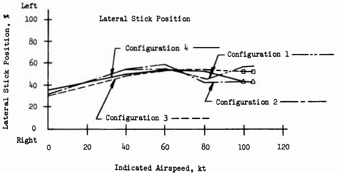
Figure 59. Lateral Stick Position vs Airspeed.
