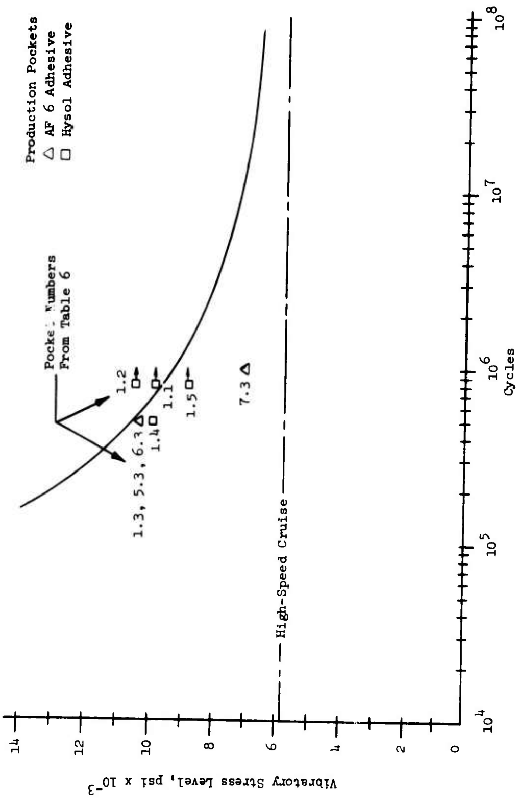
Figure 33. Damaging Cycles to Failure.
