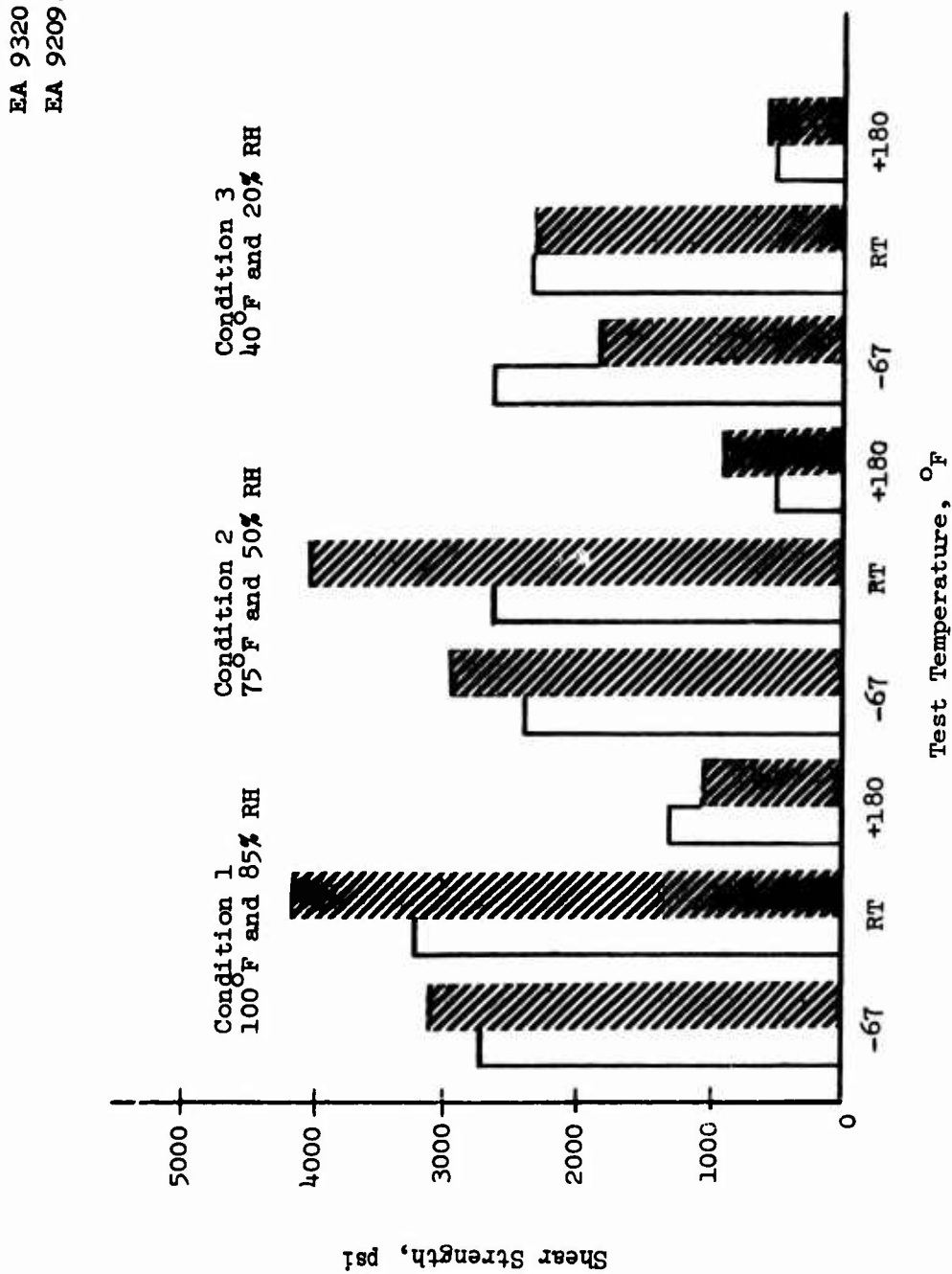
Figure 14. Comparison of EA 9320 and 9309.2 Shear Strength.
