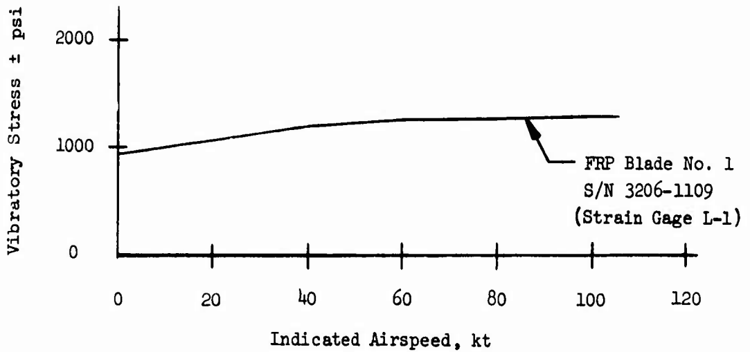
Figure 47, Configuration 1 - Blade Stresses vs Airspeed.
