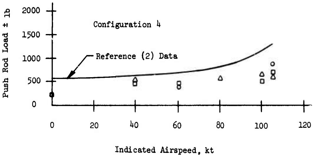
Figure 55. Configurations 3 and 4 - Push Rod Loads vs Airspeed.
