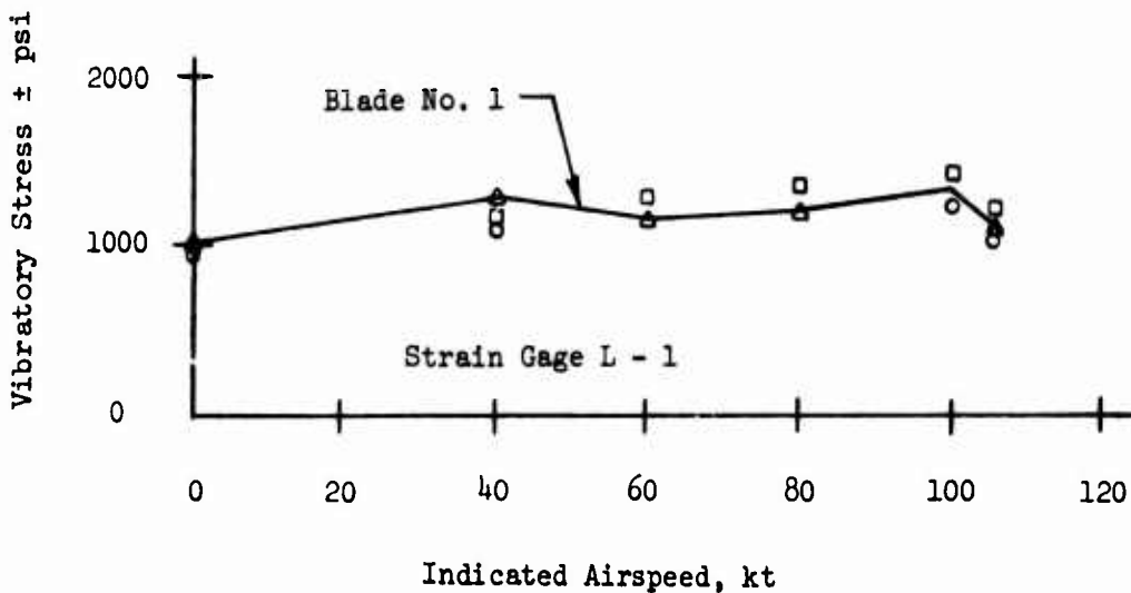
Figure 49. Configuration 2 - Blade Stresses vs Airspeed.
