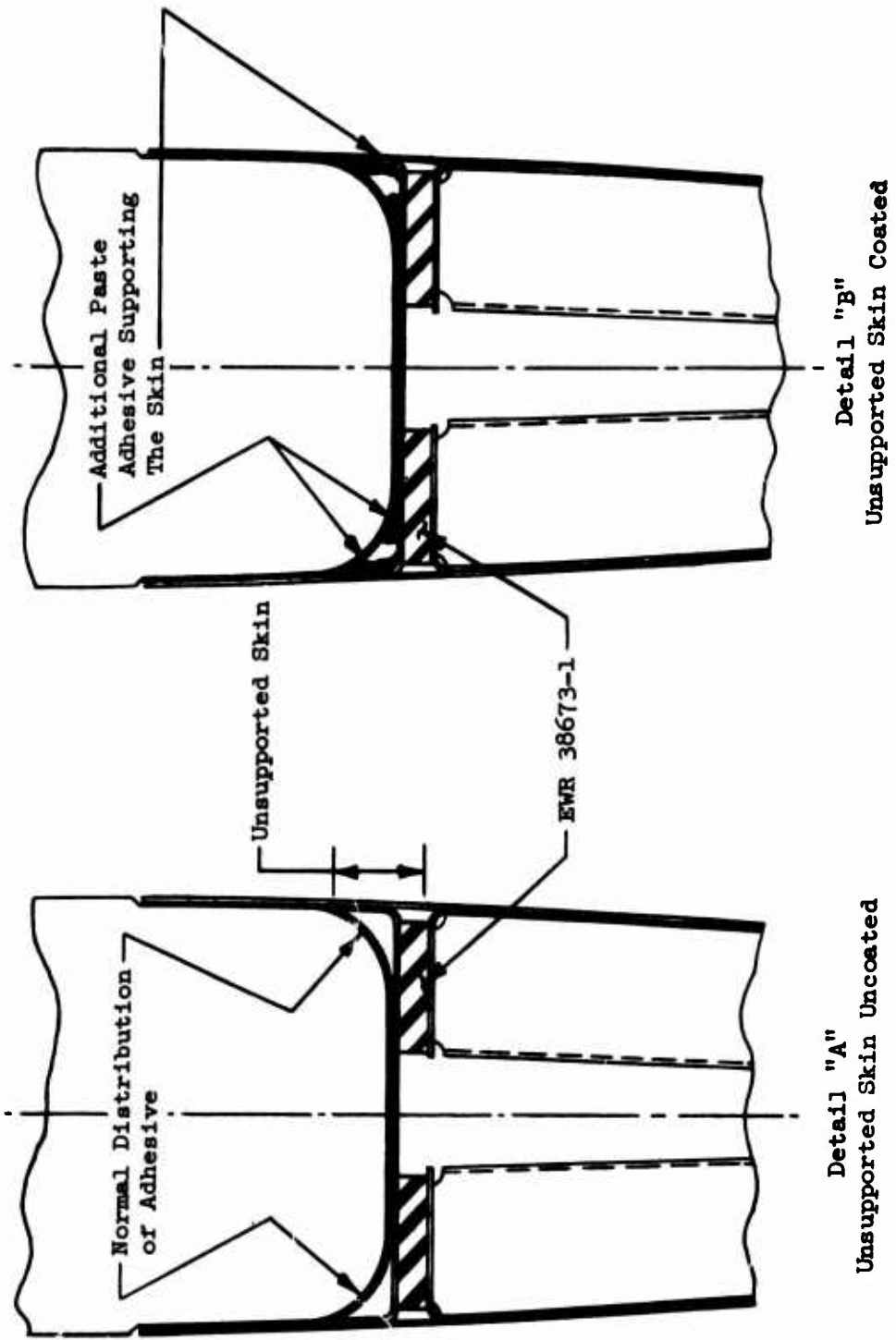
Figure A-1. Proof Load Test - Additional Paste Adhesive.
