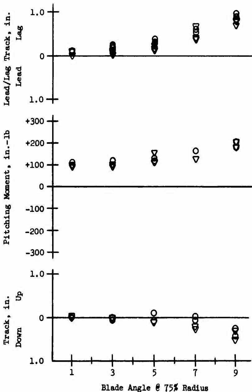
Figure 37. Blade Balance and Performance Summary.
