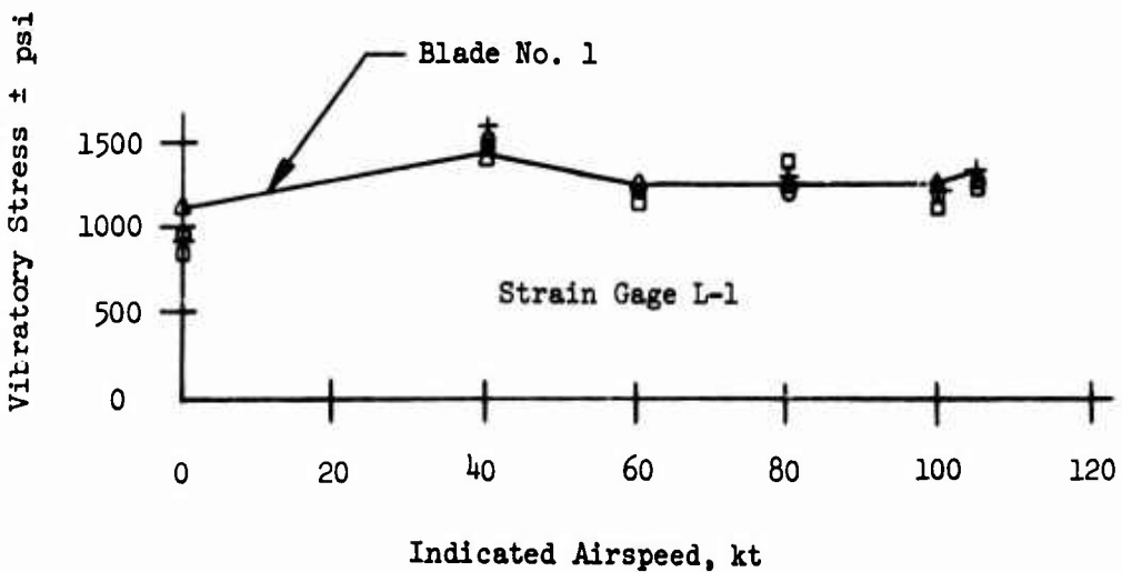
Figure 51. Configuration 3 - Blade Stresses vs Airspeed.
