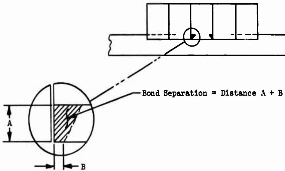
Figure C-4. Measurement of Pocket Bond Separation,
