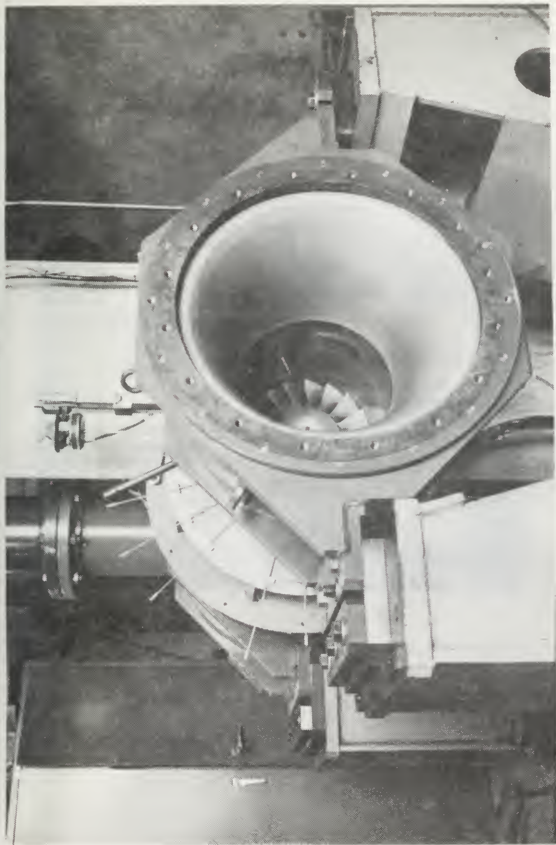
FIGURE 1(b). Test Cell
