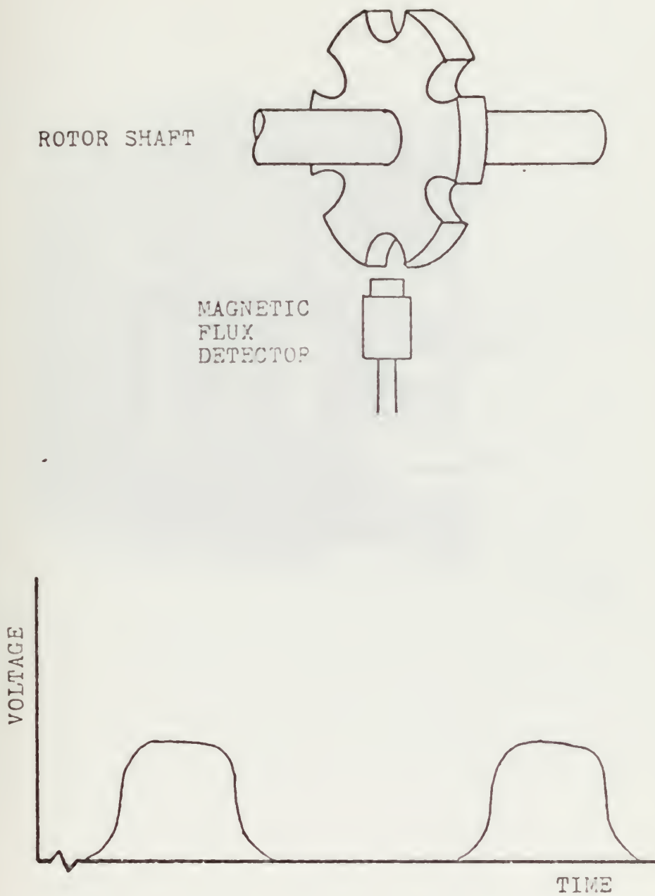
Figure A6. Magnetic Flux Cutter and Its Electrical Output
