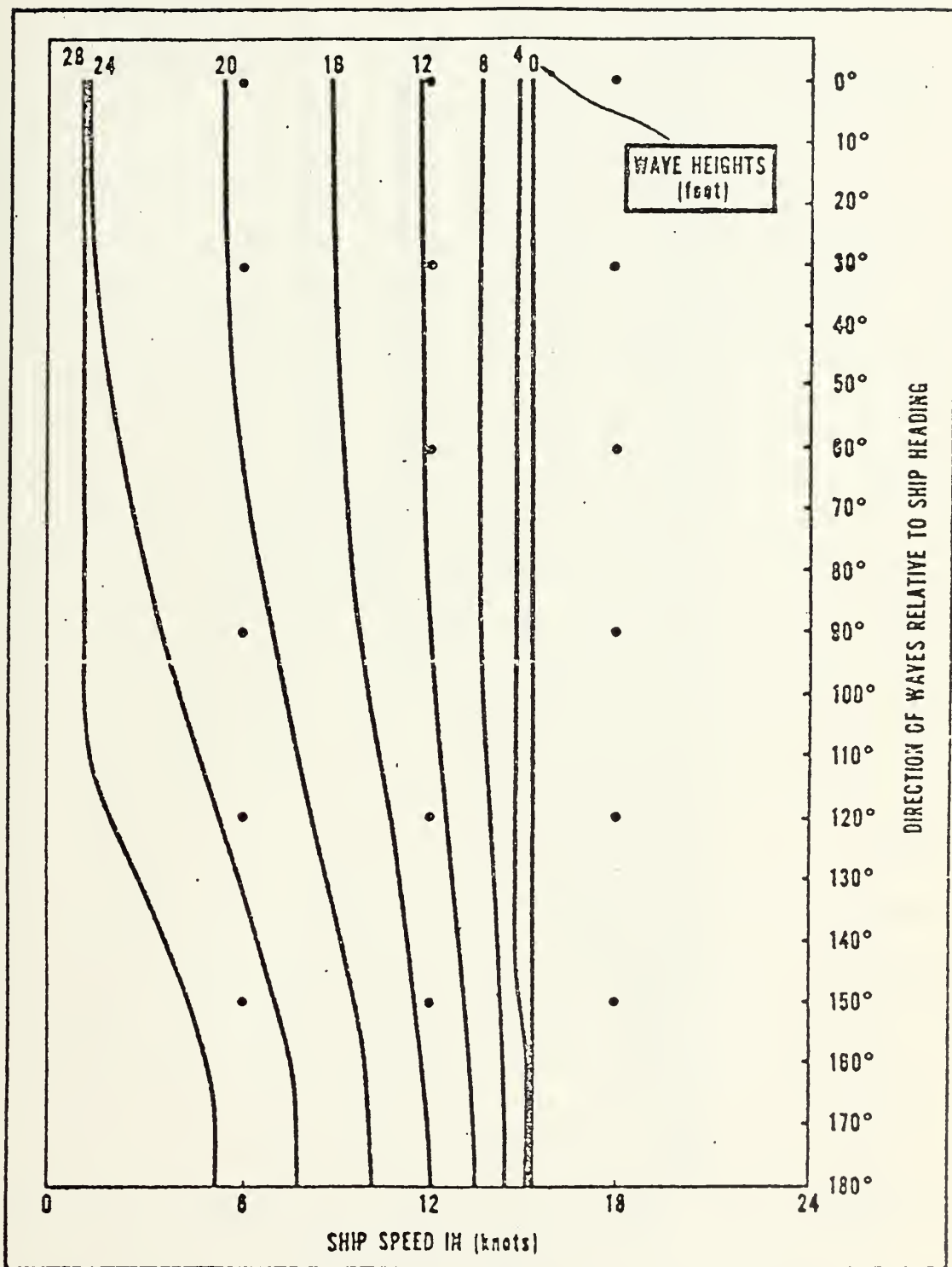
Figure C-1. Expected ship speed as a function of wave height and wave direction relative to ship's heading for a ship making 15 kt (from Nagle, 1972).
