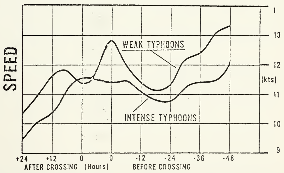
Figure 6. Average intensity (a) and speed (b) profiles for intense and weak typhoons crossing the Philippines (Brand and Bletloch, 1972).
