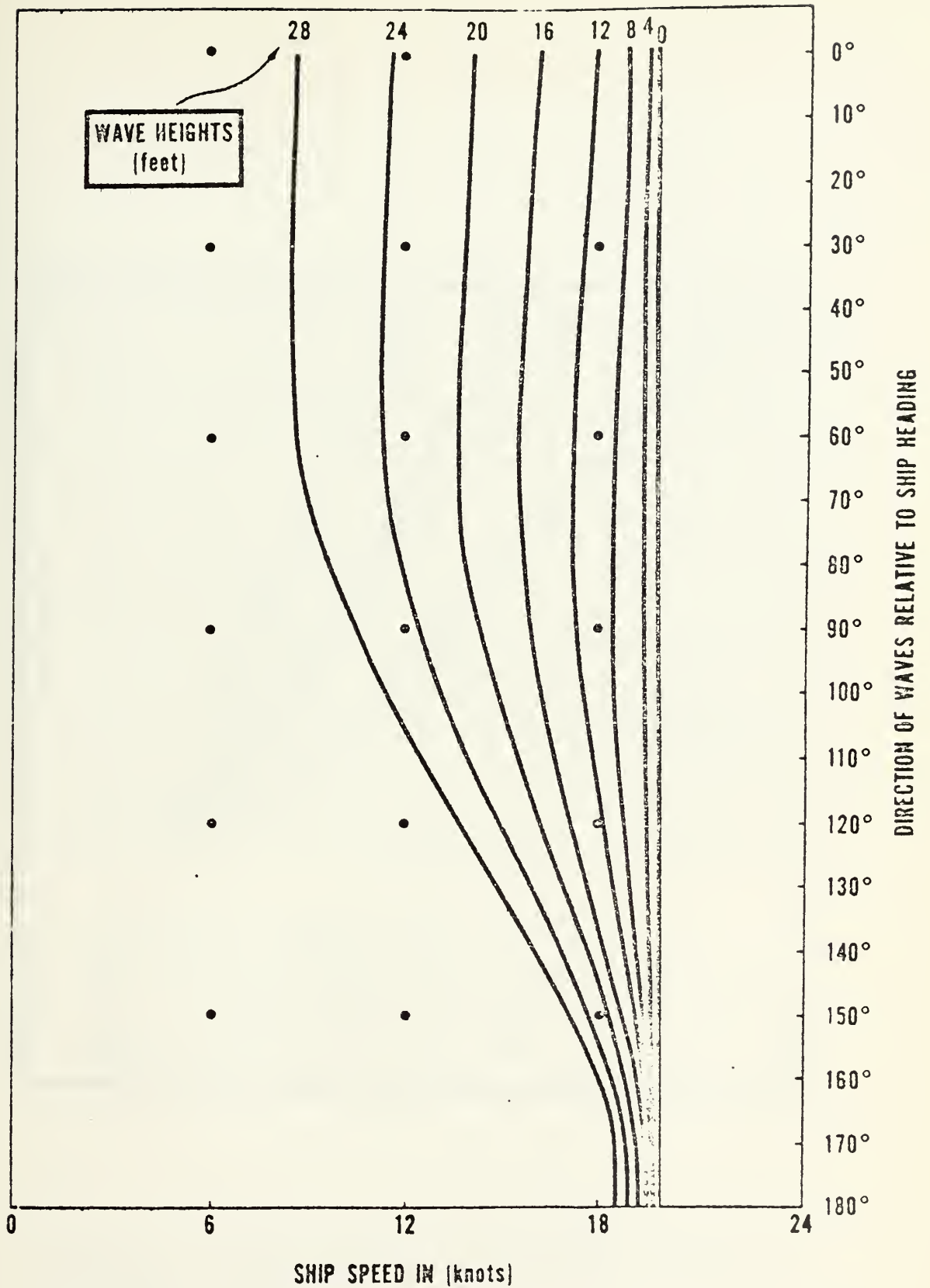
Figure C-2. Expected ship speed as a function of wave height and wave direction relative to ship's heading for a ship making 20 kt. (from Nagle, 1972).
