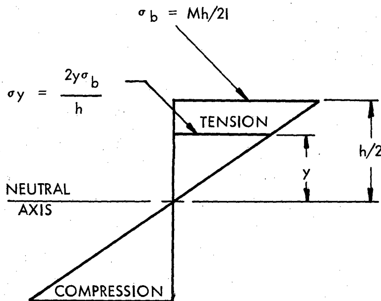
STRESS DISTRIBUTION
