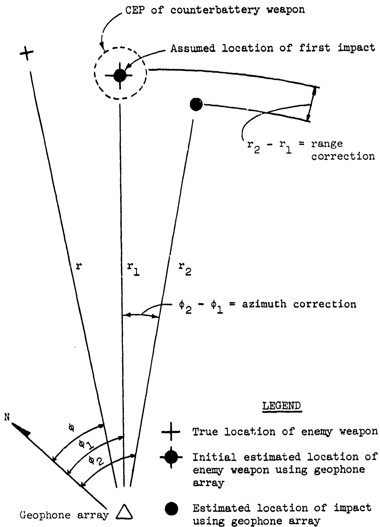
Figure B3. Calculation of position of first-round impact of counterbattery fire
