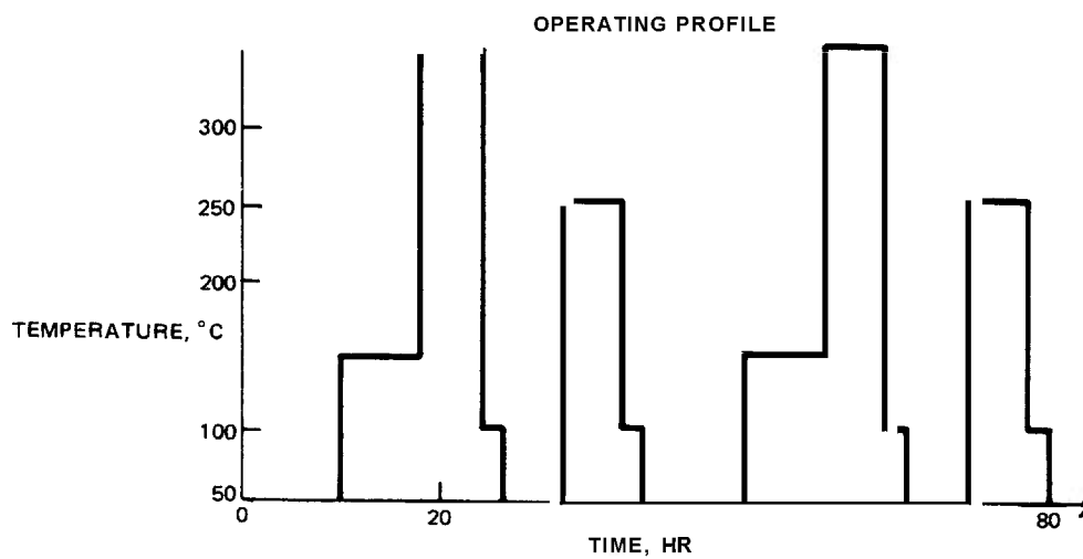
Figure 7-3. Temperature Profile
