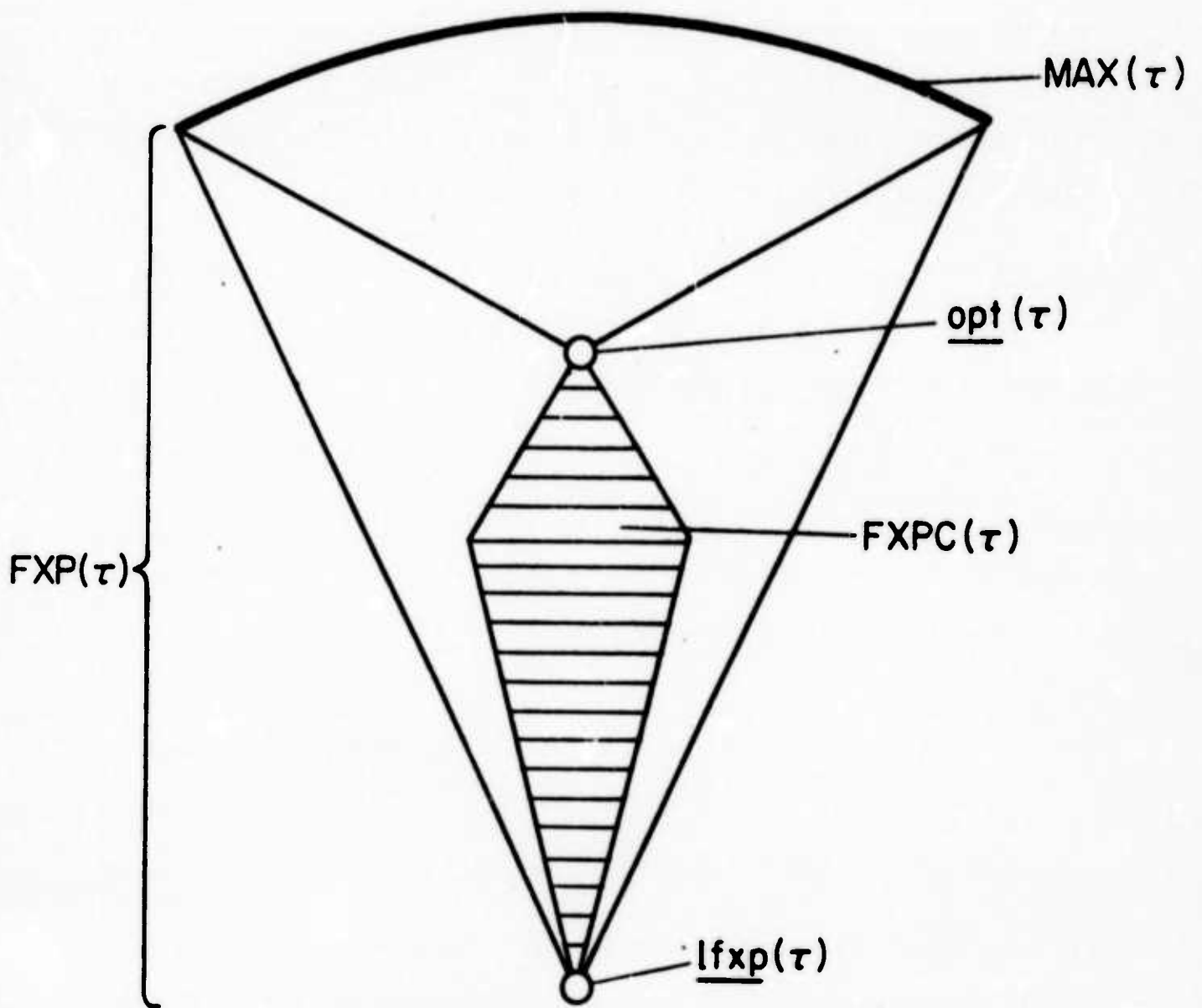
Fig. 1. The fixedpoints of a recursive program
