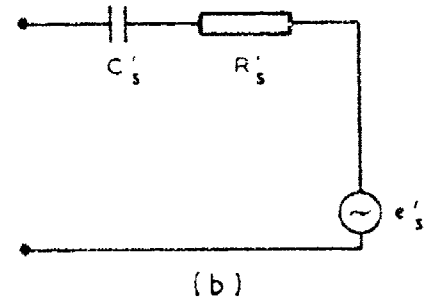
FIGS. 2(a)&amp;(b). HYDROPHONE WITH ADDED LOSS
