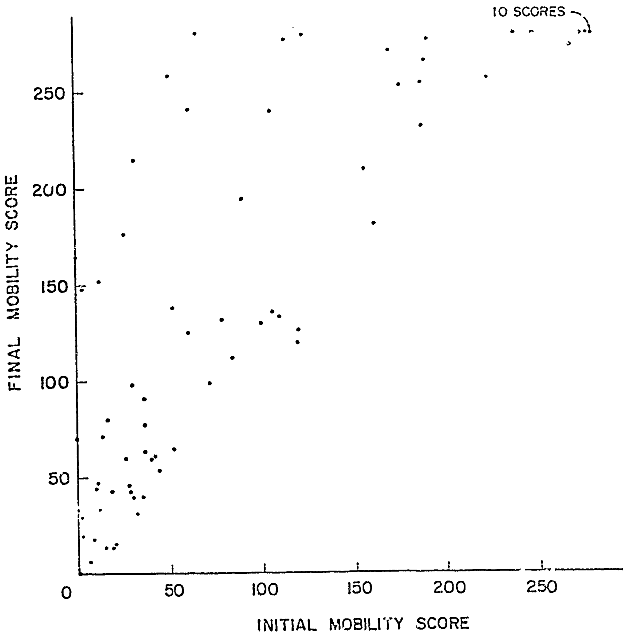
FIGURE I. SCATTER DIAGRAM OF FINAL VS. INITIAL MOBILITY SCORES FOR INJURED SPINAL CORD PATIENTS (n=75)
