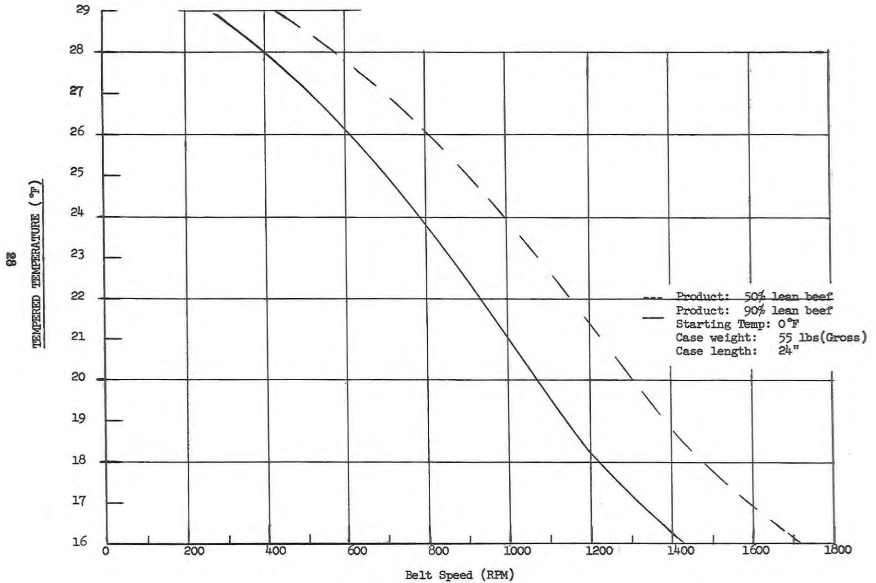
Figure B3: EFFECT OF BELT SPEED ON TEMPERED TEMPERATURE
