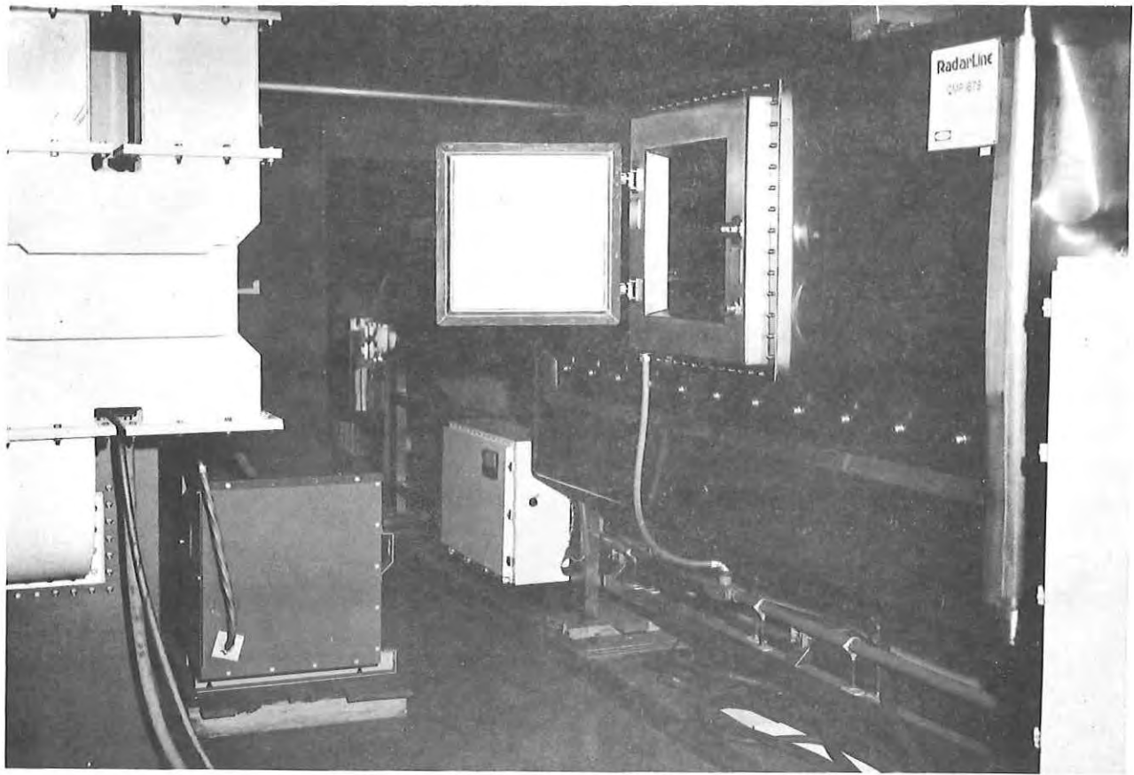
Figure A4. Side View Showing Cavity Door and Section of Waveguide
