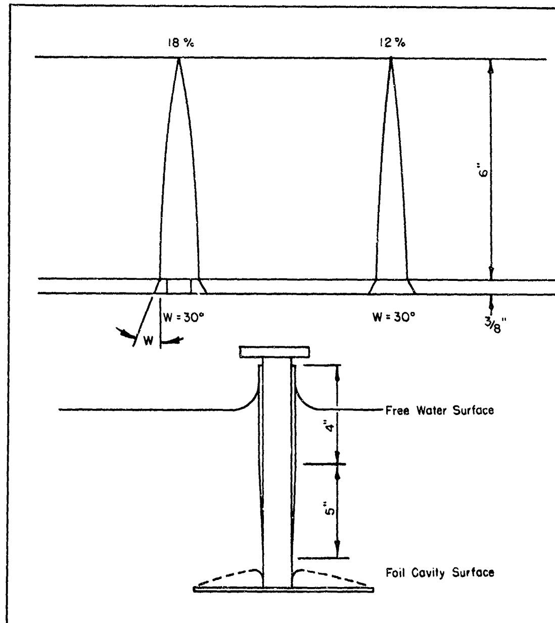
Figure 4 - Strut Spray Wedges and Boundary Layer
