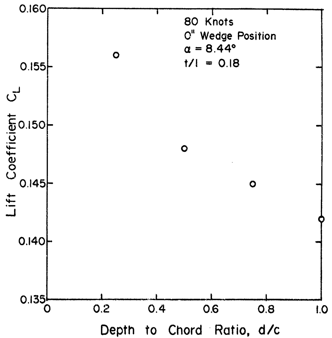
Figure 27 - Lift Coefficient versus Depth of Submergence, V = 80 Knots
