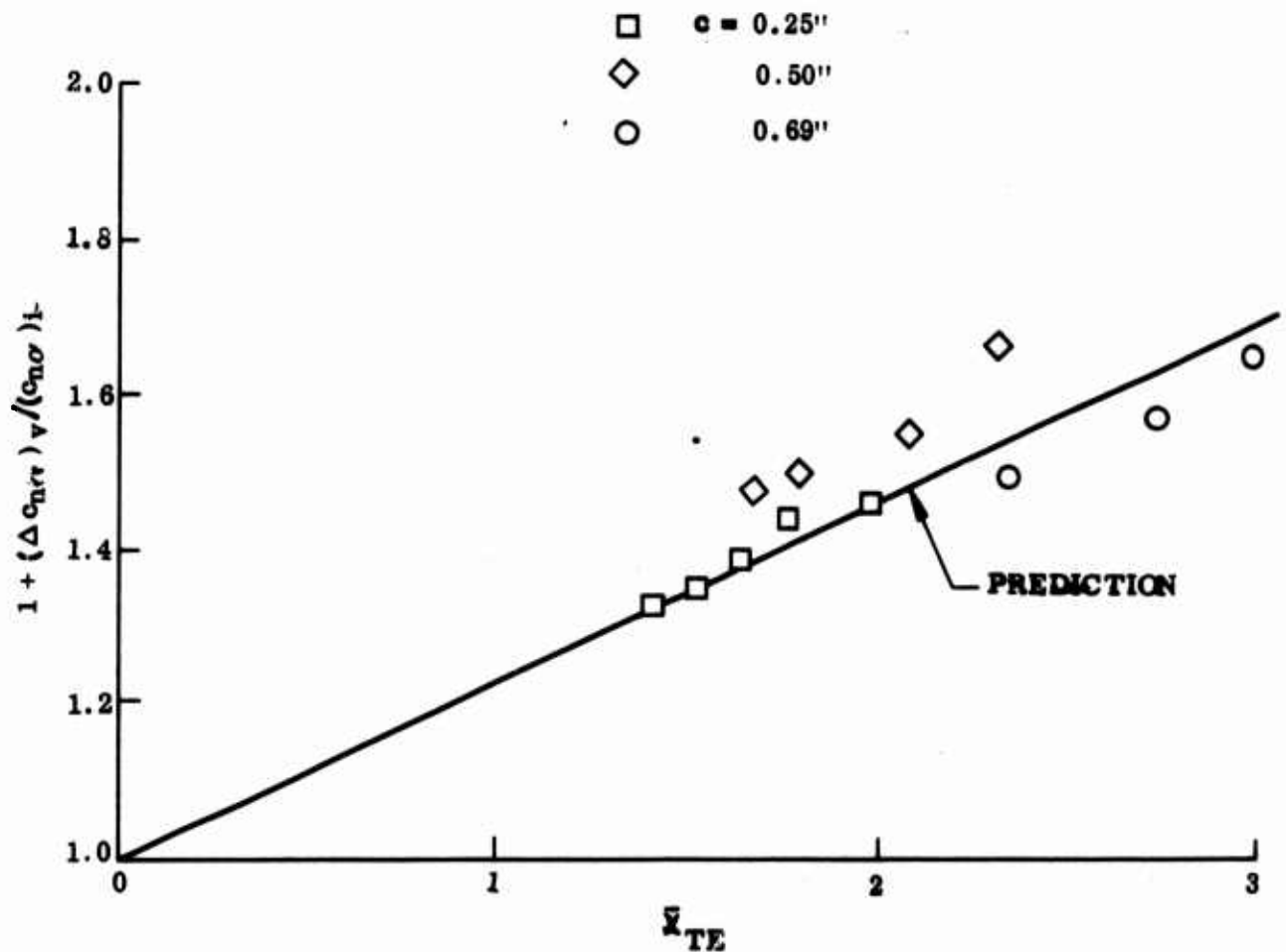
Figure 3.28 Comparison between predicted and measured viscous effects on C_{Nre} of a flat plate
