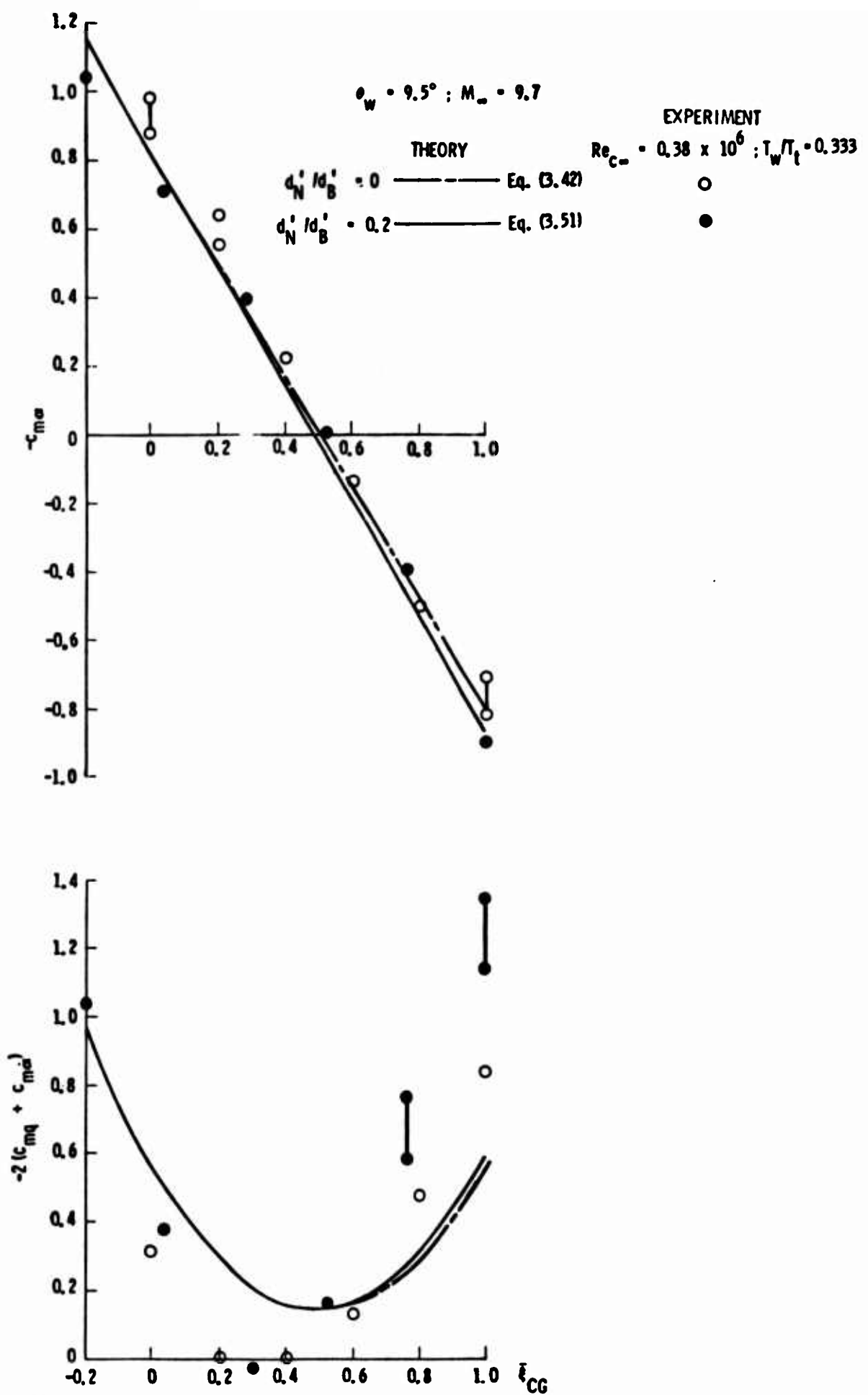
Figure 3.22 Comparison between predicted and measured viscous effects on the aerodynamic characteristics of a 9.5^\circ wedge
