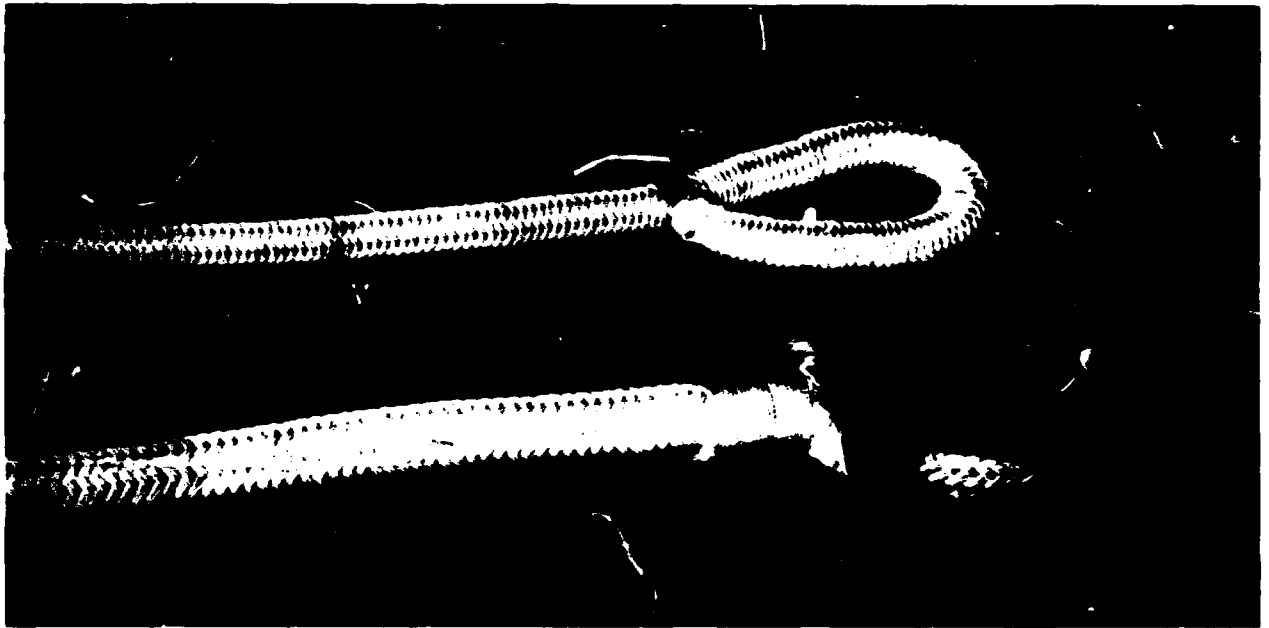
Figure 7. Modified double-braid eye splice.
